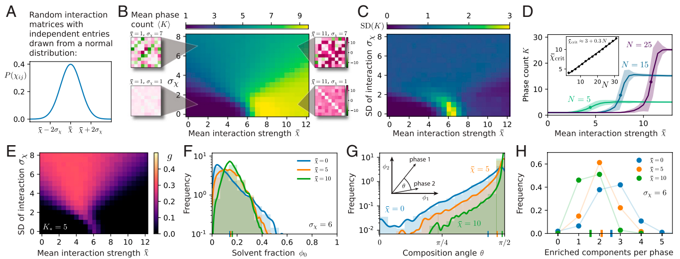
Fig. 2. Random interaction matrices cannot target specific phase counts K reliably. (A) Distribution P(\chi_{ij}) of the entries of the interaction matrix. (B and C) \langle K \rangle and SD(K) as a function of the mean \bar{\chi} and SD \sigma_\chi of the distribution for the interactions \chi_{ij} for N = 9 components (Insets show example matrices). The SD is calculated over initial conditions and averaged over the ensemble of \chi_{ij} . (D) \langle K \rangle \pm SD(K) as a function of \bar{\chi} at \sigma_\chi = 1 for N = 5, 15, 25 . The dot indicates the demixing transition point \bar{\chi}_{crit} . (Inset) \bar{\chi}_{crit} as a function of the component count N (linear fit, \bar{\chi}_{crit} = 3 + 0.3N ). (E) Performance g associated with data from B for K_* = 5 and w = 1 . (F and G) Distribution of the solvent fraction \phi_0 (F) and composition angles \theta (G) shown as histograms and using kernel density estimation (lines) for N = 9, \bar{\chi} = 6 , and several \bar{\chi} . (H) Distribution of the number of components enriched in phases for N = 9, \sigma_\chi = 6 , and several \bar{\chi} . In B–H, averages are over 10^4 realizations, and distribution means are indicated as vertical bars on the horizontal axes.
