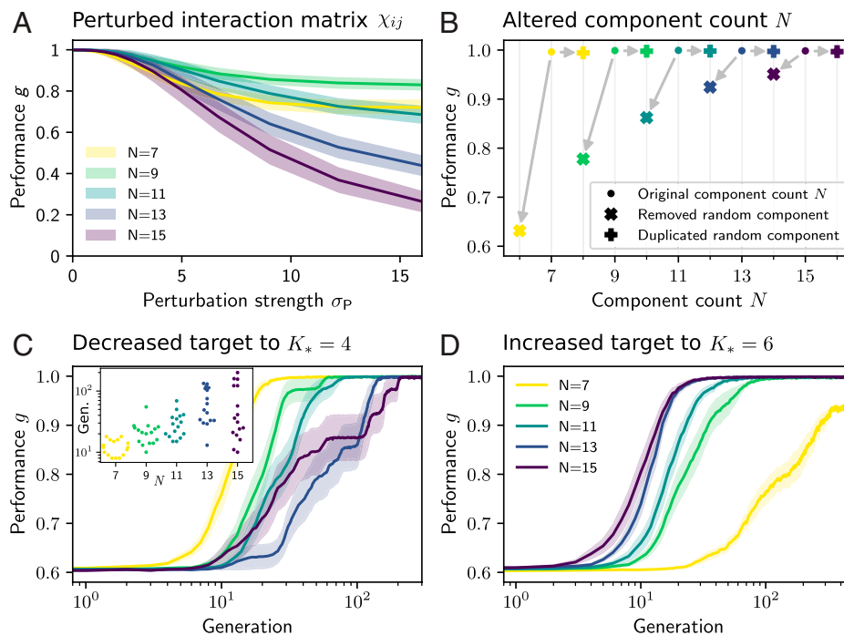
Fig. 5. Mixtures with more components are typically more robust. (A) Performance ( g ) \pm SD( g ) of optimized interaction matrices when one row (and column) is perturbed by normally distributed random numbers with SD \sigma_p for several component counts N at K_* = 5 . Averages are over all 256 optimized matrices from Fig. 4. For each matrix, g is determined from an ensemble of 64 perturbations and random initial conditions. (B) Performance g when a mixture optimized with N components loses (cross symbols) or duplicates (plus symbols) a component for various N at K_* = 5 . SD is smaller than symbol size. (C and D) Evolution of ( g ) \pm SEM( g ) as a function of generation when the target phase count is decreased from K_* = 5 to K_* = 4 (C) or increased from K_* = 5 to K_* = 6 (D) for several N . Each of the eight optimized populations from Fig. 4 is evolved twice. The Inset in C shows the generation at which individual trajectories exceed a performance of 0.8 for various N .
