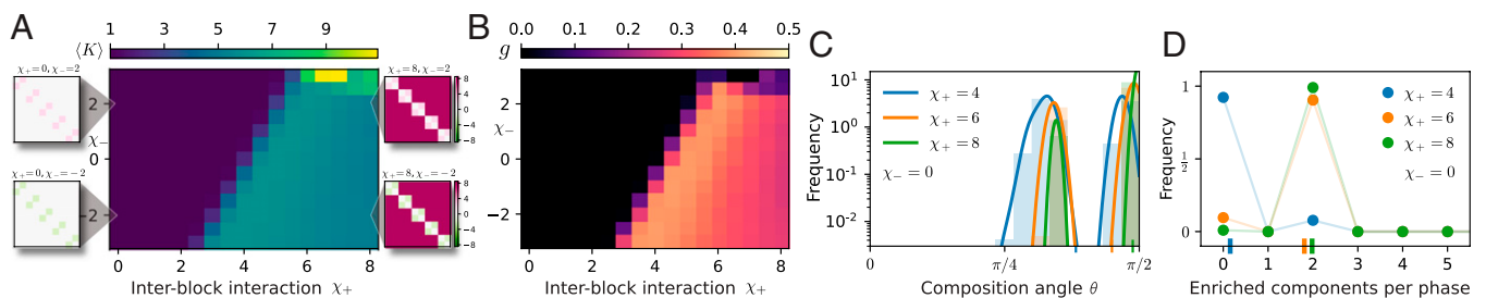
Fig. 3. Interaction matrices with block structure cannot target specific phase counts K reliably. (A and B) Mean phase count \langle K \rangle and performance g as functions of the interaction \chi_+ between different blocks and the interaction \chi_- within blocks for N = 10 components arranged in K_* = 5 equal blocks (Insets in A show example matrices). (C) Distribution of composition angles \theta shown as histograms and using kernel density estimation (lines) for several \chi_+ at \chi_- = 0 . (D) Distribution of the number of components enriched in phases for several \chi_+ at \chi_- = 0 . A–D show averages over 10^4 initial compositions. Distribution means are indicated by vertical bars.
