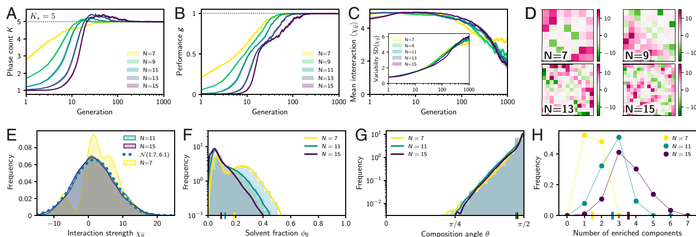
Fig. 4. Evolutionary optimized interactions result in reliable phase counts K . (A and B) Phase count K and performance g as functions of generation for different number of components N . The target phase count K_* = 5 and the maximal performance g = 1 are indicated by dotted lines. (C) Interaction strength \langle \chi_{ij} \rangle and \text{SD}(\chi_{ij}) as a function of generation. (D) Examples of optimized interaction matrices for various N . Components have been clustered by similarity. (E) Distribution of interaction strengths in the final matrices. The blue dotted line indicates a normal distribution that best fits the case N = 15 . (F and G) Distribution of the solvent fraction \phi_0 (F) and composition angles \theta (G) shown as histograms and using kernel density estimation (lines) for several N . The corresponding means are indicated as vertical bars. (H) Distribution of the number of components enriched in phases for several N with means indicated as vertical bars. In A–H, model parameters are K_* = 5 , w = 1 , \sigma_e = 0.3 , and \chi_{\text{bound}} = 5 . Each population contains 32 individuals, which were initialized with random matrices. A–C for each N show ensemble mean and associated SE (SEM) of eight independent repetitions. The statistics of the resulting 256 optimized matrices are shown in E–H.
