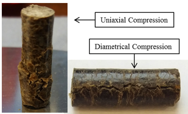
Fig. 8 Pellets after experimental compression tests
