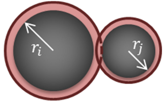
Fig. 4 Illustration of two spheres and their virtual radii in DEM
