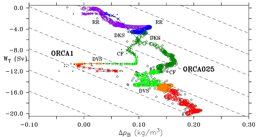
Figure 10. Scatterplot of the alongshore density difference \Delta\bar{\rho}_B (in \text{kg}/\text{m}^3 ) and the cumulative vertical transport W_T (in Sv), for (circles) ORCA025 and (crosses) ORCA1 along the path outlined in Figure 6 (black symbols: data for each grid point, colored symbols: five-point smoothed values). Key locations are labeled, the color coding indicates the path segment in accordance with Figure 6 (purple: start-RR, blue: RR-DKS, dark green: DKS-CF, light green: CF-DVS, orange: DVS-western Labrador Sea, red: western Labrador Sea-end). Dashed lines indicate the theoretical slope gz_{\text{sink}}^2/2\rho_0f that follows from equation (1).
