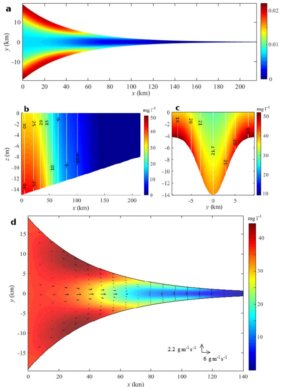
Figure 9. Same as Figure 8, but for f = 0 , w_s = 0.2 \text{ mm} \cdot \text{s}^{-1} and d_s = 10 \text{ } \mu\text{m} . The cross section in Figure 9c is taken at x = 30 \text{ km} .
