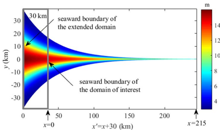
Figure 2. The bathymetry and geometry of the extended domain, and the (nonextended) domain of interest.
