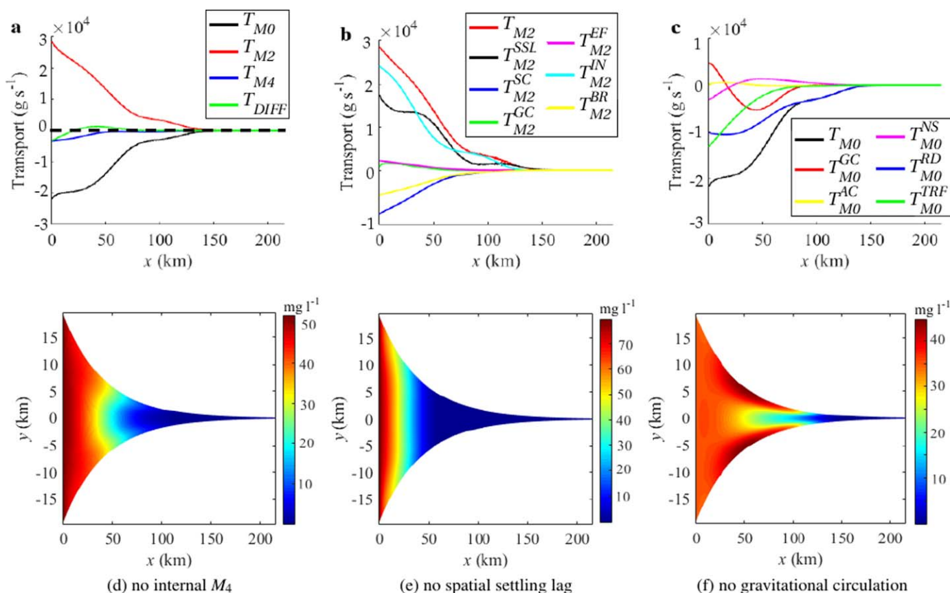
Figure 10. Same as (top) Figure 6 and (bottom) Figure 7, but for w_s = 0.2 \text{ mm} \cdot \text{s}^{-1} and d_s = 10 \text{ } \mu\text{m} .
