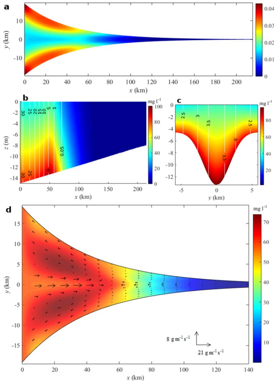
Figure 15. Same as Figure 8, but for Q = 864 \text{ m}^3 \cdot \text{s}^{-1} . The cross section in Figure 15c is taken at x = 50 \text{ km} .
