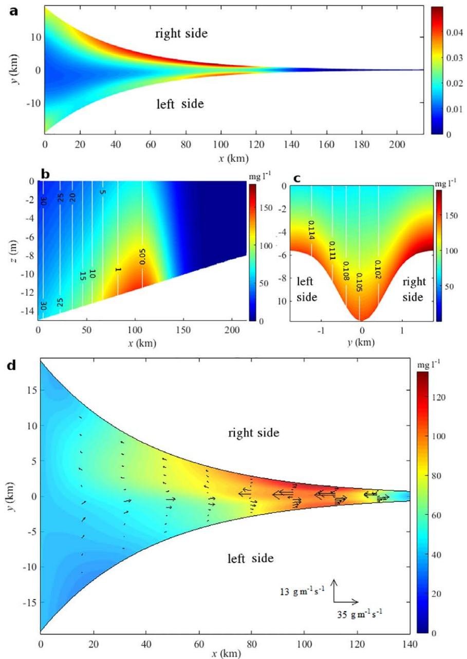
Figure 8. Same as Figures 3 and 4, but for f=1 \times 10^{-4} rad s -1 .
