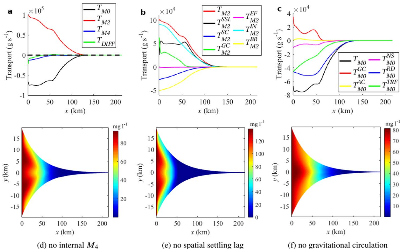
Figure 16. Same as (top) Figure 6 and (bottom) Figure 7, but for Q = 864 \text{ m}^3 \cdot \text{s}^{-1} .
