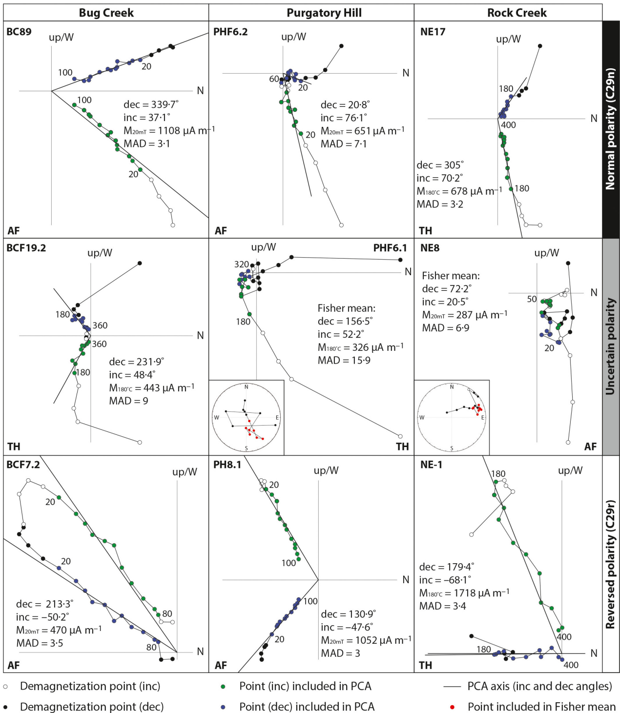
Fig. 4. Zijderveld diagrams of TH and AF demagnetized samples characteristic for the magnetostratigraphy of the Tullock Member at Rock Creek, Purgatory Hill and Bug Creek. In samples with a clear reversed polarity, stable ChRM components of inclination (inc) (open circles) and declination (dec) (solid circles) were isolated from the secondary present-day overprint component upward from 180°C (TH) and 20 mT (AF). Samples with a normal polarity were interpreted assuming similar unblocking spectra of the ChRM component. Points included in the anchored PCA are indicated for declination (blue) and inclination (green). In two panels (middle and middle-right), equal area plots have been included since these directions are calculated with a Fisher mean. Points included in the Fisher mean are indicated in red. Magnetostratigraphic polarity plots of inclination, declination and ChRM intensity for the different composite sections are shown in Figure S2 (A to E).
