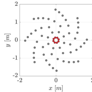
b) Underbrink spiral microphone distribution
