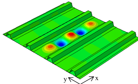
Figure 2. First buckling mode of four-stringer panel.
