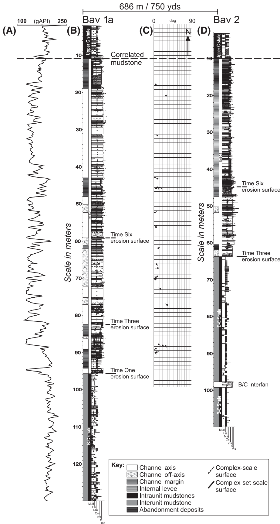
Figure 6. Correlation panel between boreholes Bav 1a and Bav 2 using the Upper C mudstone as a datum: (A) Gamma-ray log through Bav 1a; (B) Bav 1a sedimentary log (no well logs were run in this borehole). (C) Dipmeter measurements of erosion surfaces in subunit C2. (D) Bav 2 sedimentary log. Csi = coarse-grained siltstone; fs = fine-grained sandstone; Fsi = fine-grained siltstone; ms = medium-grained sandstone; Msi = medium-grained siltstone; Mud = mud grade sediment; vfs = very fine-grained siltstone.
