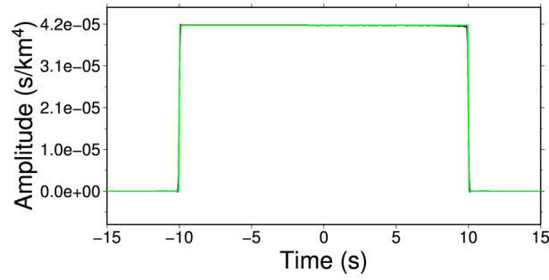
Figure 6. Stacked cross correlation resulting from a spherical distribution of sources surrounding the two receivers, predicted (green line) by the approximate analytical formula (53) and computed (black) numerically as described in section 4.2 and already illustrated in Figure 3 (only the real part is shown here). The source/station setup is the same as for Figure 3.
