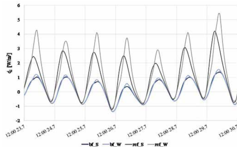
Fig. 6 Heat flux on the inner surface of the south- and west oriented façade with (bf) and without (ref) the bionic façade in Madrid.
