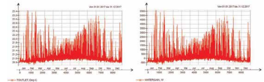
Fig. 12 Outlet temperature and heat gain of the FFG on the south façade.
