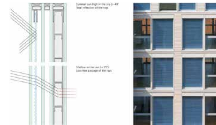
Fig. 5 Example of triple glass component. The prismatic panel reflects the radiation during summer and instead allows the heating of the thermal storage module (PCM in a polycarbonate box) in the winter season. The whole system, which looks like a translucent window, has a thickness of 80 mm, a thermal transmittance of 0.48 W/m 2 K and a light transmission coefficient that can reach up to 45% (GlassX AG technical documentation - www.glassx.ch).
