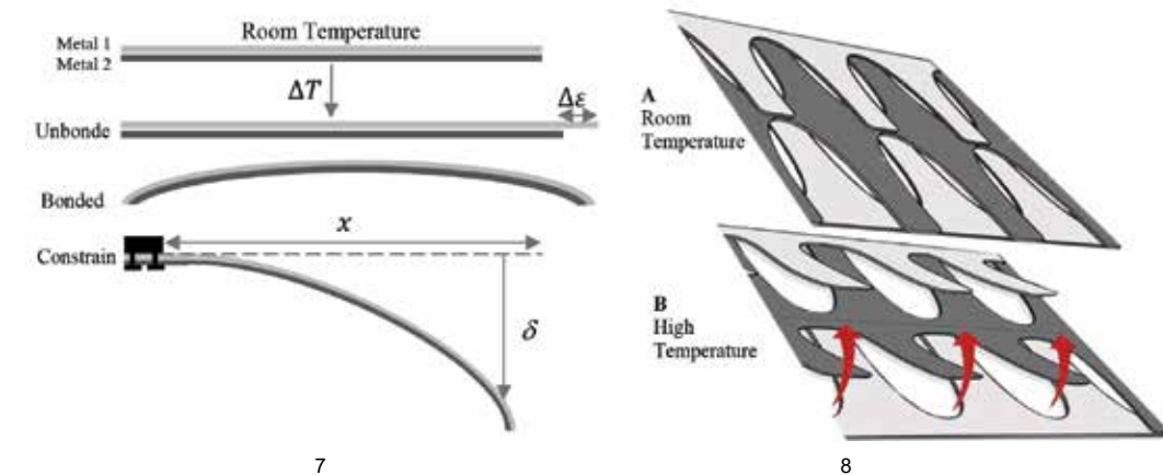
Fig. 7 Bimetal Strip. Two metals bonded together with different expansion coefficients. Fig. 8 Bloom Research Installation Los Angeles. Panel behavior Position A. Room temperature, closed module, Position B. High temperature, opened module.
