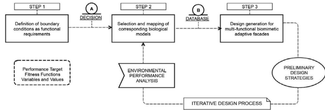
Fig. 3 A new framework for designing multi-functional biomimetic adaptive façades
