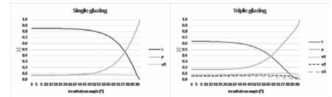
Figure 3 – Fresnel solution for single glazing (left) and TGU (right) with transmission \tau , external reflection \rho and absorption coefficients for each glass pane a_i (where 1 is the external and 3 internal glass pane)
