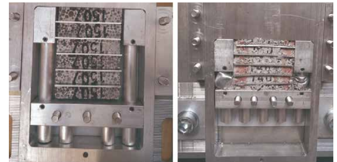
Fig. 5 Dissipative bracket. a) Dissipative bracket in undeformed state with hybrid crash components aluminium sleeves and dissipative concrete. b) Dissipative bracket after inward testing.
