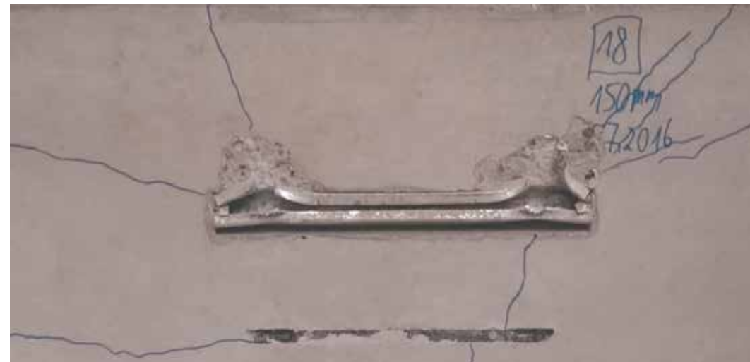
Fig. 10 Typical failure mode for both standard and rebar channels in the experimental investigations.
