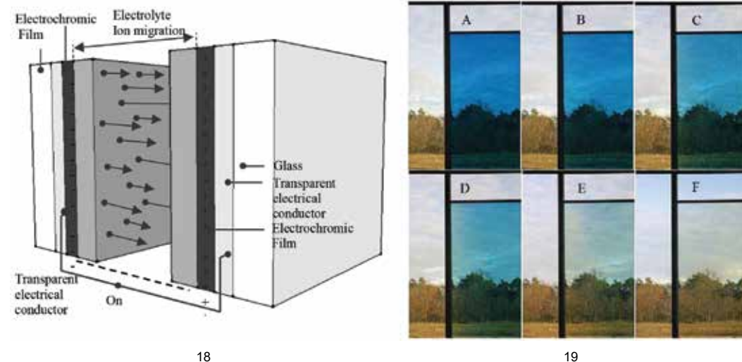
Fig. 18 The basis is a glass or plastic covered by a transparent conducting film, on multiple cathodic electroactive layers is affixed. A layer of ion conductor follows these, on its turn followed by an ion-storage film or one (or multiple) complimentary anodic electroactive layers and another transparent conducting film. Fig. 19 Tungsten Oxide Electrochromic coated window, the process of change of conductive and reflecting properties From A (blue) to F (transparent) M_xWO_3 \leftrightarrow WO_3 + xM^+ + xe reproduced from Gesimat (2009).
