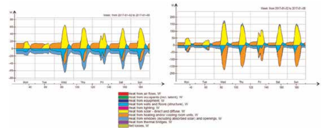
Fig. 11 Results for 100% FFG modules (left) and solar coated standard glazing (right).
