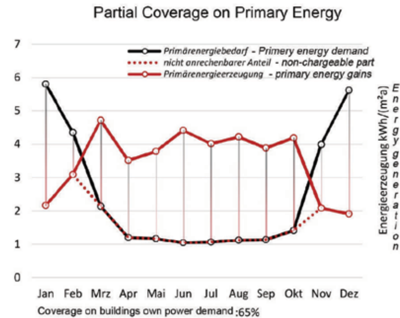
Fig.22: enerCalc-program: final energy balance - partial coverage on primary energy - 3rd configuration
