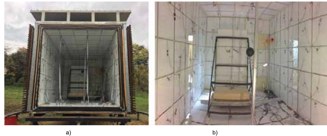
Fig.5. Overview of: a) the Heat Flux Tiles system inside the Test Room; b) Connection in series by means of flat cables and interface modules to obtain final signals.
