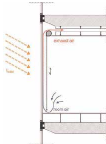
Fig. 1 Operation mode Active Cavity Transition Facade
