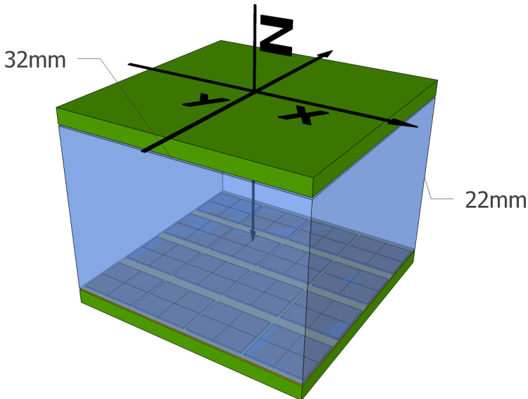
Figure 4.1: Sketch of a partially assembled dual-sided readout detector with the reference system used in the analysis.
