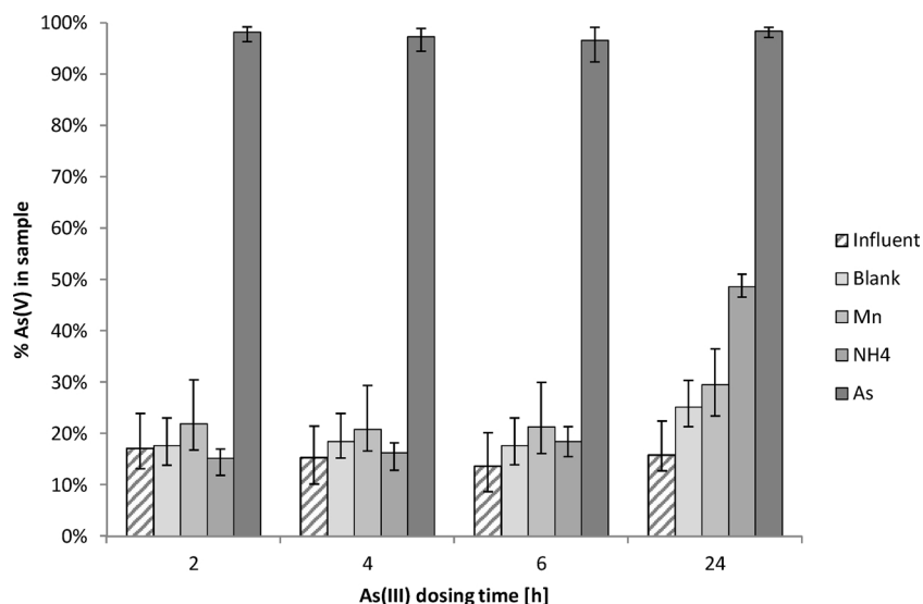
Fig. 3. Percentage of As(V) of total As in water sample during 24 h in the preloaded sand columns. Samples obtained from influent and filtrate of the filter sand columns after preloading with drinking water, NH 4 , As(III) or Mn(II).
