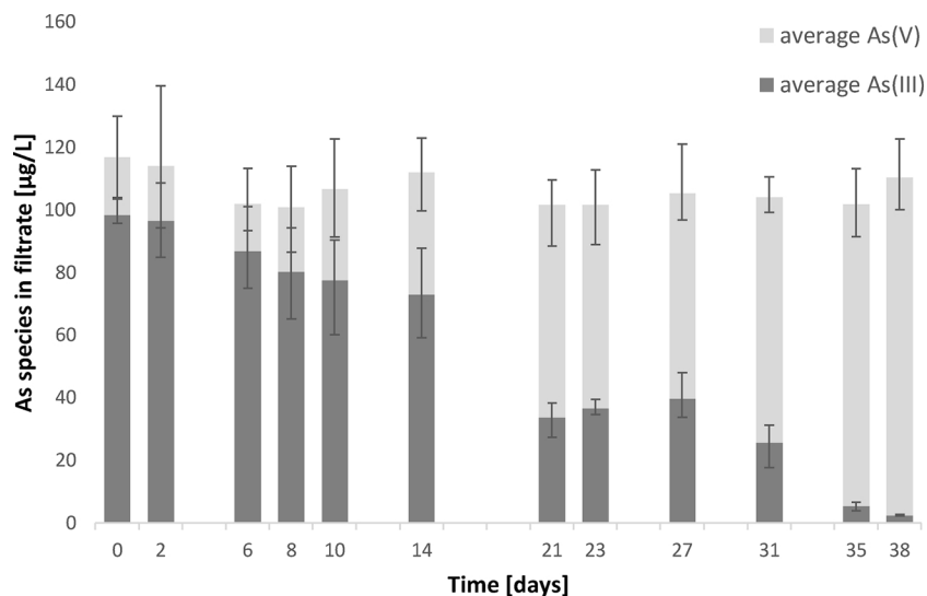
Fig. 4. As(III) and As(V) species in the filtrate of sand columns over time (38 days) by feeding drinking water added with approximately 100 µg/L As(III).
