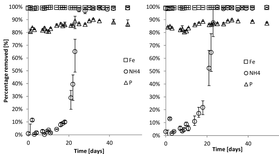
Fig. 7. Removal percentage of Fe, \text{NH}_4 and P over time in virgin sand columns (Left) and As(III) preloaded sand columns (Right). Filtration velocity 1 m/h; bed height 0.5 m. Initial concentration of the groundwater: Fe 1.4 mg/L; As 13 \mu\text{g/L} (as As(III)); \text{PO}_4 0.45 mg/L; Mn 0.04 mg/L; \text{NH}_4 0.62 mg/L; pH 7.54; Water temperature 14 – 18 °C. After aeration/supernatant level: \text{O}_2 4.4 mg/L; pH 7.65.
