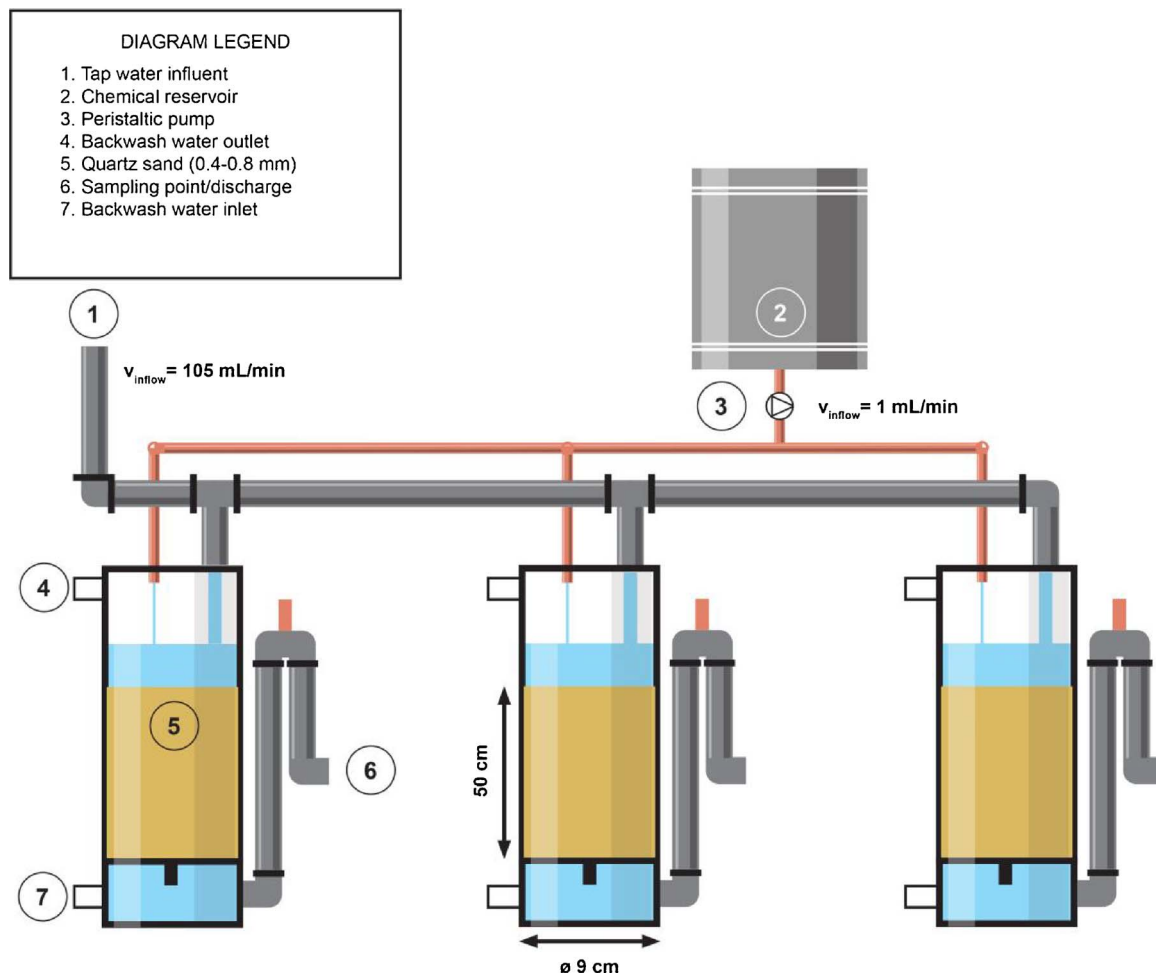
Fig. 1. Schematic overview of sand filter set-up as triplicates (valves not shown).
