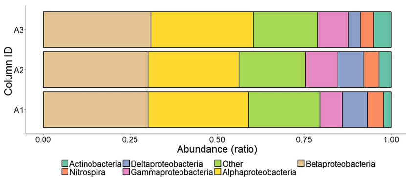
Fig. 5. Results of microbial community analysis after feeding drinking water with 100 µg/L added As(III) for 38 days. Relative abundance of bacteria is shown at the taxonomic rank Class (L3) of the filter sand columns ID's A1, A2 and A3 (triplicates).
