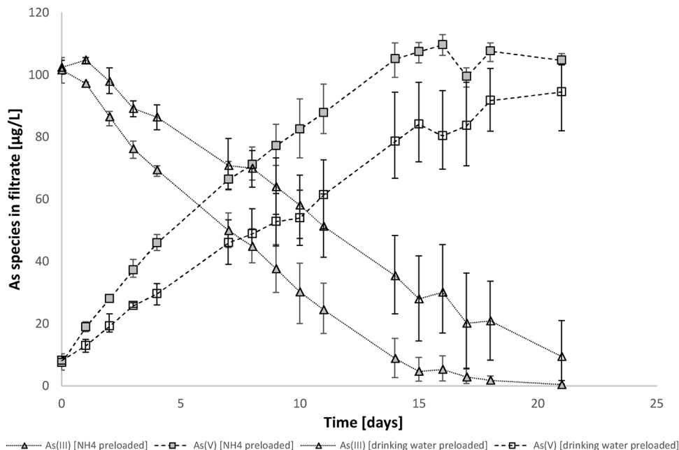
Fig. 6. As(III) and As(V) in the filtrate of drinking water pre-loaded columns spiked with and without 0.79 mg/L-N NH 4 . Influent As(III) concentration was 98 µg/L min 83 max 118 (n = 16) As(III) spiked in drinking water.
