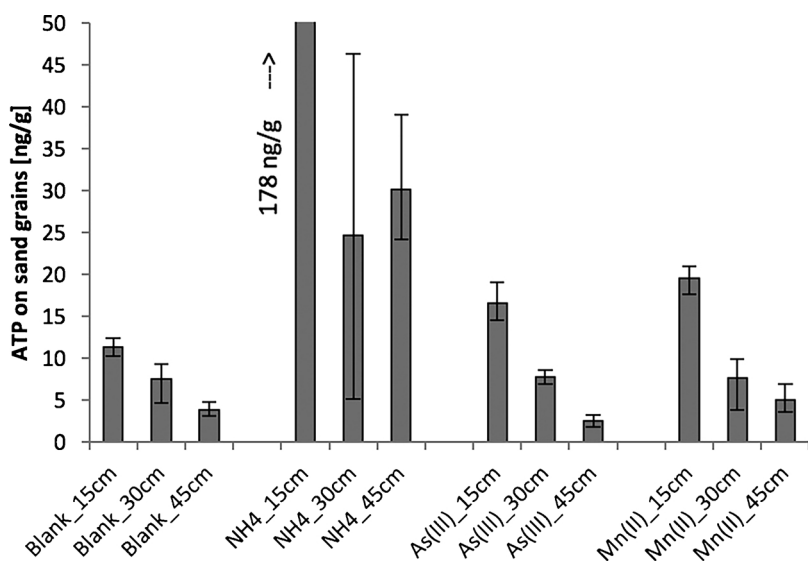
Fig. 2. ATP concentration on the filter sand at 15, 30 and 45 cm from top of the filter after preloading with drinking water (blank), NH 4 , As(III) or Mn(II). Two outliers removed with 95% certainty interval with Dixon’s Q-test.
