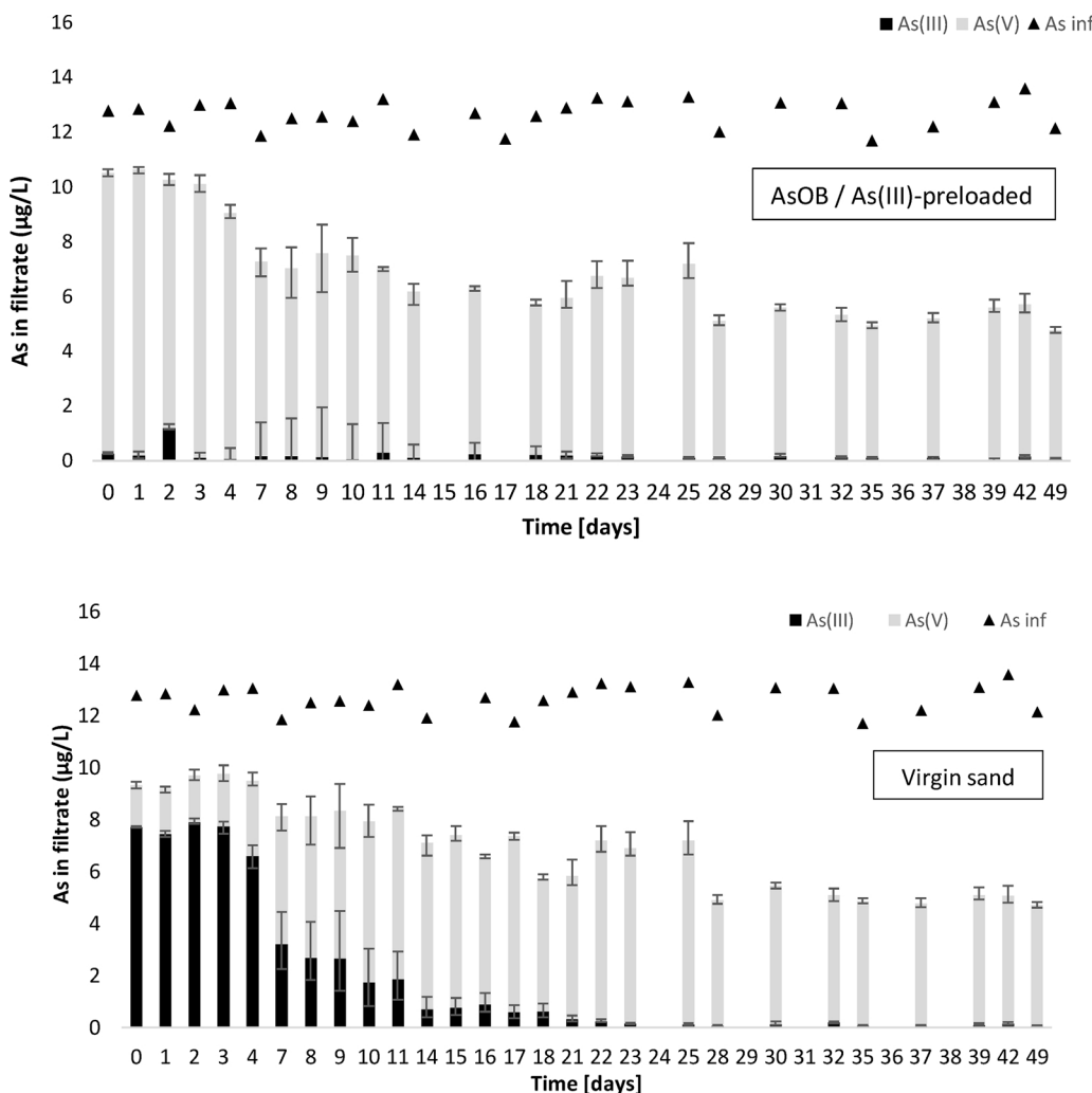
Fig. 8. As(III) and As(V) in the filtrate of As(III) preloaded (top) and virgin sand columns (bottom) over time. Filtration velocity 1 m/h and bed height 0.5 m. Initial concentration of the groundwater: Fe 1.4 mg/L; As 13 µg/L (as As(III) also depicted < > ; PO 4 0.45 mg/L; Mn 0.04 mg/L; NH 4 0.62 mg/L. As concentration in the filtrate is depicted as the sum of the As(III) and As(V) species.
