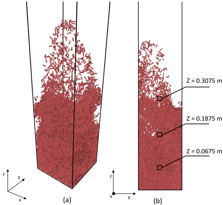
Fig. 6. (a) Snapshot of the fluidised bed reactor with fluid velocity 1.7U_{mf} where the hydrodynamic force case is “Drag only”. (b) Analysis positions in the bed reactor along the z-direction. These system snapshots were visualised using OVITO (Stukowski, 2010).
