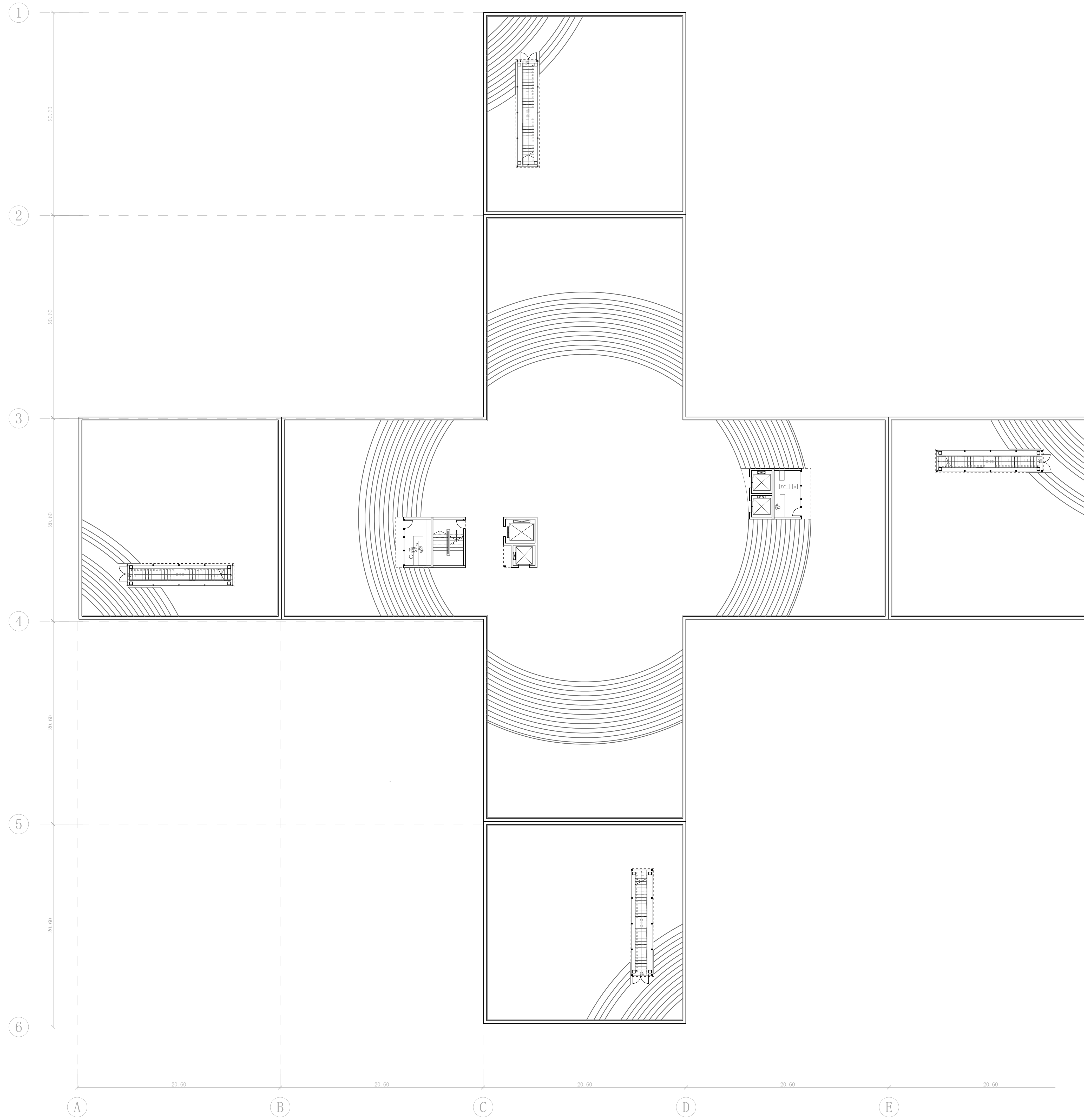
Roof Plan - Cinema - 1:200
