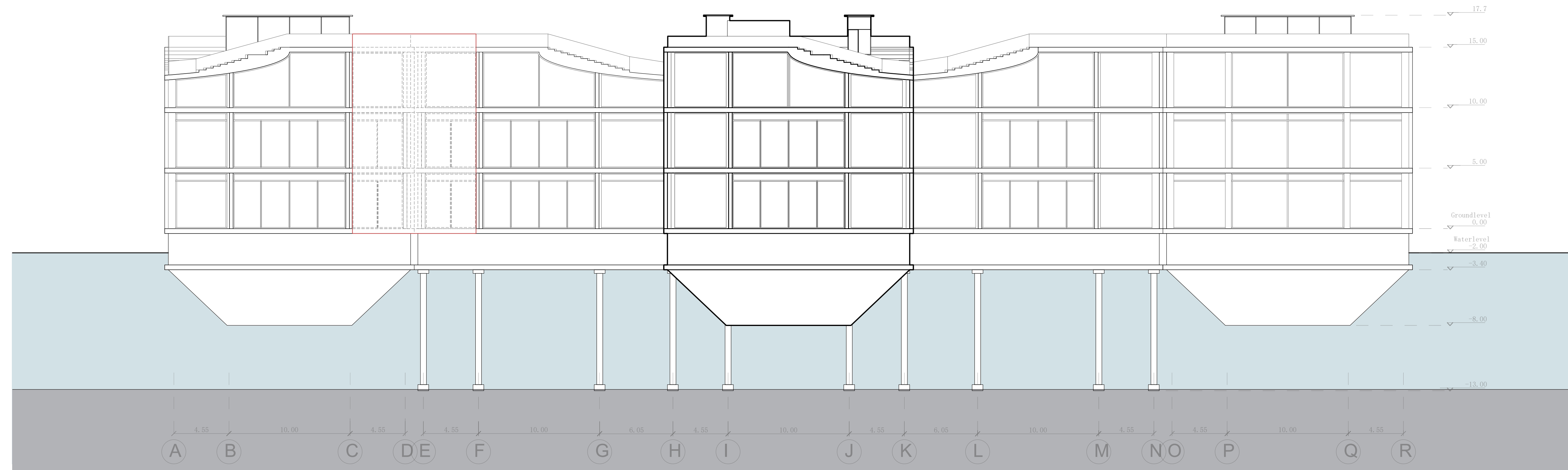
North Elevation - Cinema - 1:200
