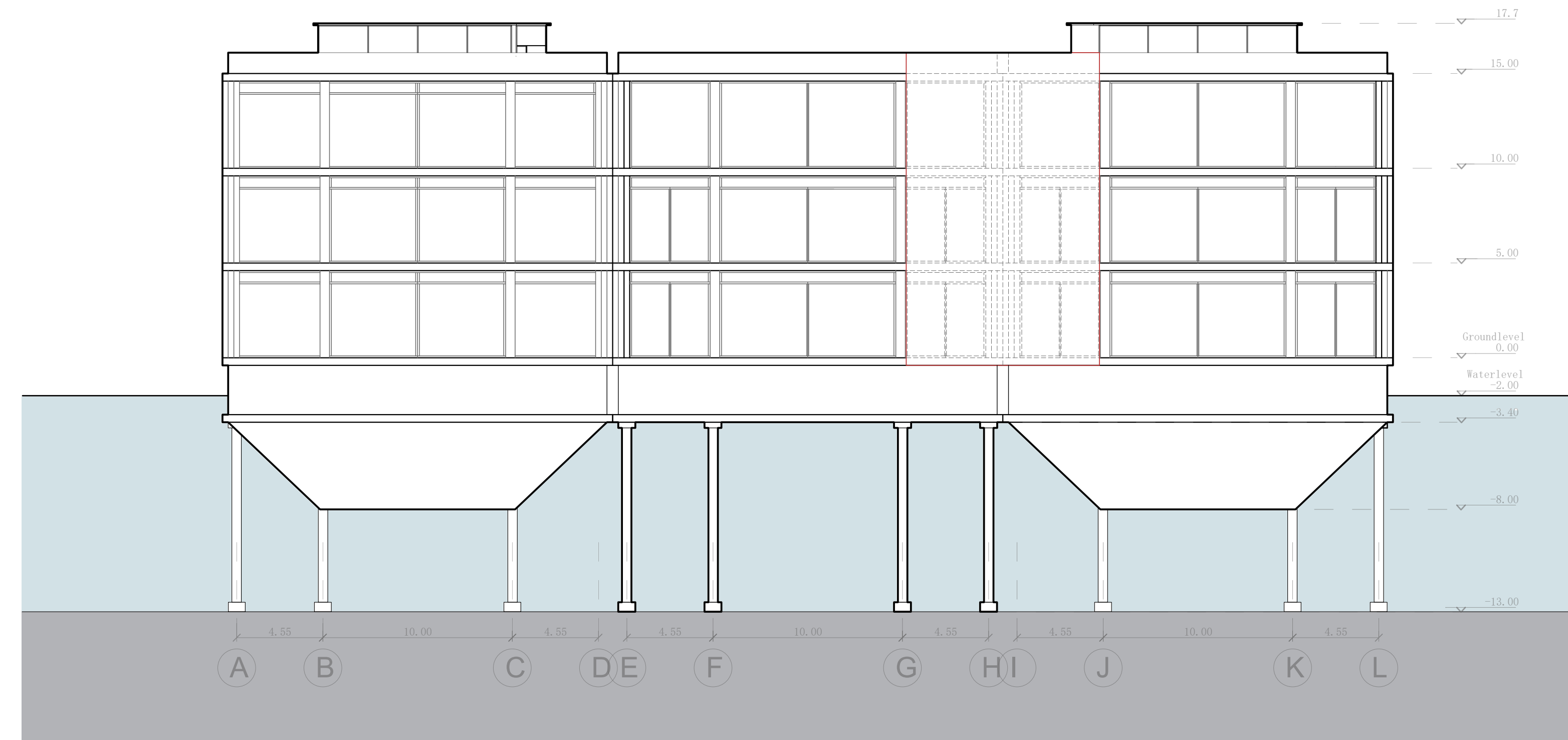
North Elevation - Festival - 1:200
