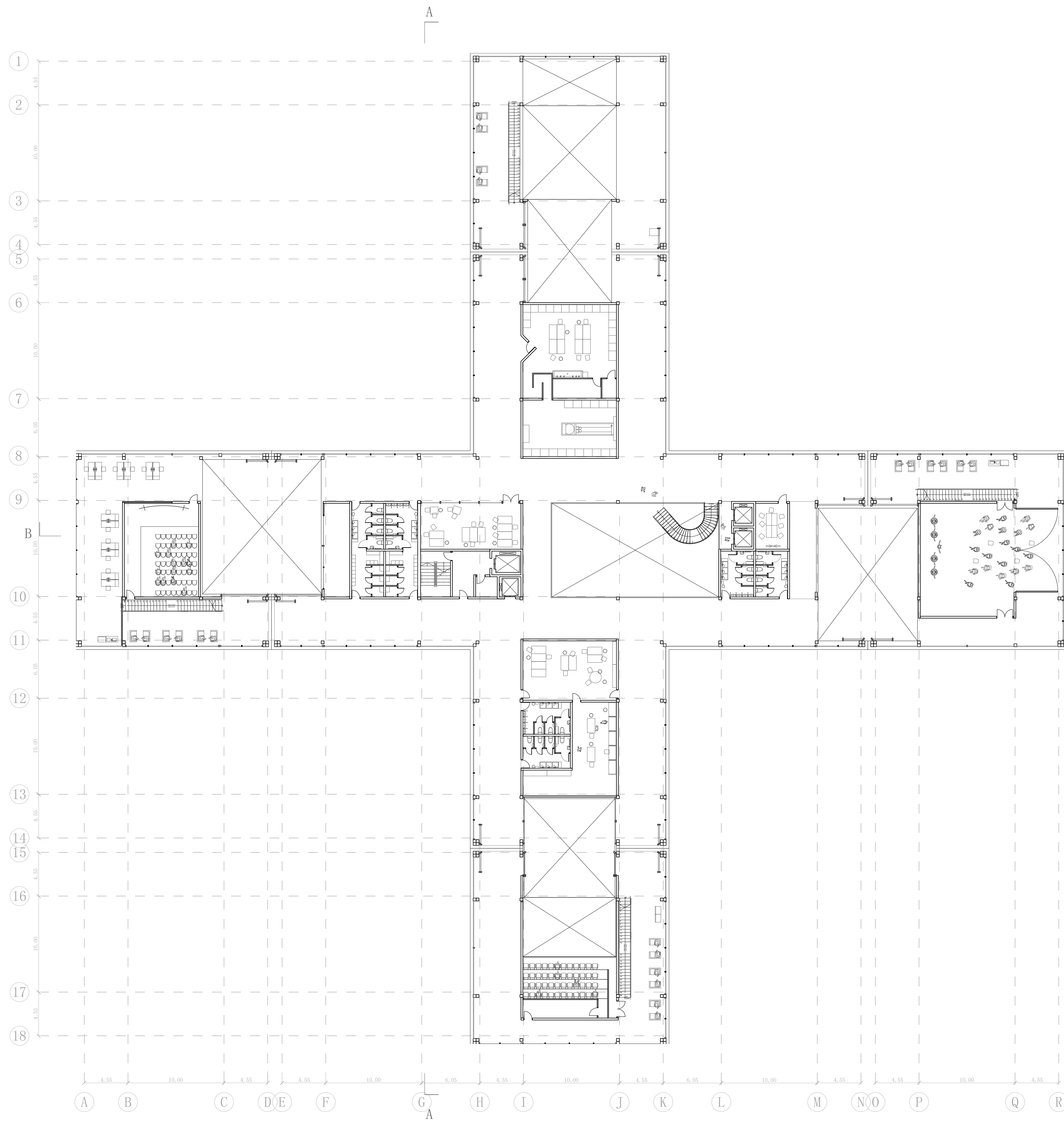
1st Floor Plan - Cinema - 1:200
