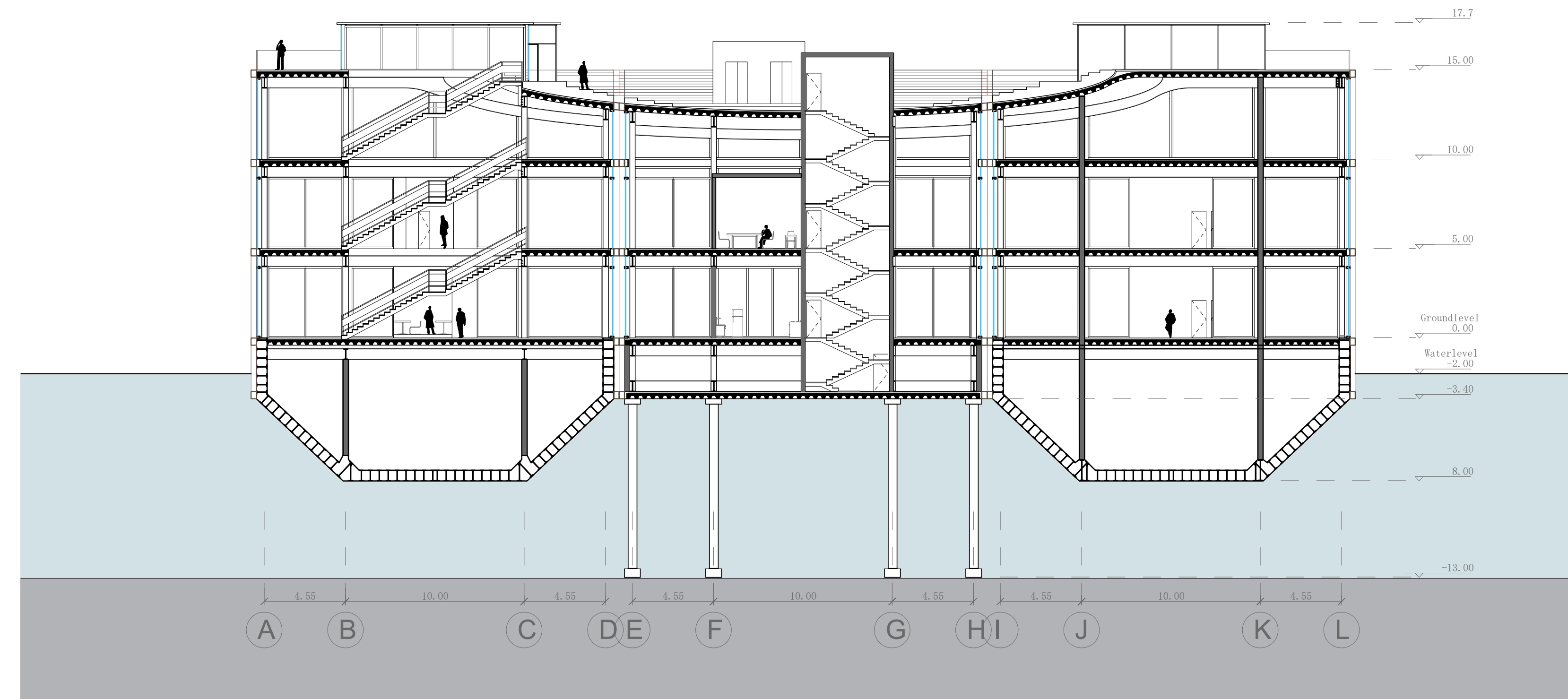
A-A Section - Festival - 1:200
