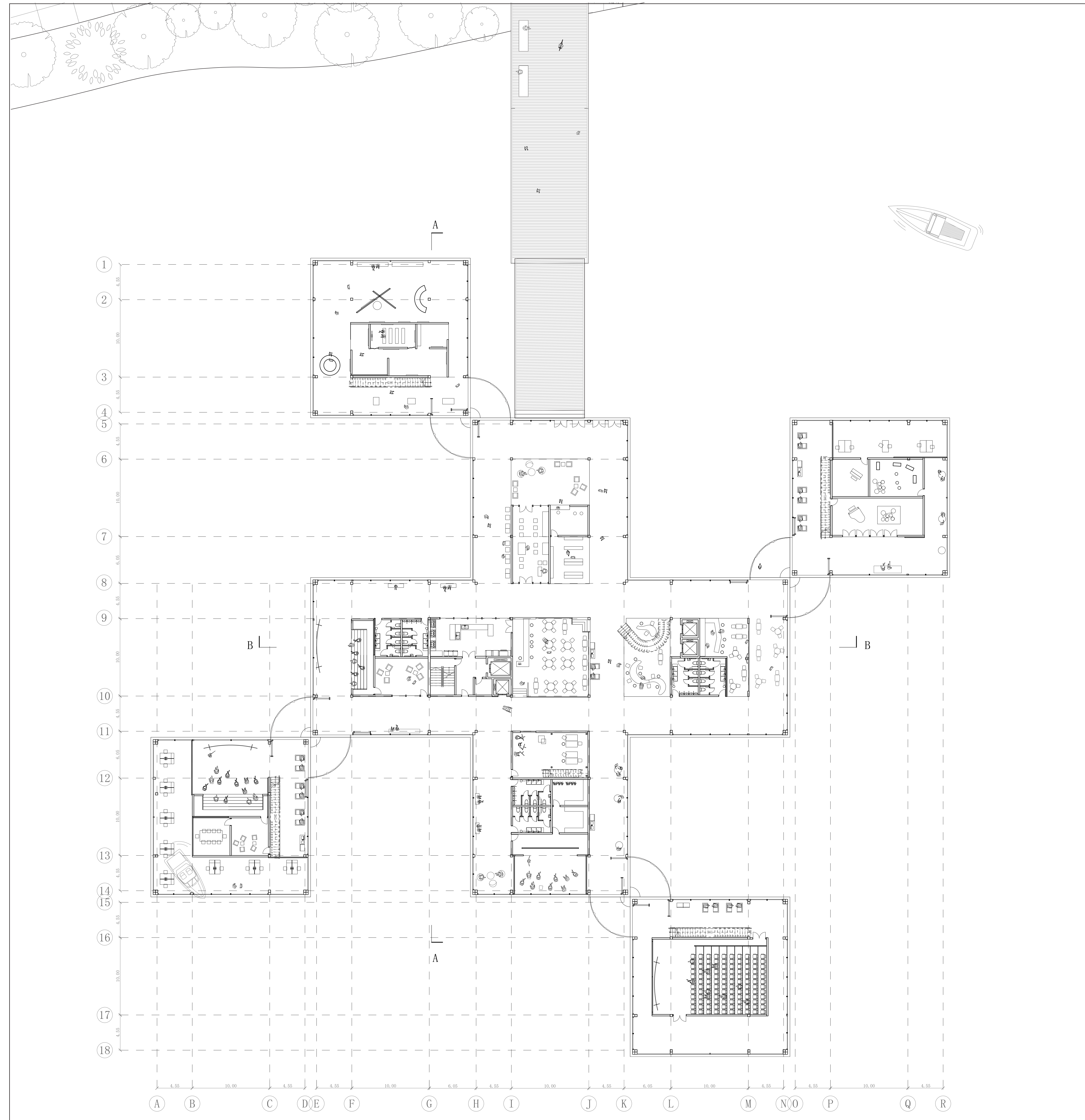
Ground floor Plan - Theater School - 1:200
