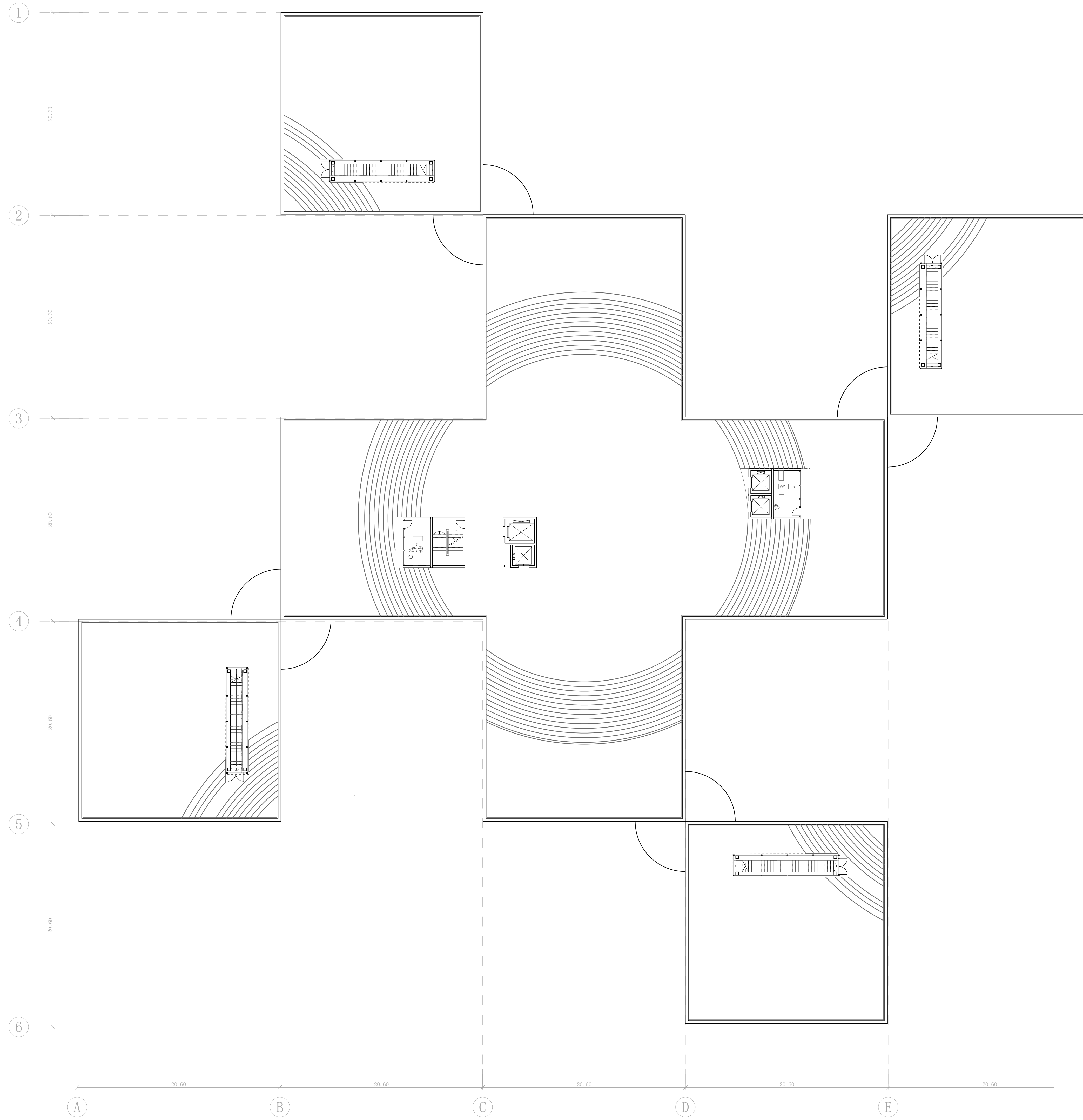
Roof Plan - Theater School - 1:200
