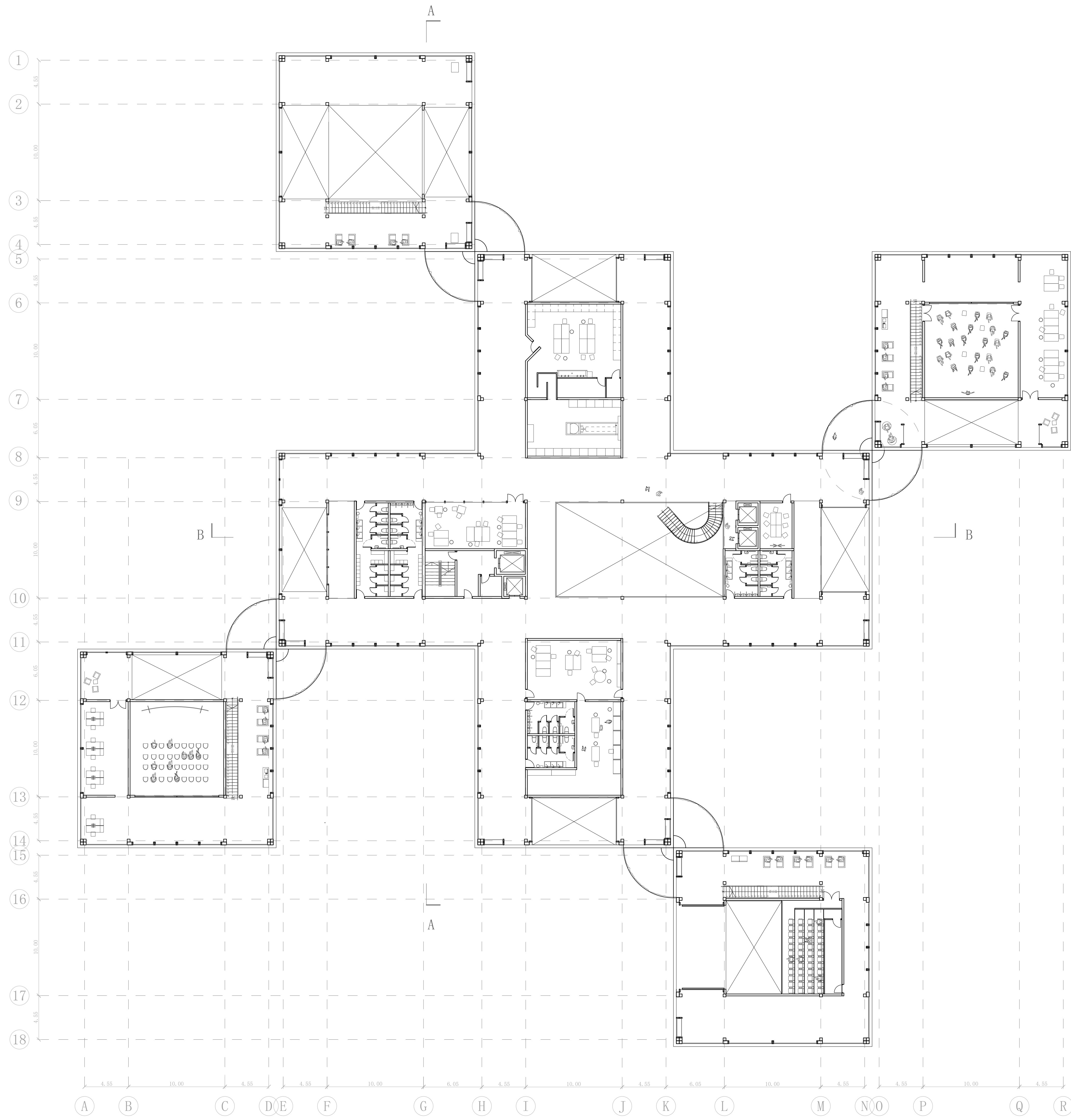
1st Floor Plan - Theater School - 1:200
