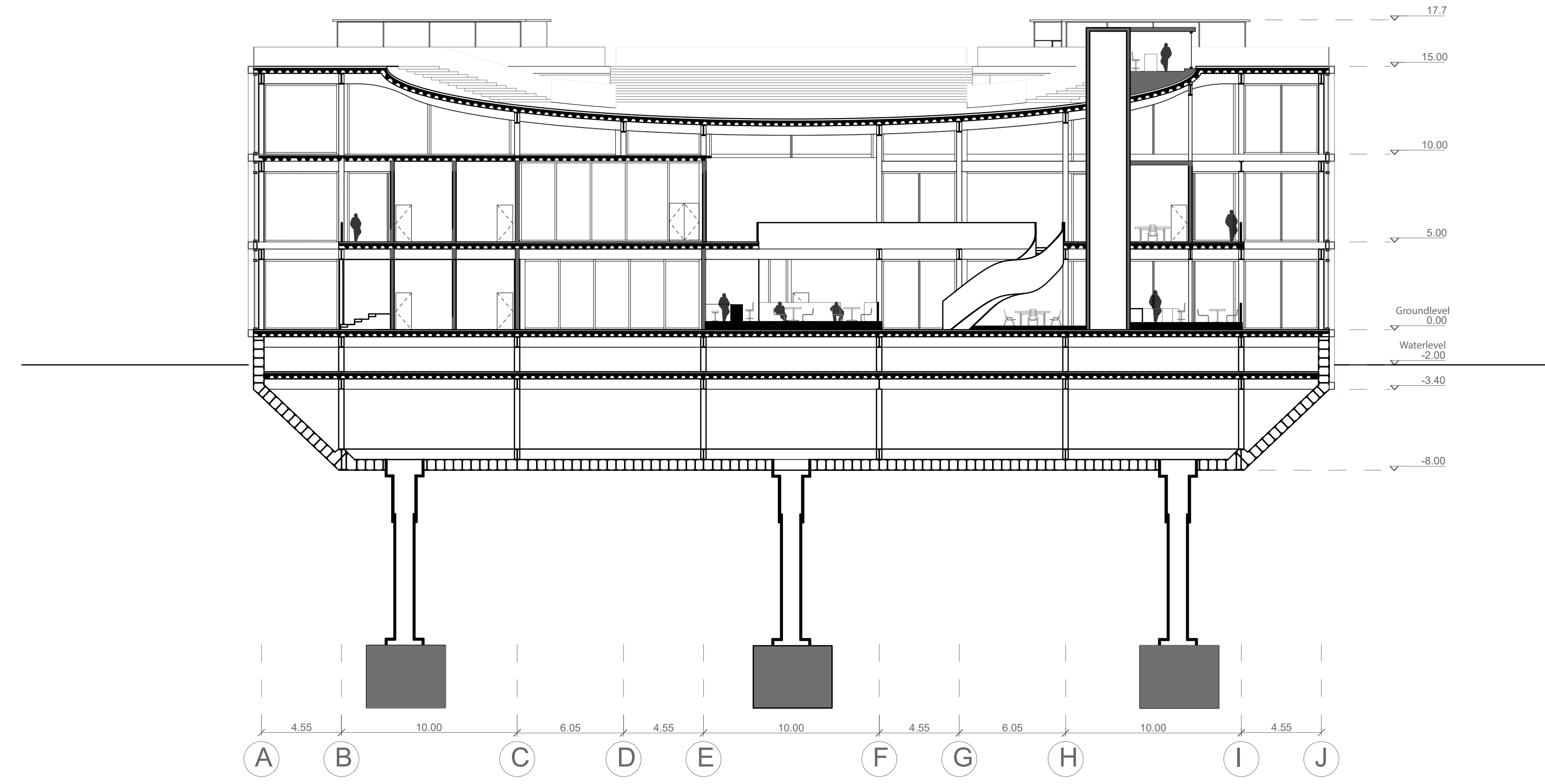
B-B Section - Festival - 1:200
