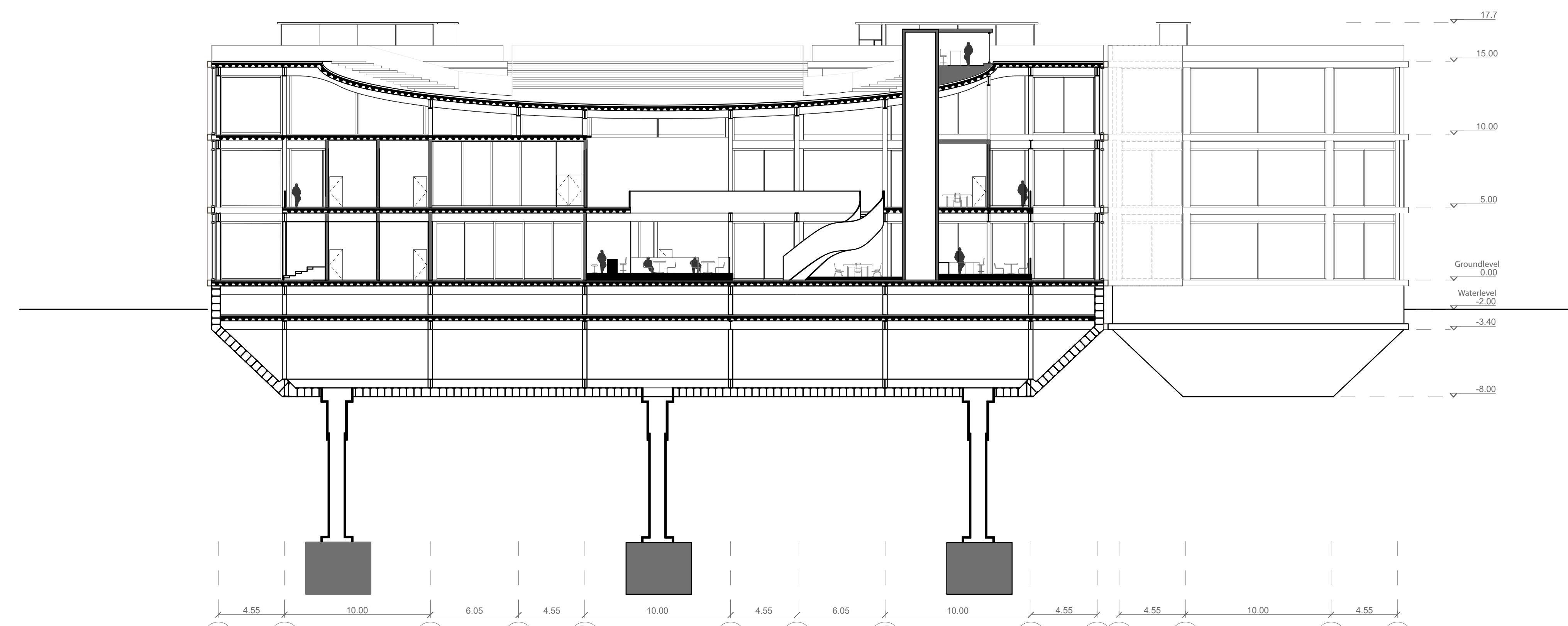
B-B Section - Theater School - 1:200
