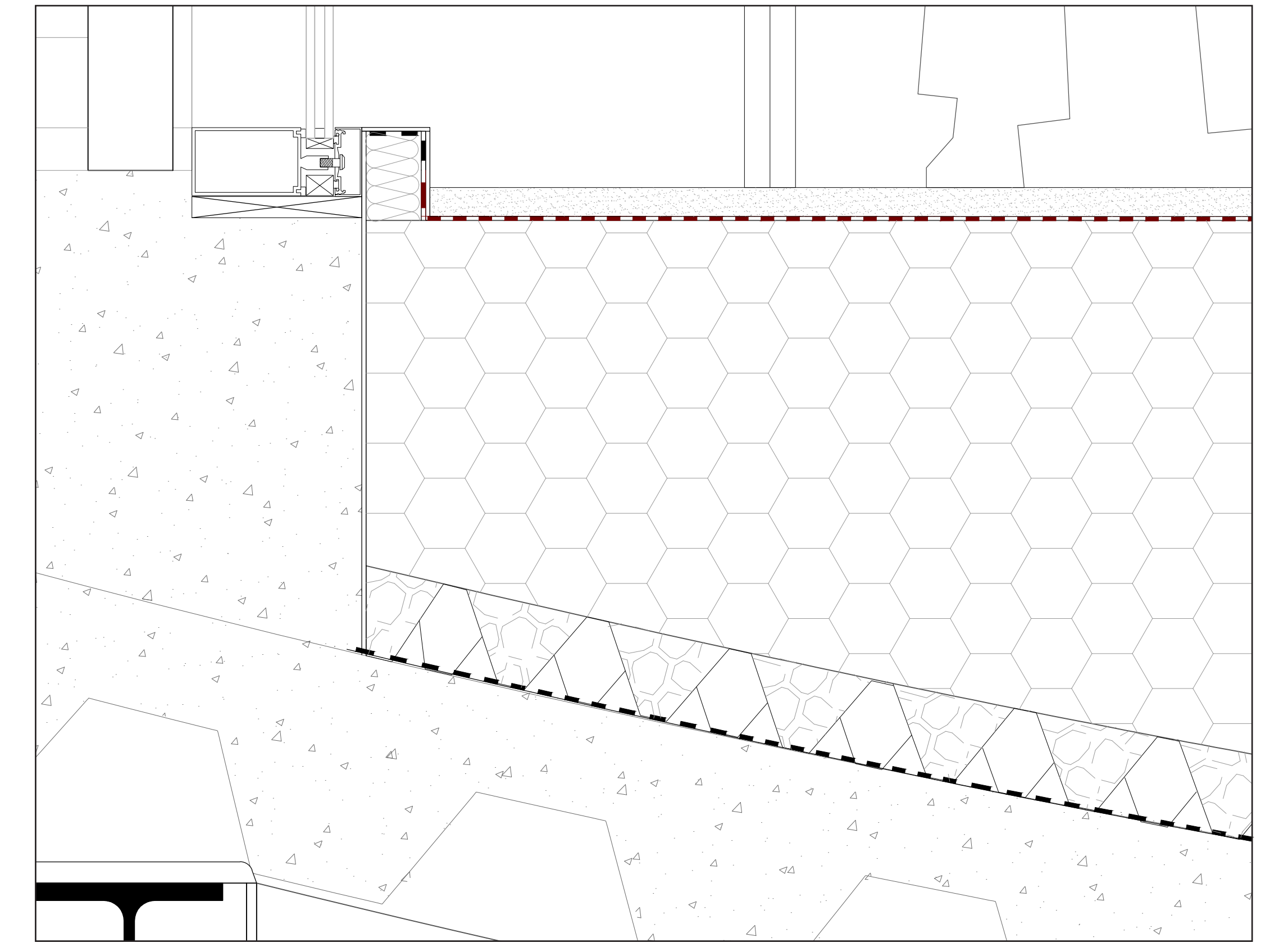
Detail- 1:5
