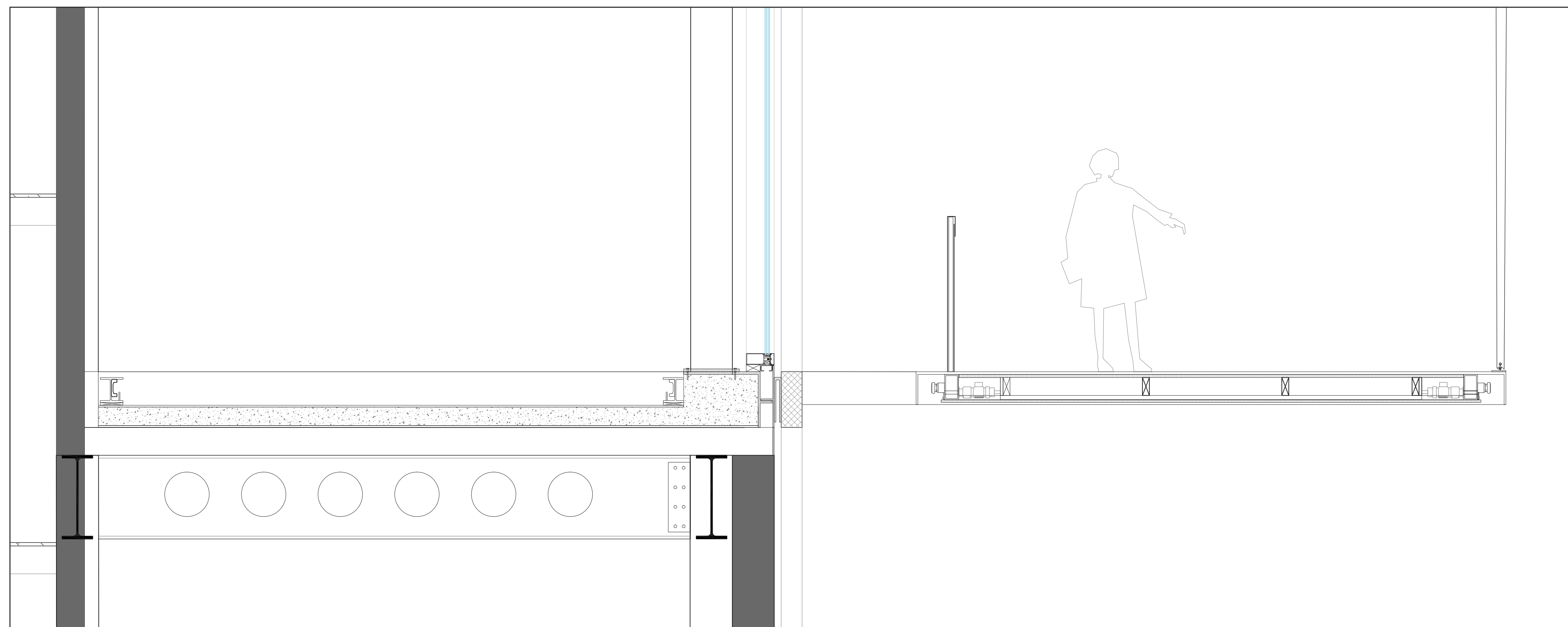
Section Fragment- Sliding - 1:20
