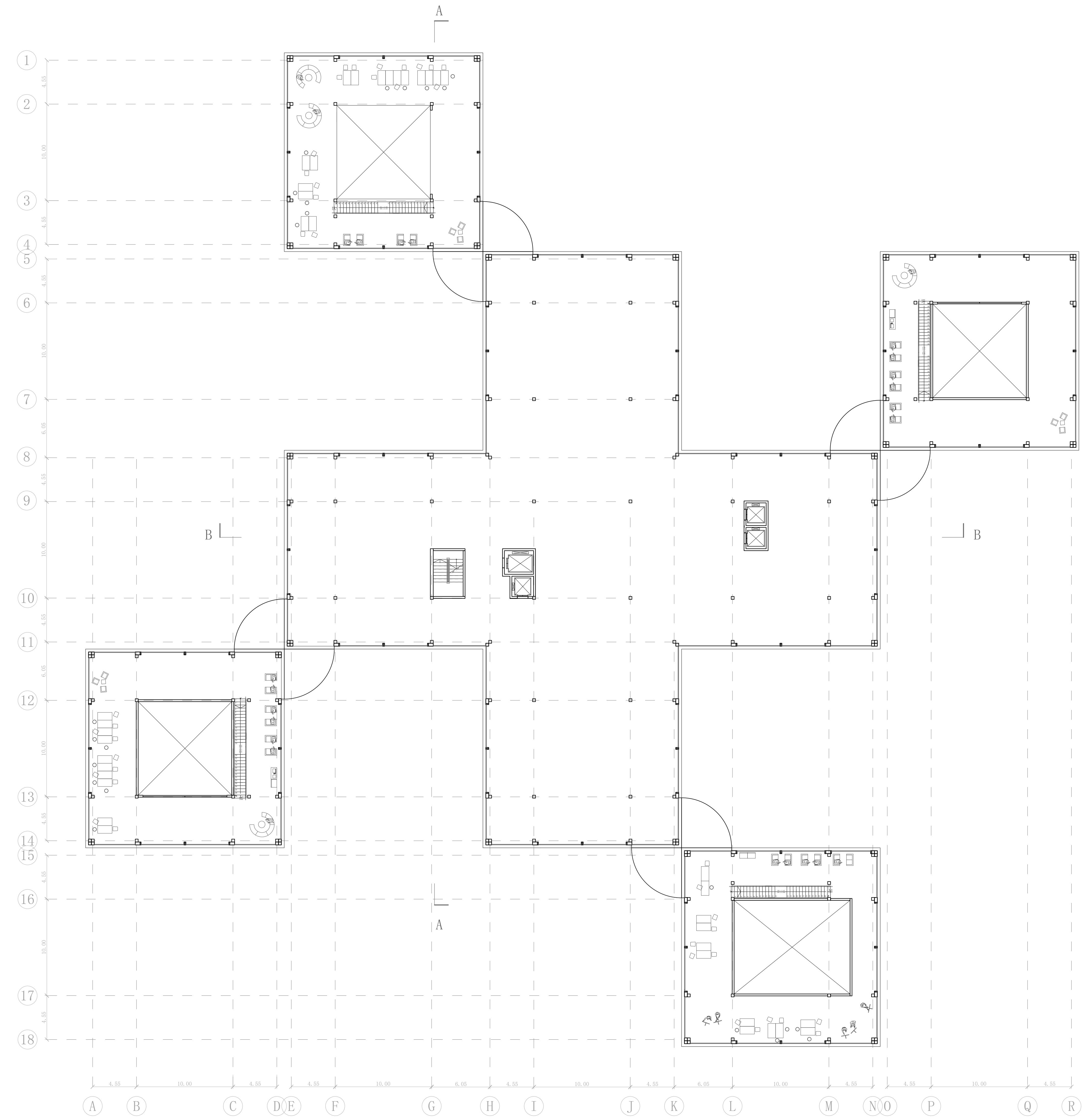
2nd Floor Plan - Theater School - 1:200
