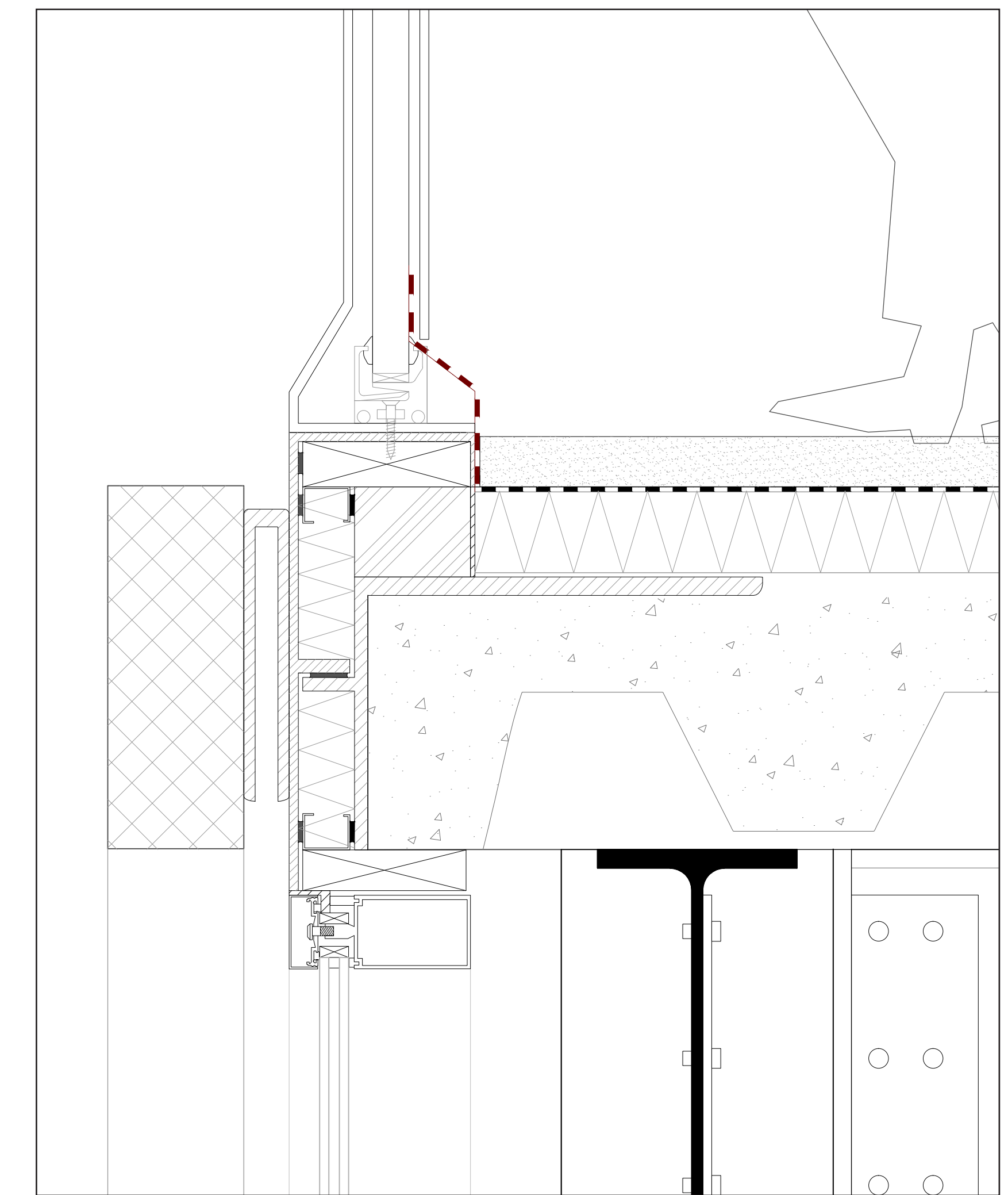
Facade detail- 1:5
