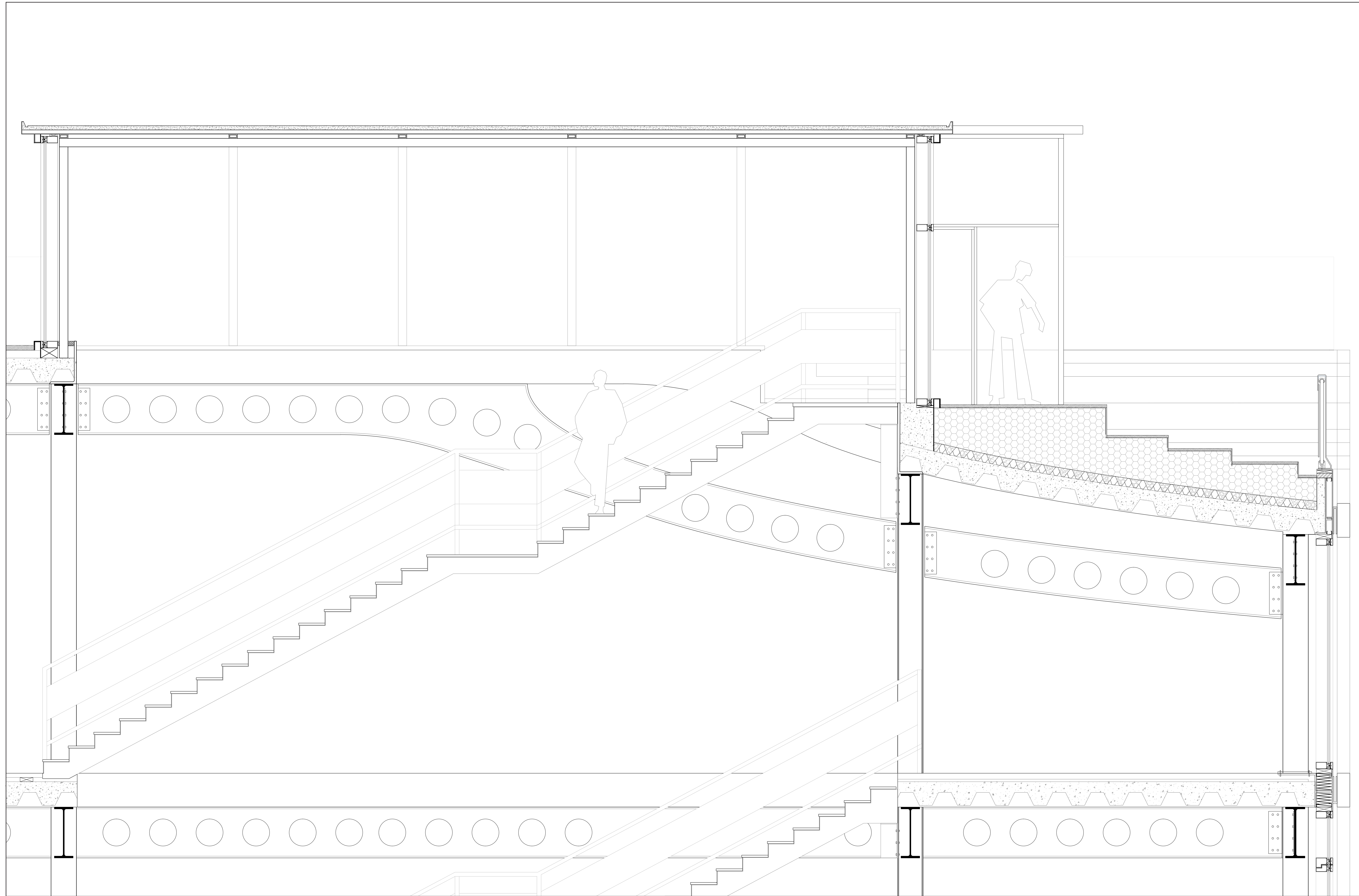
Section Fragment - 1:20
