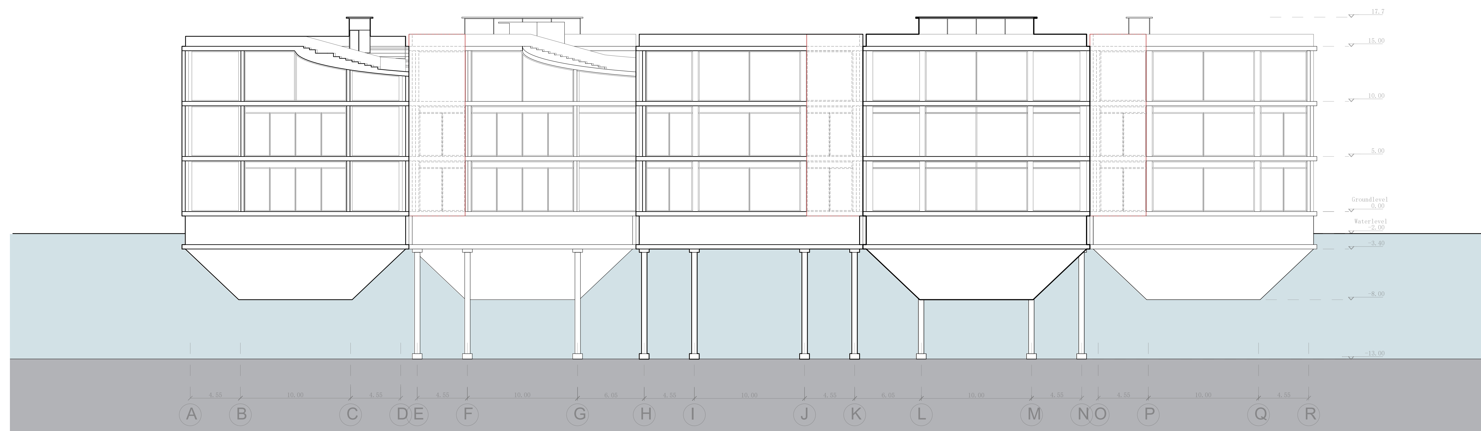
North Elevation - School - 1:200
