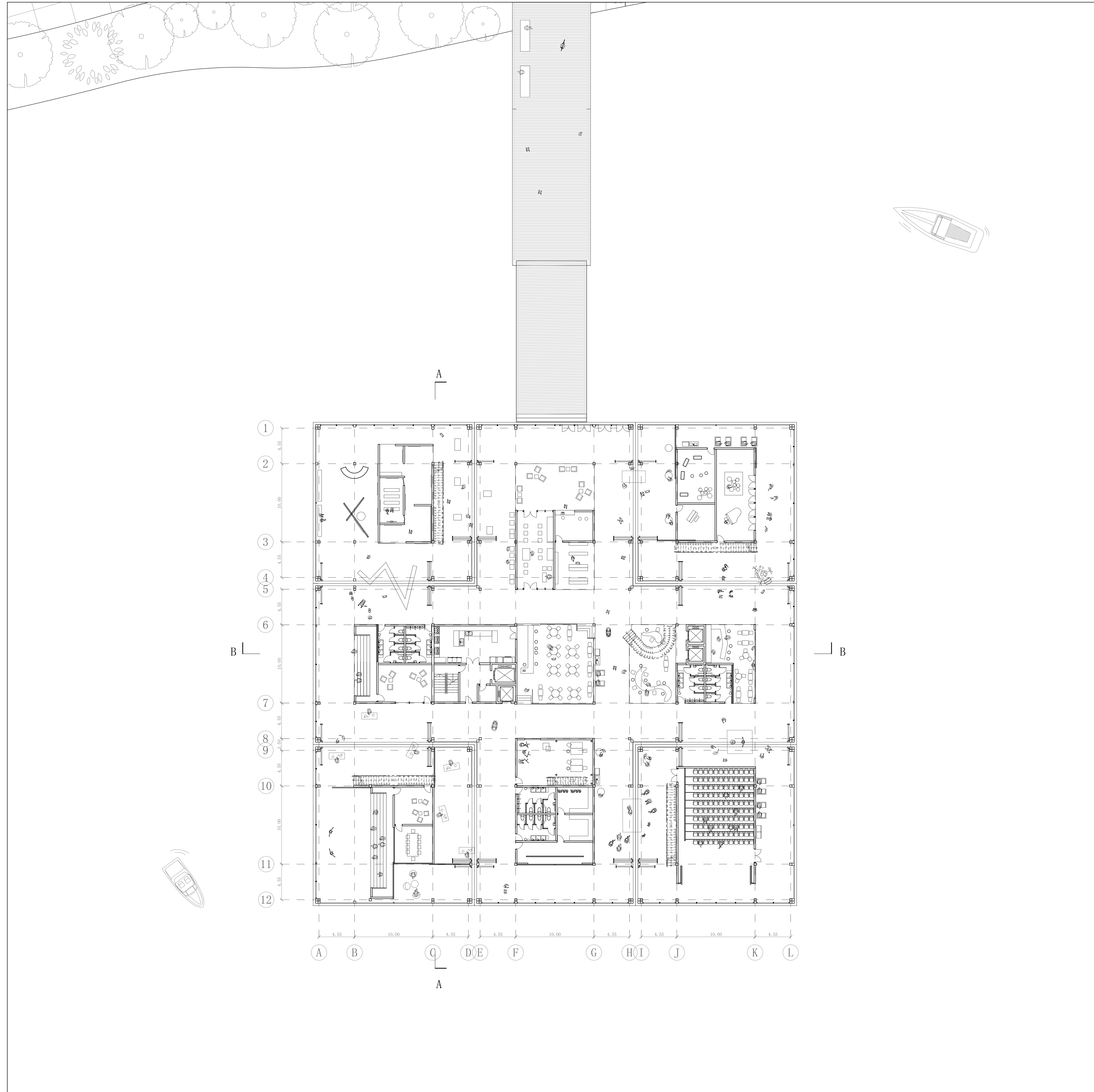
Ground floor Plan - Festival - 1:200
