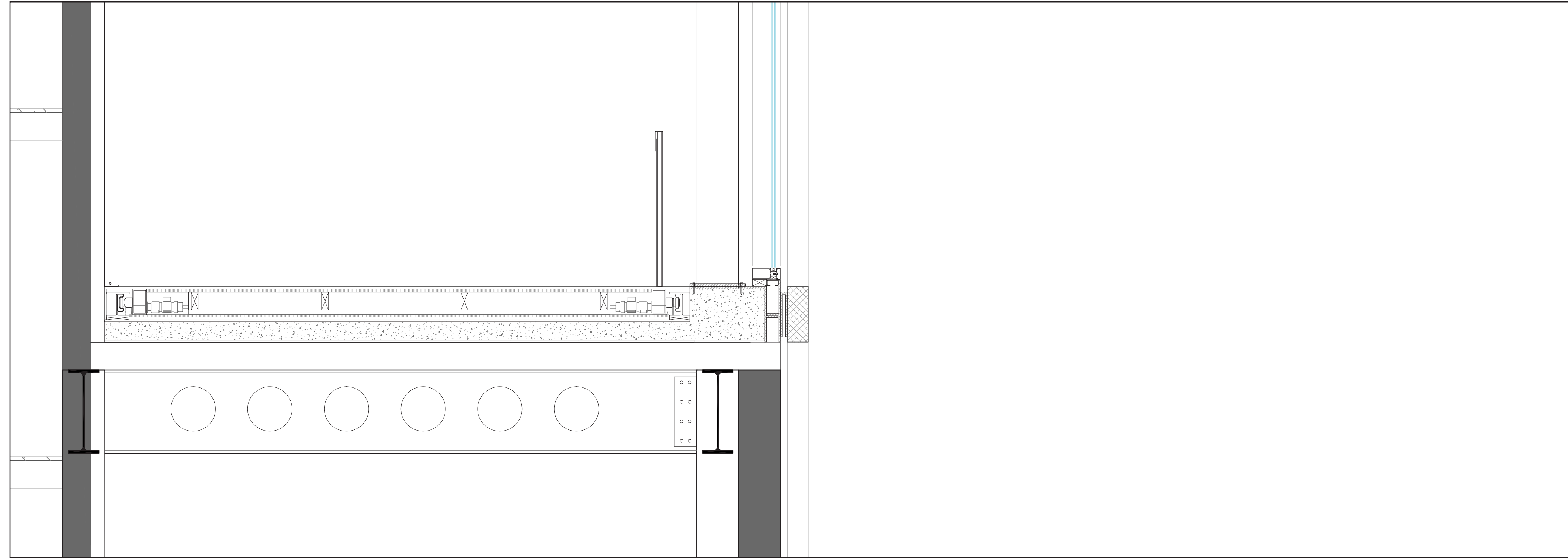
Section Fragment- Sliding - 1:20
