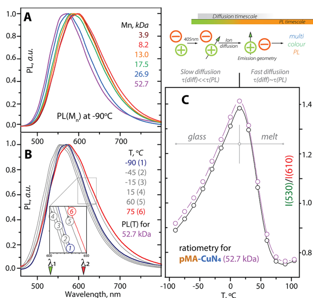
Figure 2. (A) Molecular weight dependence of emission spectra of end-labeled pMA in the glassy state at -90\text{ }^{\circ}\text{C} . (B) Thermochromism of end-labeled pMA with M_n = 52.7\text{ kDa} at selected temperatures with wavelengths used for ratiometry analysis indicated – \lambda_1 = 530\text{ nm} , \lambda_2 = 610\text{ nm} . (C) Ratiometric data for pMA with M_n = 52.7\text{ kDa} , duplicate measurements shown.
