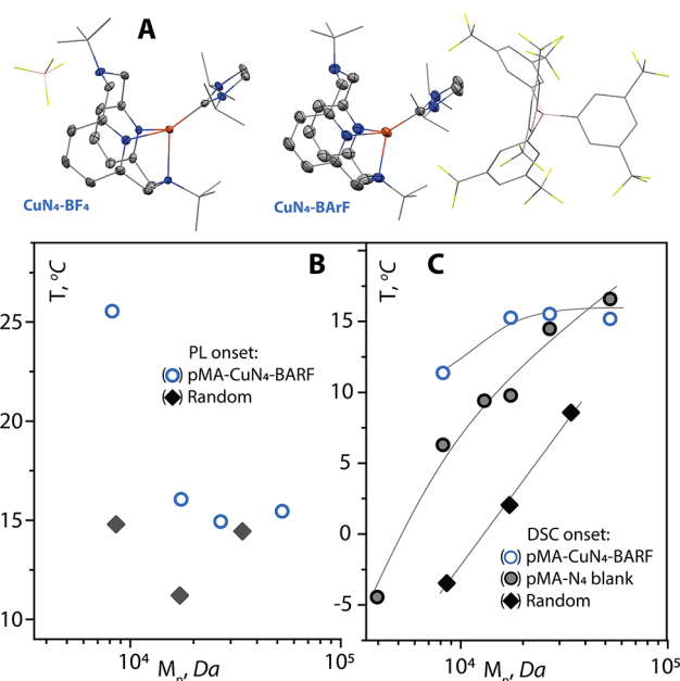
Figure 4. (A) Solid state structures of small molecule probes with tetrafluoroborate and BARF counterions indicating their different sizes; structures reproduced with permission from refs 29 and 30. (B) Comparison of PL data for end- and side-chain-labeled pMA. (C) DCS data for these polymers compared to the neutral pMA-N 4 reference.
