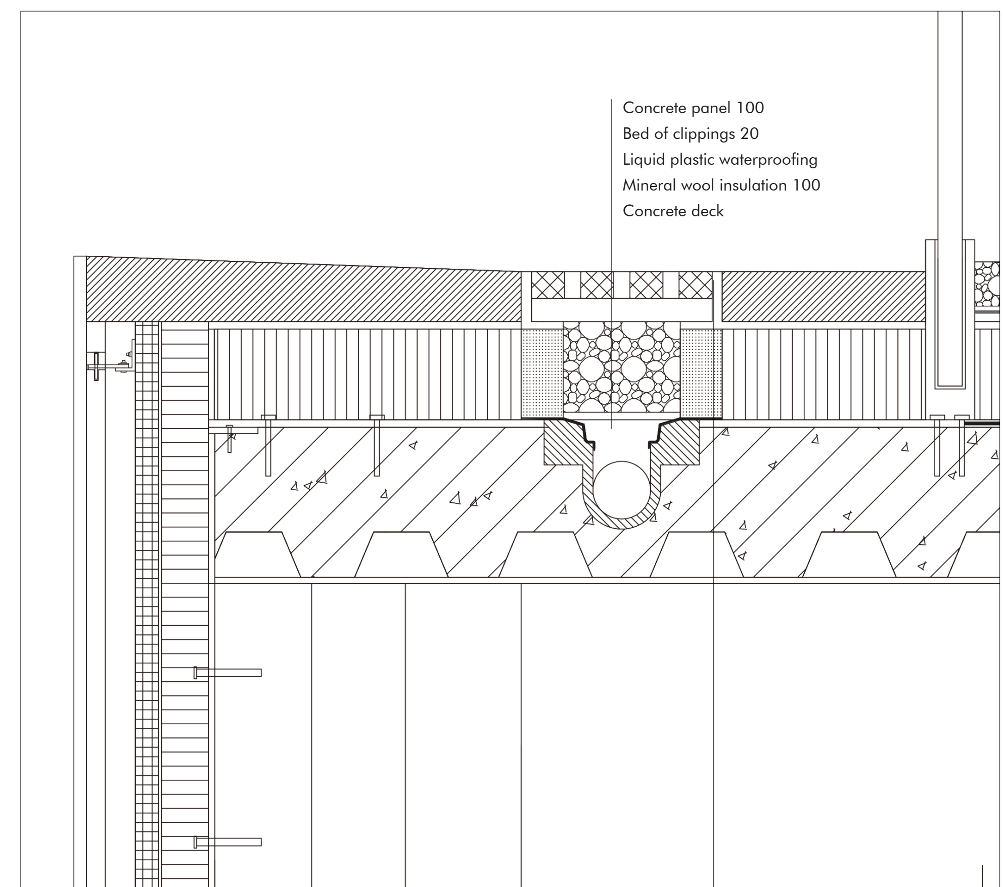
DETAIL B Roof gutter
