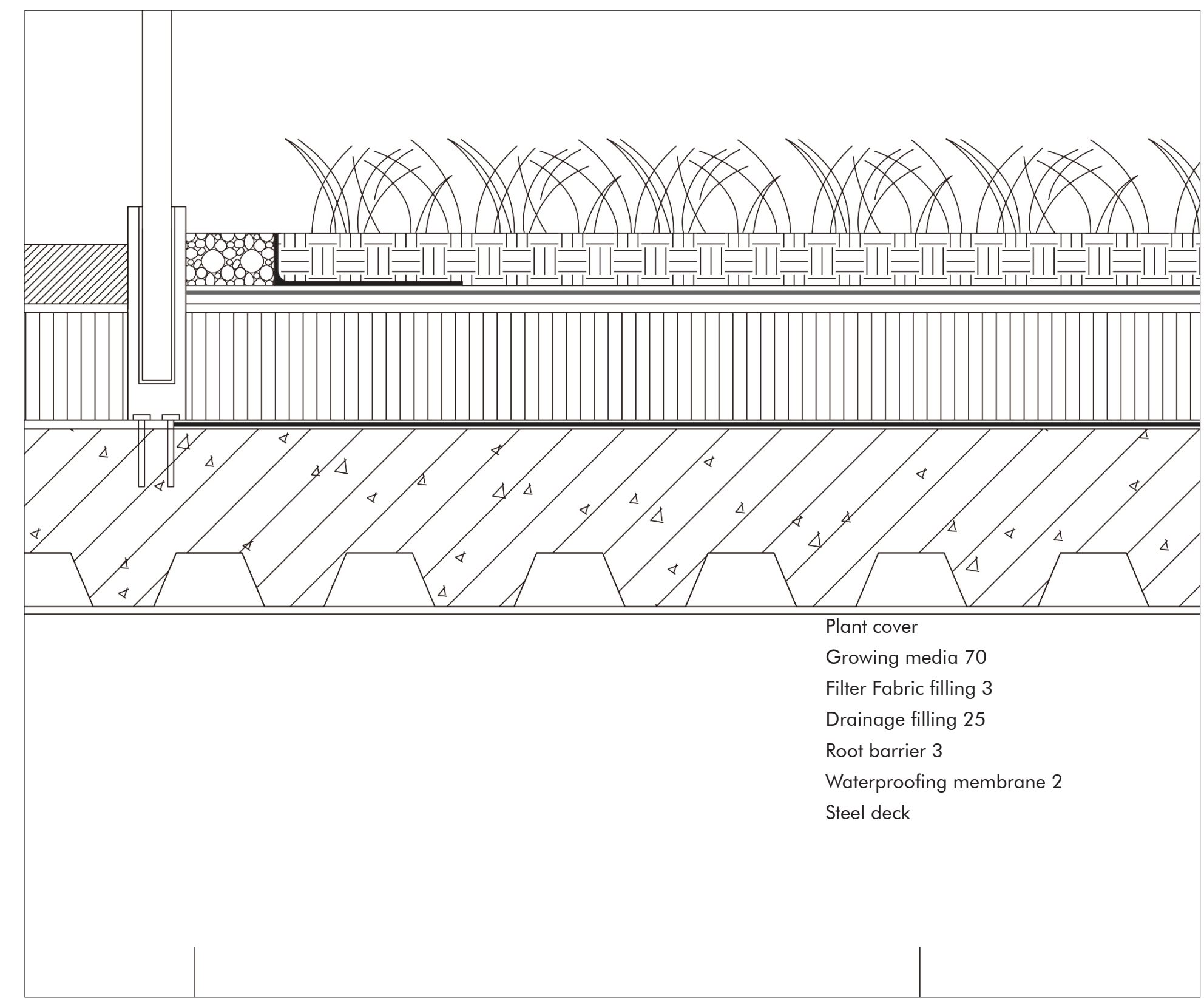
DETAIL B Roof gutter
