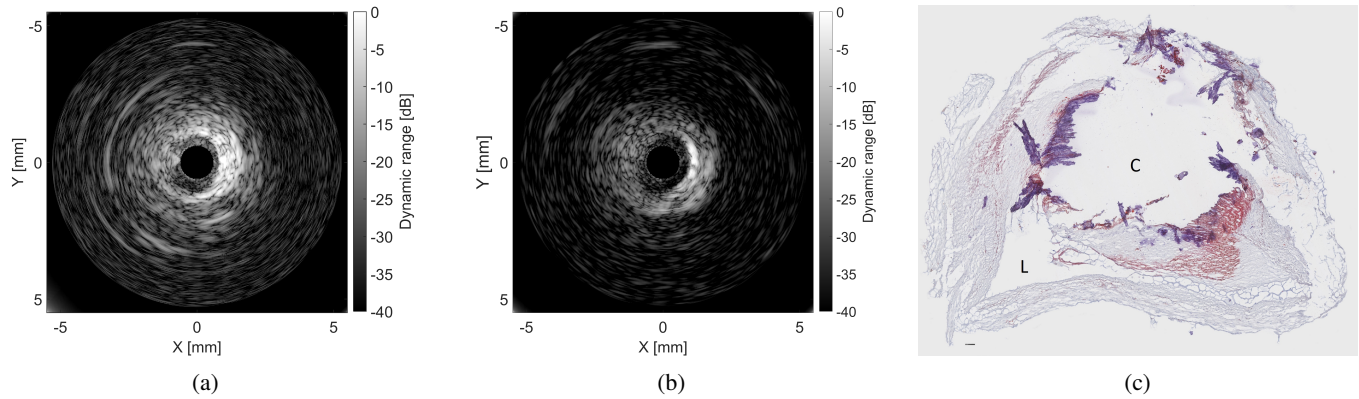
Fig. 8: Ex-vivo human coronary artery image reconstruction using the short pulse (a) and the chirp signal (b) by the rolled-up CMUT array. (c) is the histology image of the coronary sample. The scale bar is 100 \mu m
