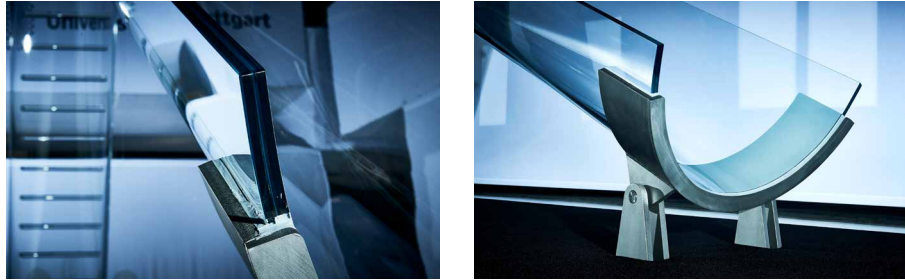
FIG. APP.A.13 Base detail with stainless steel shoe fixed to glass surface with structural silicone
