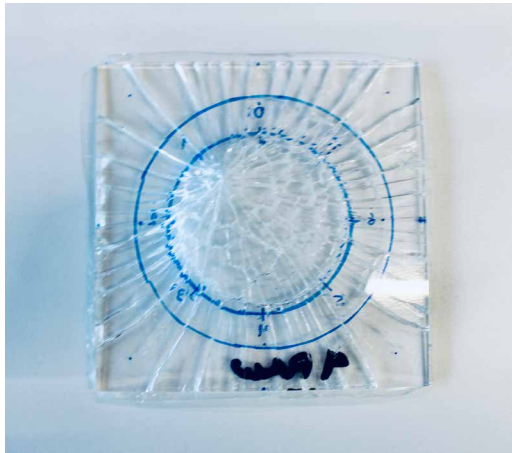
FIG. 6.44 Fracture Pattern specimen 4 AR
