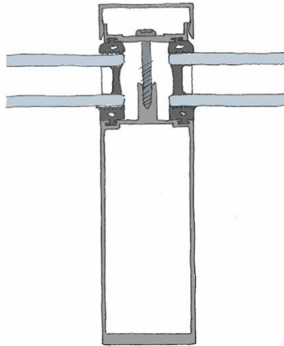
FIG. 4.19 Capped aluminium mullion, dry glazed
