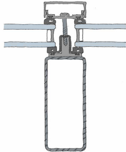
FIG. 4.20 Capped steel mullion, with aluminium CW mount, dry glazed
