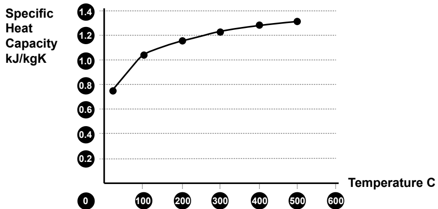
FIG. 5.11 Specific heat capacity of Borofloat 33
