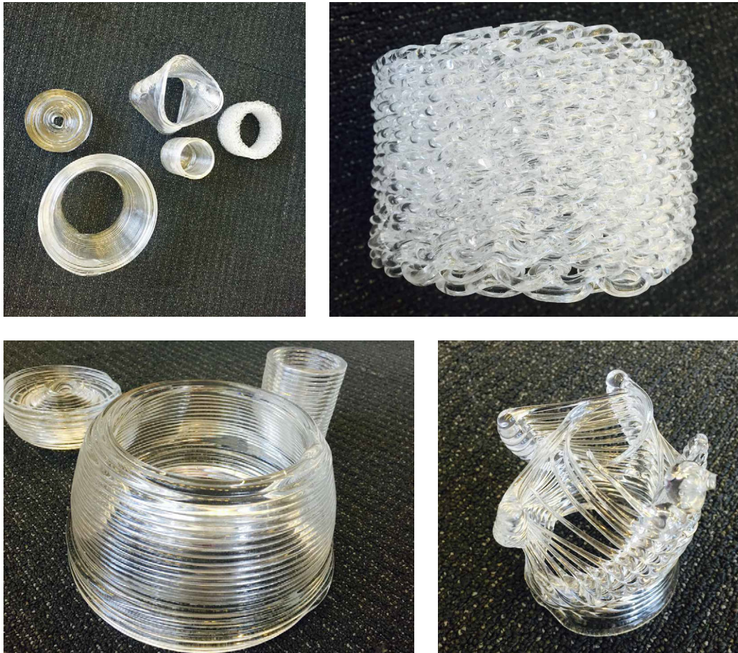
FIG. 5.6 Examples of objects created with 'G3DP' process at MIT
