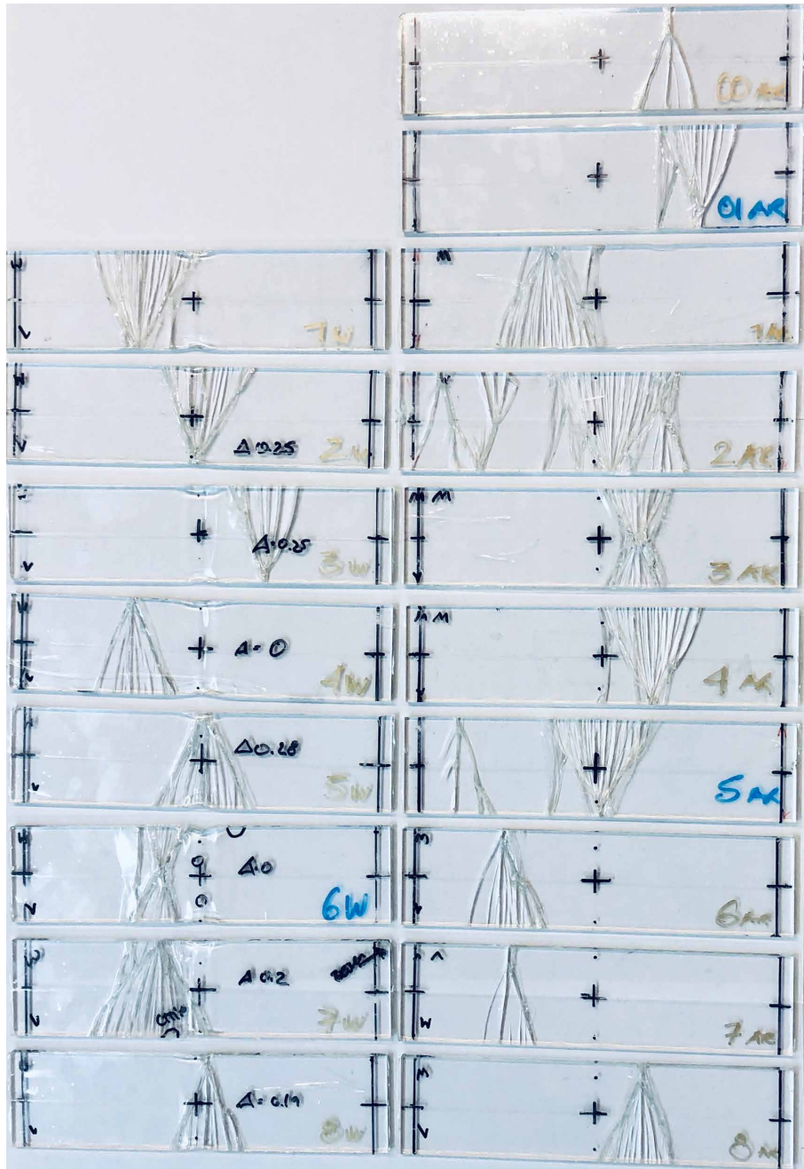
FIG. 6.38 Specimens after 4 point bending test. Left side heat bonded specimens (HB), right side as received (AR)
