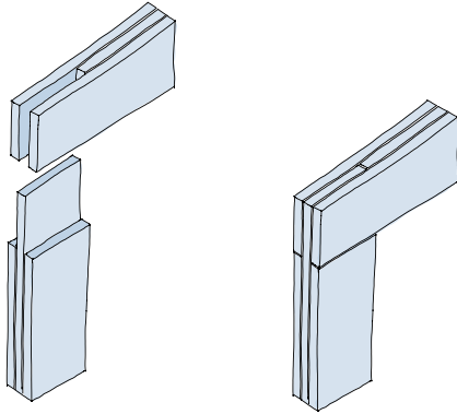
FIG. 4.52 Schematic mortise joint
