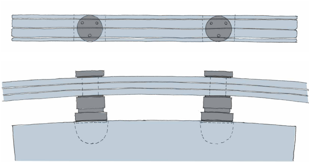
FIG. 4.41 Bolted stair point fitting, circular stair
