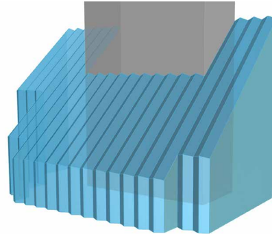
FIG. 7.12 Suggested replacement with a corrugated all-glass structure
