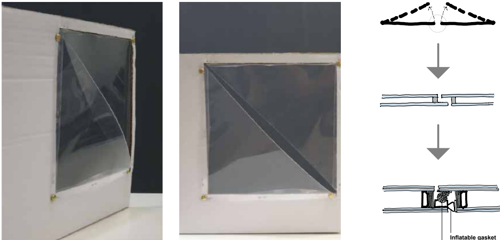
FIG. 7.39 Model of flexible ventilation panel
