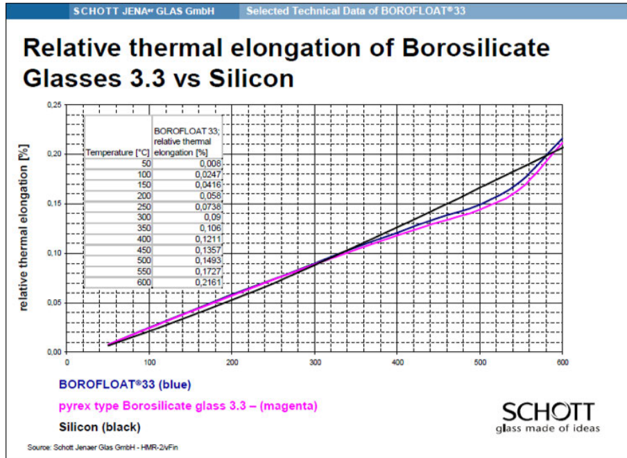
FIG. 5.12 Thermal elongation as obtained from (Schott ,2013)
