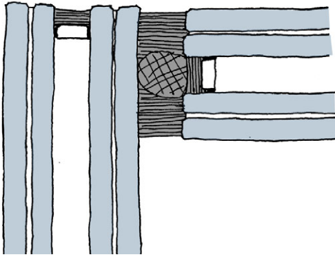
FIG. 4.62 Butt jointed corner
