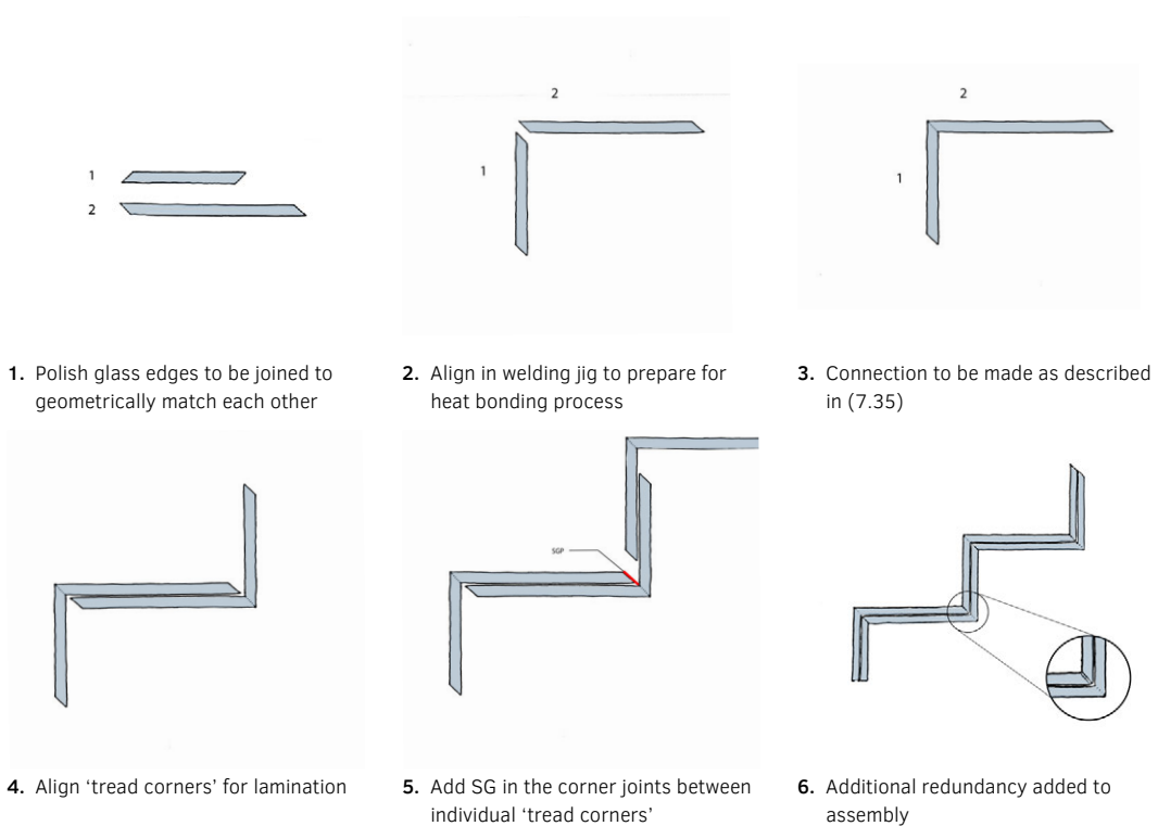
FIG. 7.2 Stair tread assembly
