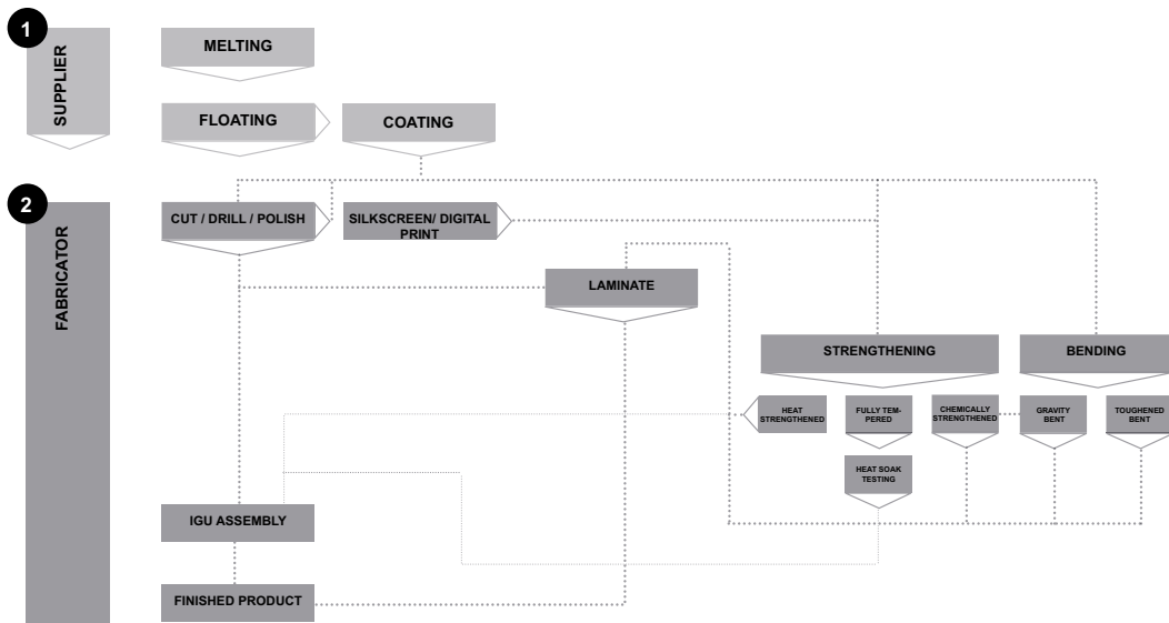
FIG. 2.13 Glass Processing
