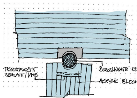
FIG. APP.A.20 Detail of central acrylic bearing block
