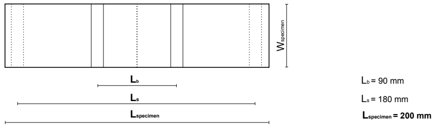
FIG. 6.35 Schematic of 4-point bending test set-up
