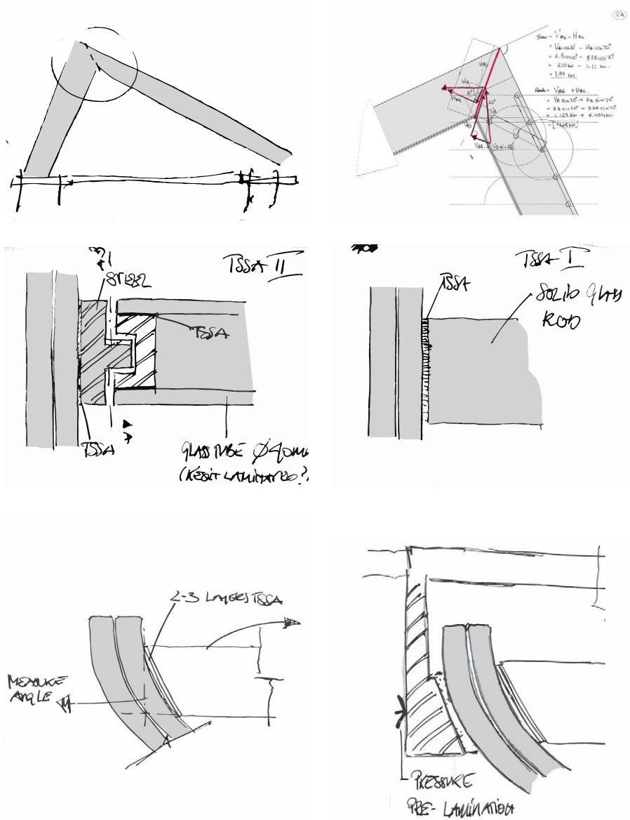
FIG. APP.A.12 Design and connection development
