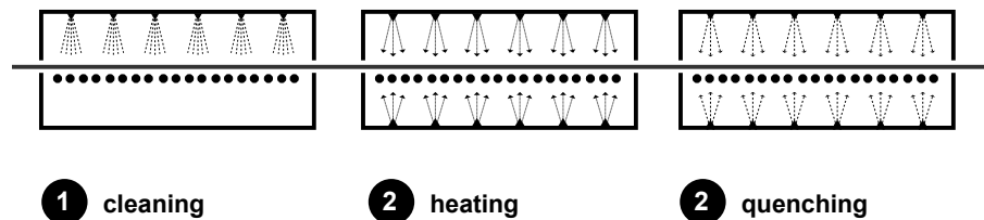
FIG. 2.15 Process of thermal tempering
