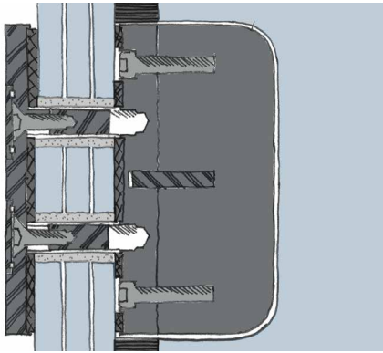
FIG. 4.48 Laminated fitting with clamping plate
