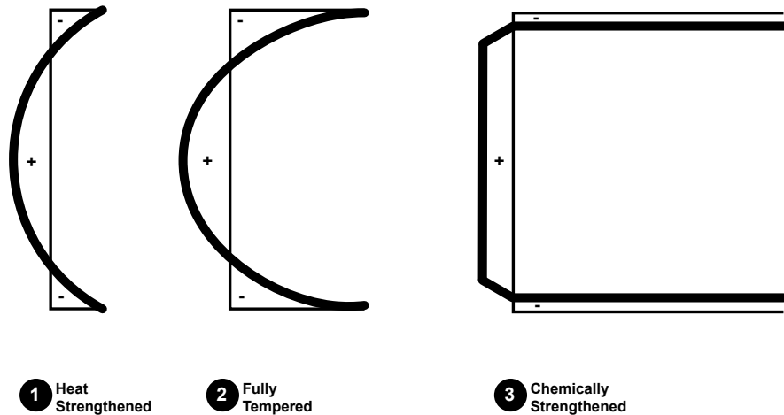
FIG. 2.16 Pattern of pre-stress through the material thickness for 1. Heat Strengthened (HS), 2. Fully Tempered (FT) and 3. Chemically Strengthened (CT) glass
