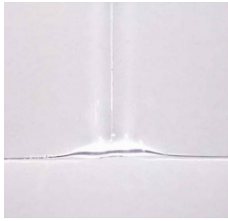
FIG. 6.27 Distorted edge due to temperature impact and fusing of the cut edge
