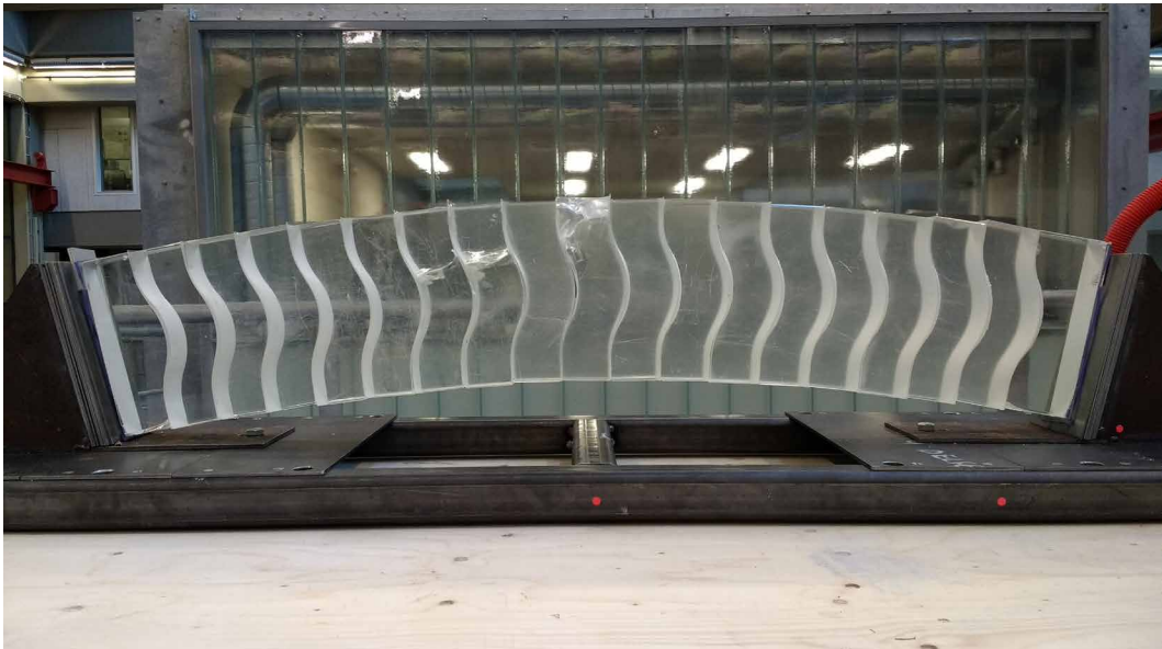
FIG. 3.71 Interlocking cast glass brick footbridge (Snijder, TU Delft)
