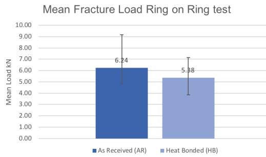
FIG. 6.43 Mean fracture Load for AR and HB specimens
