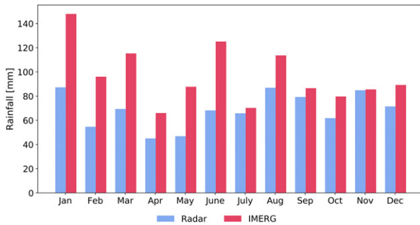
FIG. 1. Spatially averaged (time series calculated from IMERG native resolution over the entire period of evaluation) monthly rainfall accumulations according to the radar and IMERG datasets for the January 2015–December 2019 period.
