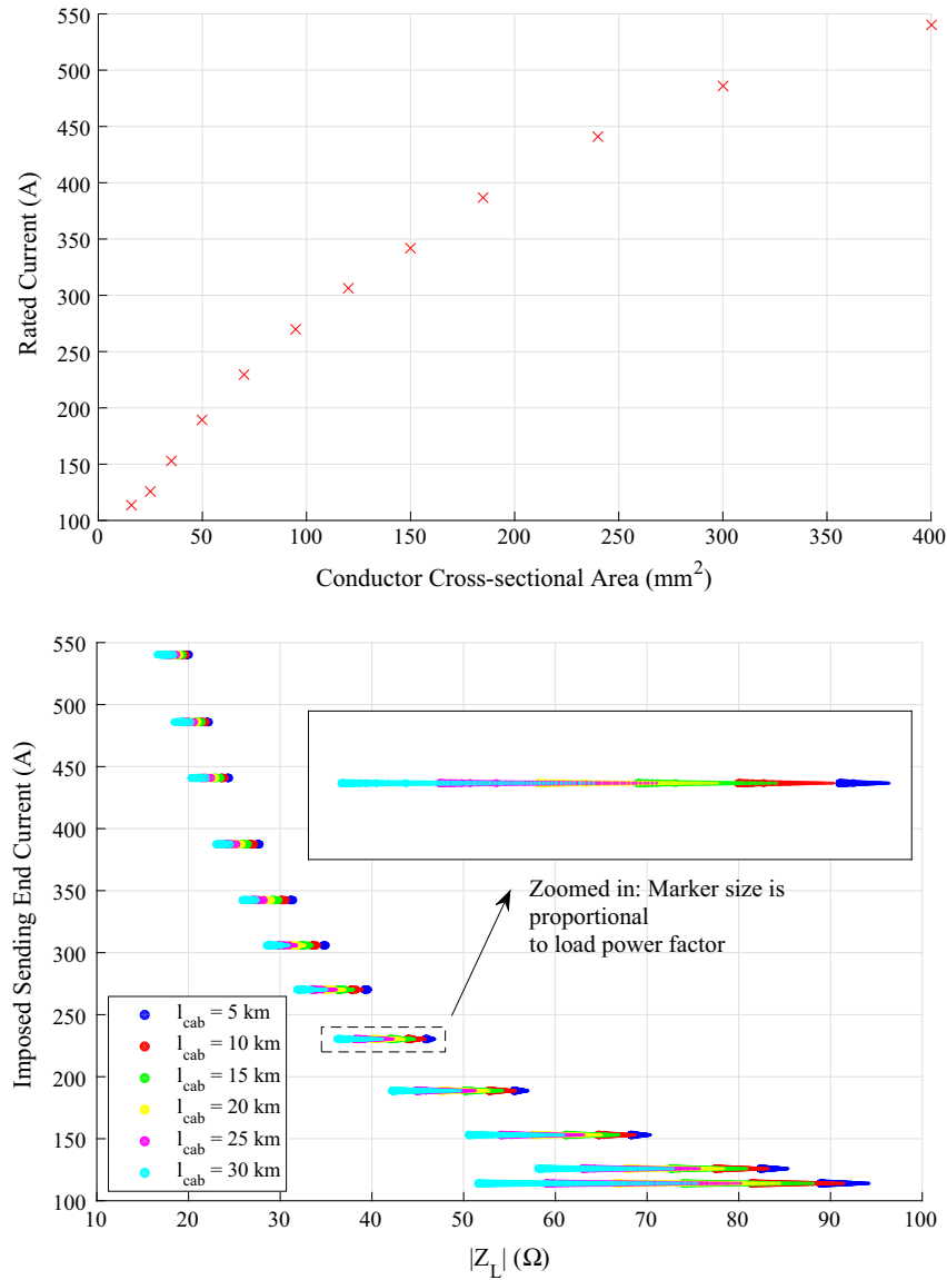
Fig. A.15. Computed load impedance magnitude with respect to imposed sending end cable current magnitude for varying cable lengths and load power factors.
