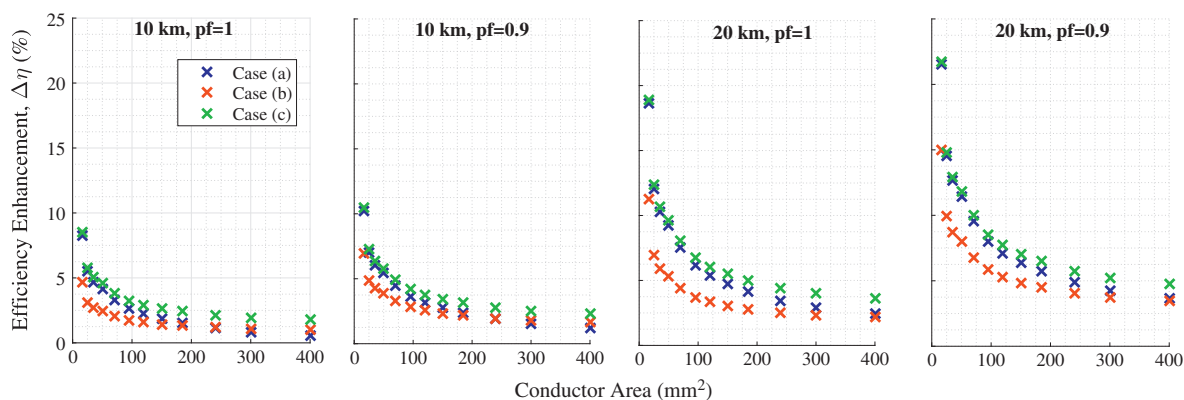
Fig. 9. Efficiency enhancement ( \Delta\eta ) for different cable cross-sectional areas, link lengths and load power factors.
