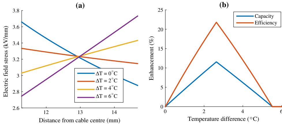
Fig. 12. Temperature dependence of (a) electric field stress on insulation of the cable (b) Transmission capacity and efficiency enhancement with proposed dynamic voltage rating.
