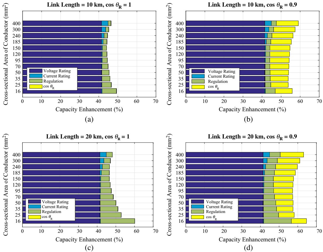
Fig. 8. Factor split of capacity enhancement by refurbishing 3 phase double circuit ac cable link to 3× bipolar dc link.
