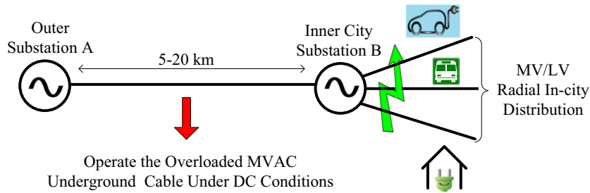
Fig. 1. Reconfigurable DC links for bulk power transmission into the city collection centre.
