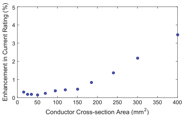
Fig. 3. Current rating enhancement in dc due to reduction of dielectric losses and absence of skin and magnetic proximity effects of ac operation.
