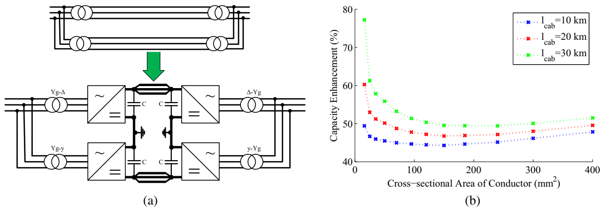
Fig. 6. Transmitted power capacity enhancement with conductor cross-sectional area for different cable lengths at unity load power factor for 3-phase double circuit ac to 3× bipolar dc links.
