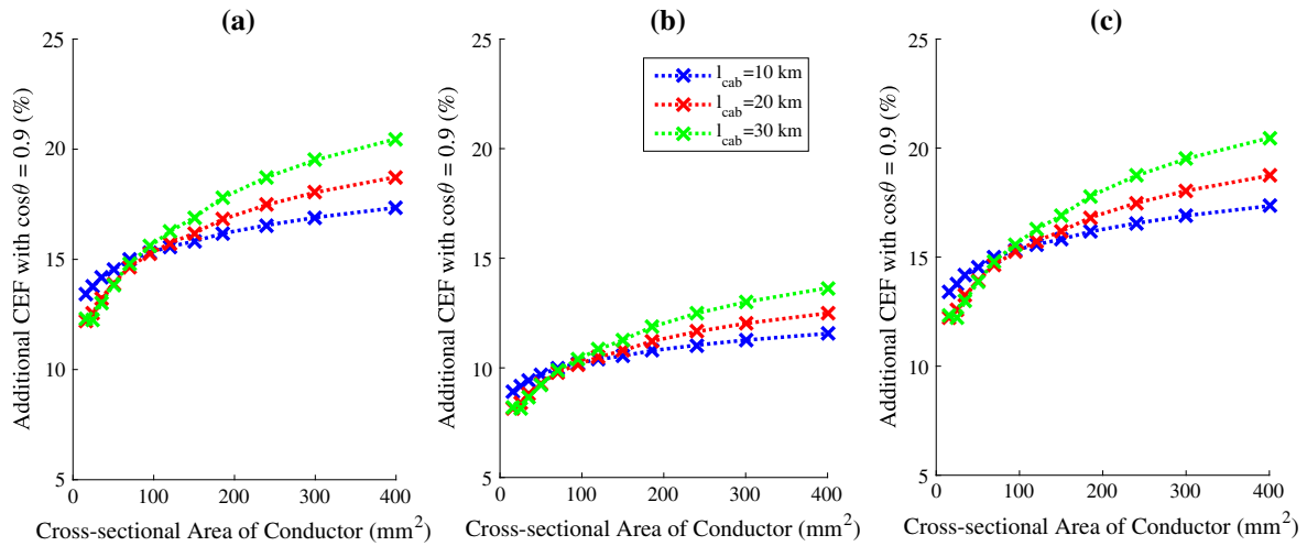
Fig. 7. Additional capacity enhancement for different conductor cross-sectional area for different cable lengths at 0.9 load power factor for (a) 3-phase single circuit ac to monopolar dc link with ground return (b) 3-phase single circuit ac to bipolar dc link (c) 3-phase double circuit ac to bipolar dc link.
