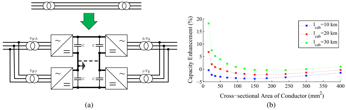
Fig. 5. Transmitted power capacity enhancement with conductor cross-sectional area for different cable lengths at unity load power factor for 3-phase single circuit ac to 1× bipolar dc links.
