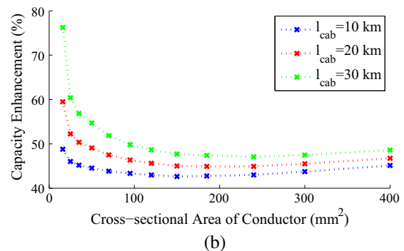
Fig. 4. Transmitted power capacity enhancement with conductor cross-sectional area for different cable lengths at unity load power factor for 3-phase single circuit ac to monopolar dc link with ground return.
