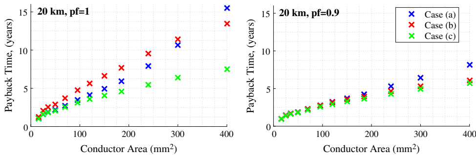
Fig. 11. Payback time based on energy savings due to system efficiency enhancement for different topologies.
