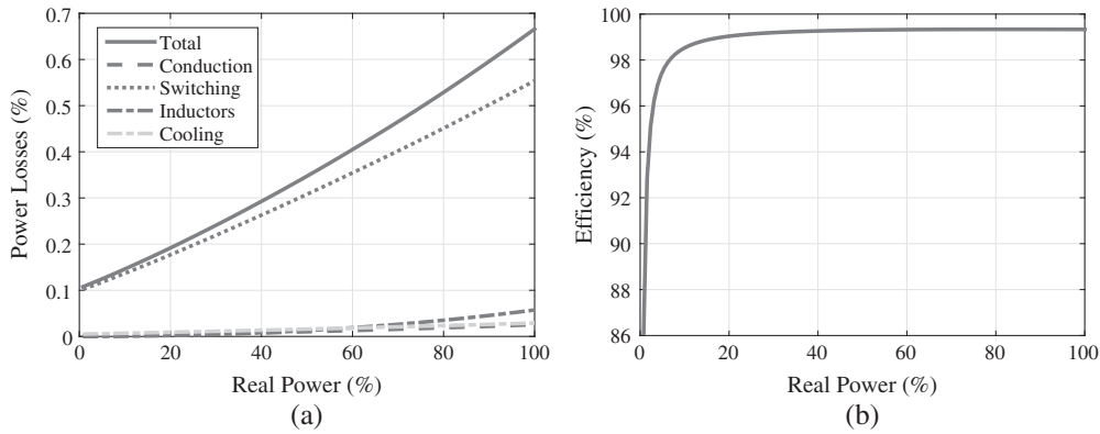
Fig. 10. Converter losses breakdown (a) and efficiency curve (b) for 300 mm 2 cable conductor area and converter power 7.7 MW.
