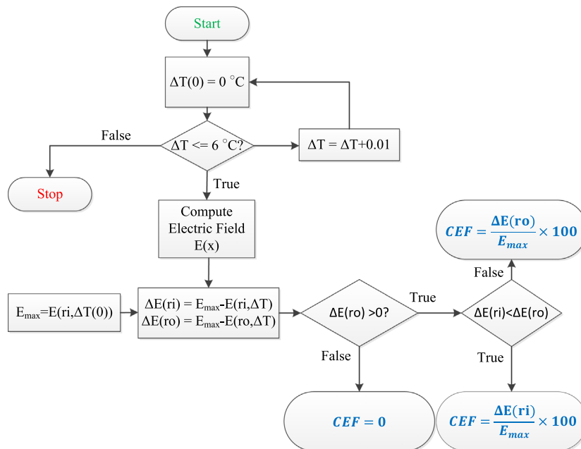
Fig. 13. Algorithm flowchart for computing the capacity enhancement factor (CEF).
