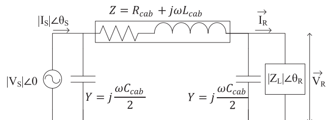
Fig. A.14. Equivalent circuit for underground MVAC distribution cable link.
