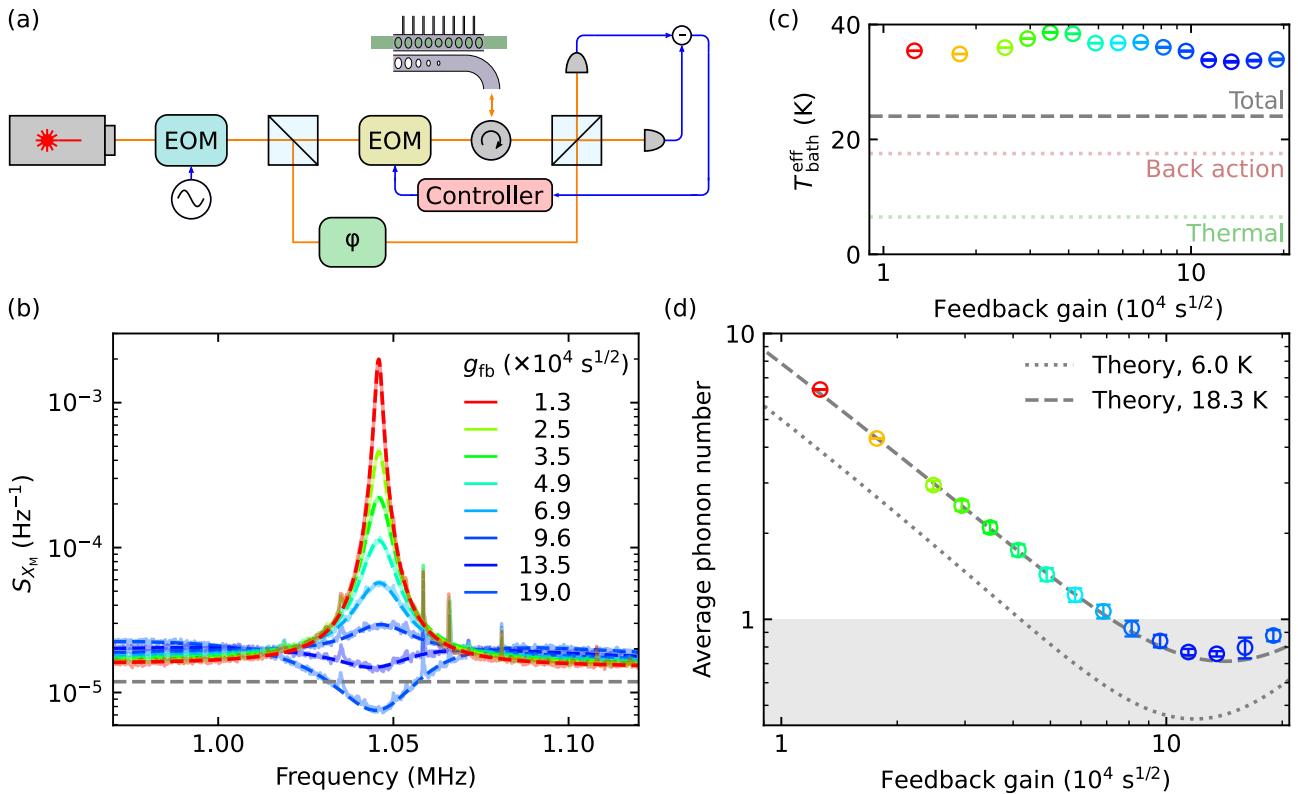
Fig. 3 | Feedback cooling without sideband-asymmetry measurement. a Feedback cooling setup. A single, slightly red-detuned laser is used to perform the measurement. b A measured spectrum, converted into the displacement quadrature quanta, of the mechanical resonator, at different feedback strength. The fits (dashed lines) are used to extract the system parameters and the phonon
