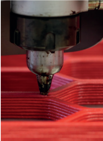
Fig. 7A: 3D-printing process of the polymer core
