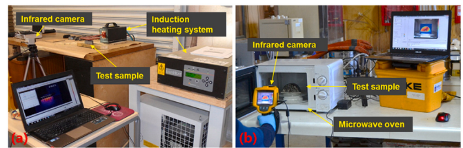
Fig. 4. Thermal induced healing technology: (a) electromagnetic induction heating healing and (b) microwave induction heating healing (Norambuena-Contreras and García, 2016).
