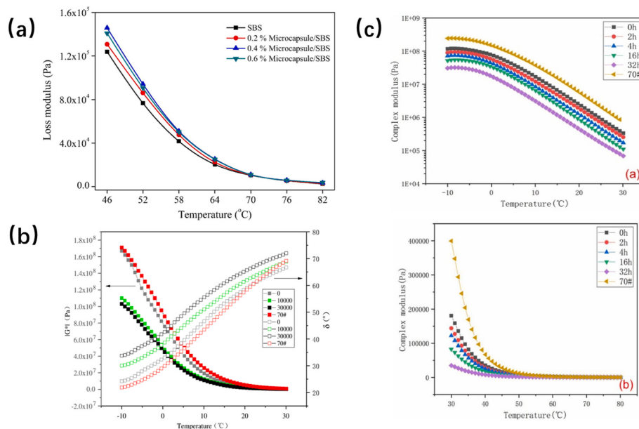
Fig. 15. (a) The loss modulus of SBS modified asphalt binder containing different dosage of UF microcapsules after healing accomplish (Li et al., 2020), (b) the complex modulus and phase angle of asphalt binder extracted from asphalt mixtures with Ca-alginate capsules after different cycles of loading (Bao et al., 2021), (c) the complex modulus of asphalt binder extracted from asphalt mixtures with Ca-alginate capsules after different time of cyclic loading via wheel tracking test (Rao et al., 2021).
