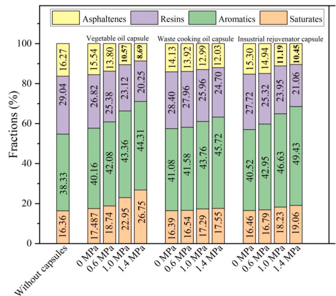
Fig. 16. The SARA component variation of the extracted asphalt binder after 10000 cycles of compression loading at 0.6 MPa, 1.0 MPa and 1.4 MPa respectively (Wang, H. et al., 2022b).
