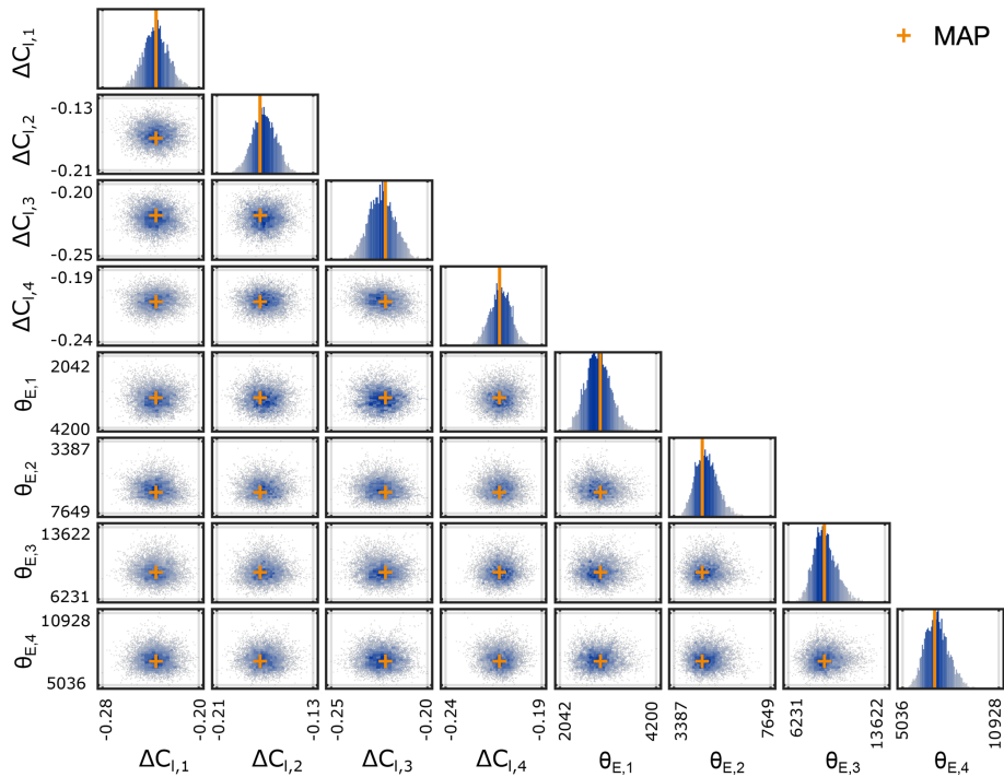
Figure 8. Samples of the posterior distribution of model parameters \theta_M = (\Delta C_{l,1}, \dots, \Delta C_{l,4}) and discrepancy parameters \theta_E = (\theta_{E,1}, \dots, \theta_{E,4}) for the DANAERO test case with 200 measurements. The orange crosses correspond to the MAP estimates.
