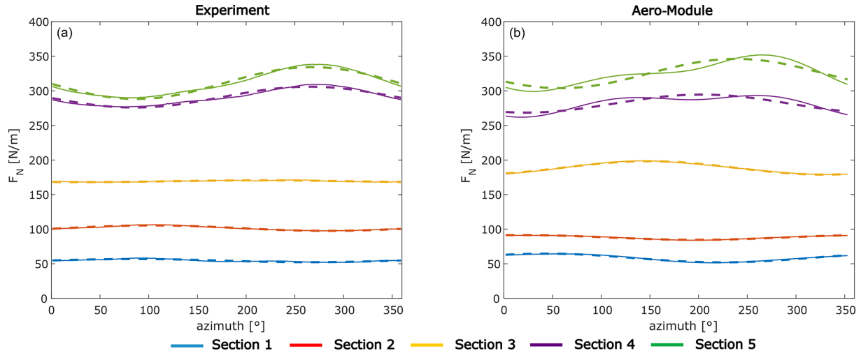
Figure 5. Representation of measurements (a, solid lines) and Aero-Module output (b, solid lines) using three Fourier coefficients (dashed) at different radial sections, for scenario \mathcal{S}_1 (run 935) of the New MEXICO experiment (last revolution shown).
