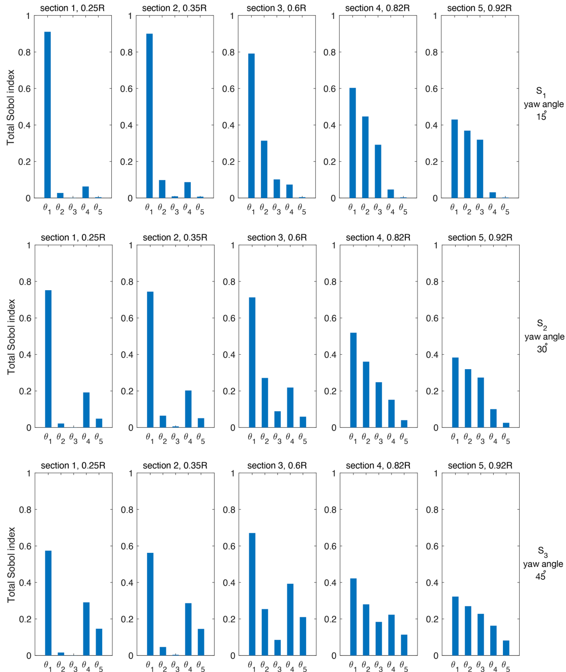
Figure 10. Sensitivity analysis for three different operating conditions: \mathcal{S}_1 (top), \mathcal{S}_2 (middle), and \mathcal{S}_3 (bottom). Here \theta_M = (\theta_1, \theta_2, \theta_3, \theta_4, \theta_5) = (AM_{11}, AM_{12}, AM_{13}, AM_{14}, AM_{15}) .
