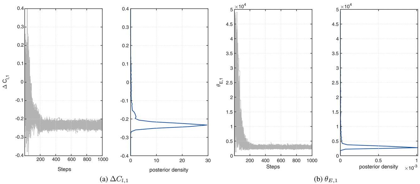
Figure B4. Examples of MCMC chains and resulting posterior for model parameter \Delta C_{l,1} and hyperparameter \theta_{E,1} , using 200 measurement points. For the results reported in Sect. 5.1, the first 50 % of the chains is discarded (so-called burn-in).
