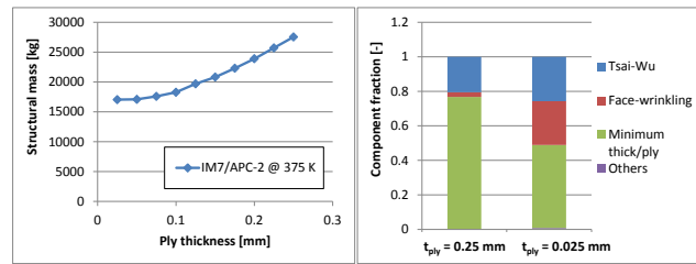
FIGURE 13. Computed structural masses for different ply thicknesses (left); sizing criteria for two selected ply thicknesses (right)
