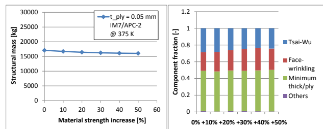
FIGURE 14. Computed structural masses as a function of material transverse and shear strength increase (left); sizing criteria (right)
