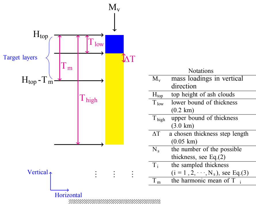
Figure 2. Illustration of the satellite observational operator (SOO).
