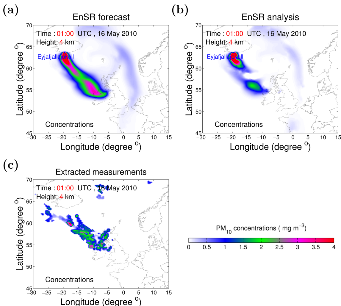
Figure 4. Examination of EnSR effect when assimilating SEVIRI-extracted ash concentrations at 01:00 UTC 16 May 2010. (a) EnSR forecast (ensemble mean) of PM 10 concentrations. (b) EnSR analysis (ensemble mean) of PM 10 concentrations. (c) Extracted measurements of PM 10 concentrations from the SOO. (a), (b), (c) are illustrated at a height of 4 km.
