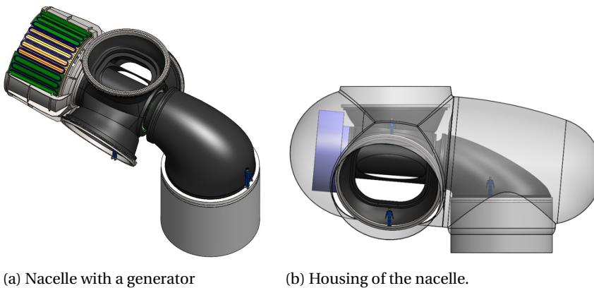
Figure 2.30: INNWIND.EU nacelle concept using a kingpin for 10-20 MW direct-drive wind turbines. The generator is located in front of the hub. [11]
