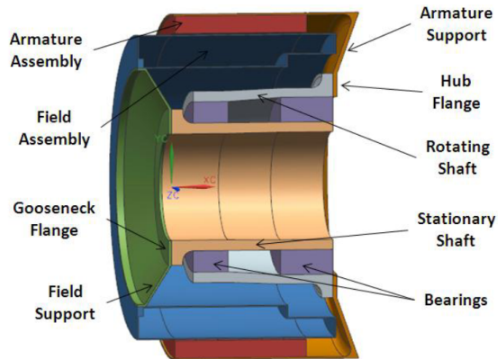
Figure 2.27: Integration concept by General Electric for a 10 MW direct-drive LTS generator. [20]
