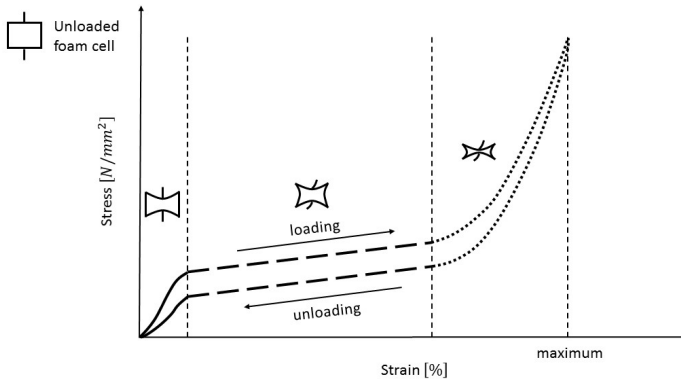
Figure 2.8: Hysteresis-Diagram
