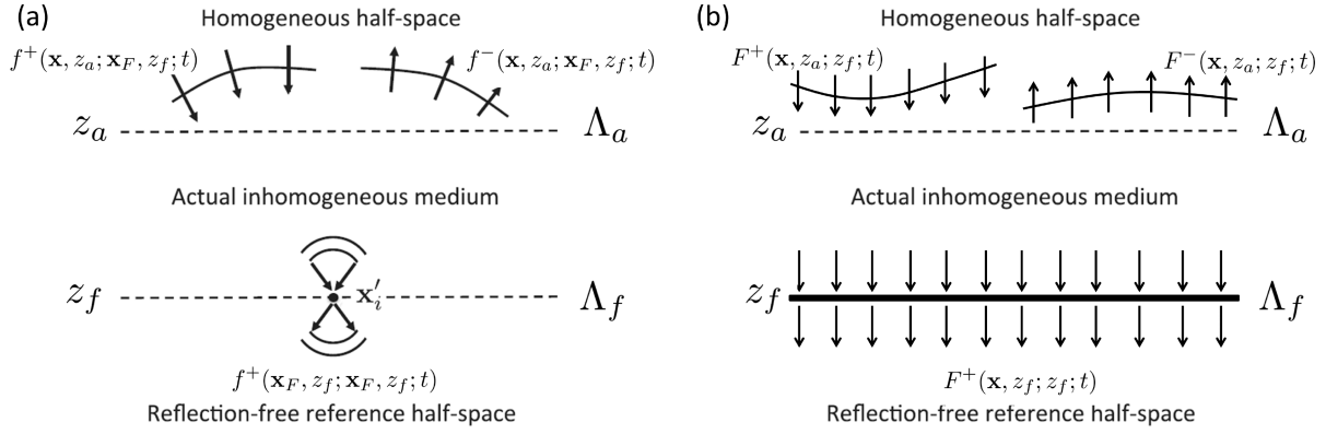
Figure 1. Down- and upgoing components of the focusing functions of the 3-D wave equation in a reference configuration. (a) Standard space–time focusing function f_i , leading to point-source responses (Green’s functions). (b) Time focusing function F_1 , leading to areal-source responses.
