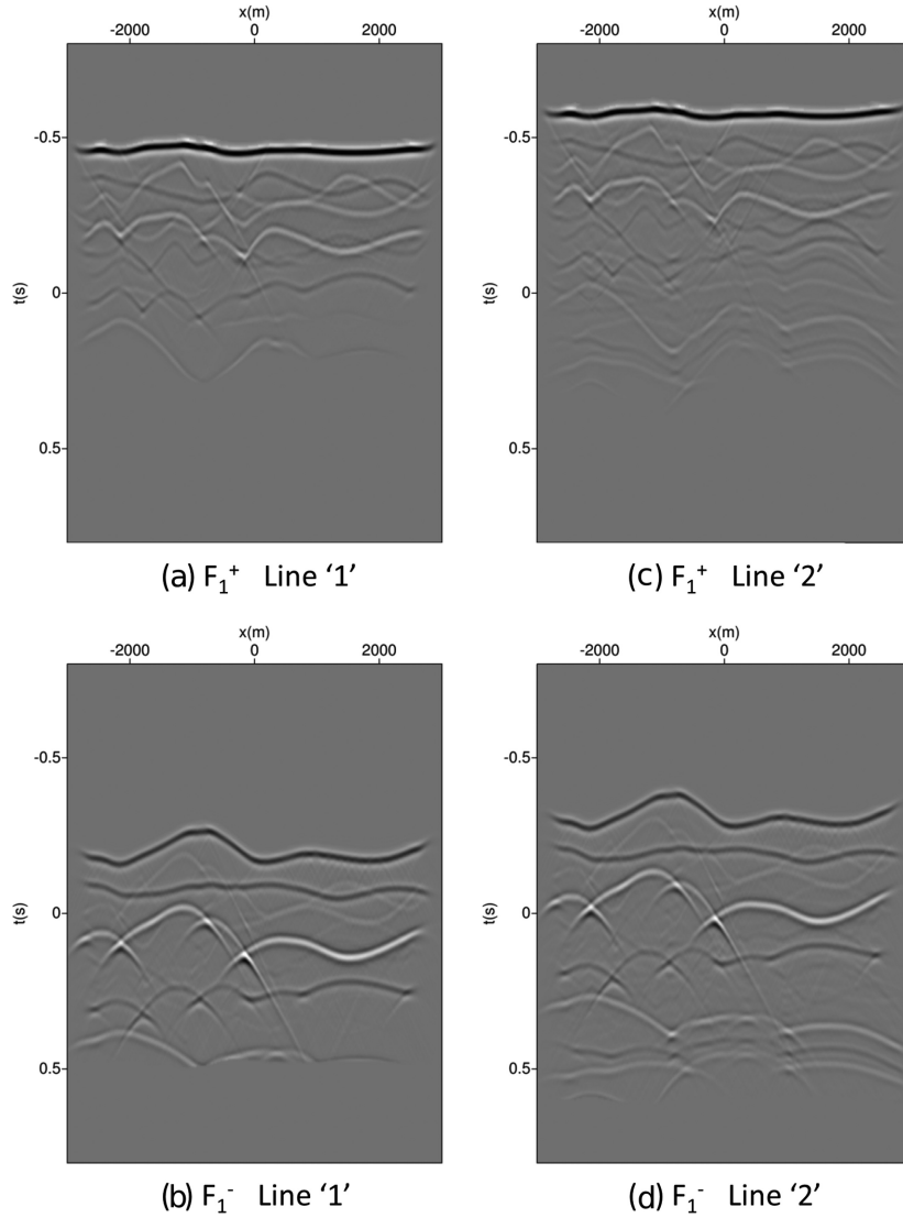
Figure 3. (a) Downgoing component of the focusing function F_1 associated with F_{1d^+} being first arrival of \int_{L_1} d^2 \mathbf{x} g^+(\mathbf{x}, z_f; t; \mathbf{x}', z_a; 0) . (b) Upgoing component of the focusing function F_1 associated with F_{1d^+} being the first arrival of \int_{L_1} d^2 \mathbf{x} g^+(\mathbf{x}, z_f; t; \mathbf{x}', z_a; 0) . (c and d) As for panels (a) and (b), but for F_{1d^-} associated with the first arrival of \int_{L_2} d^2 \mathbf{x} g^+(\mathbf{x}, z_f; t; \mathbf{x}', z_a; 0) .
