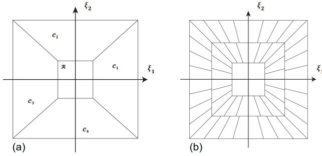
Figure A2. The cone-adapted continuous shearlet system. (a) Bias in directions is handled by dividing the frequency plane into four cones \mathcal{C}_1, \mathcal{C}_2, \mathcal{C}_3, \mathcal{C}_4 , and a square low-frequency box region in the centre \mathcal{R} . (b) Trapezoidal-shaped wedge tiling of the frequency-induced domain induced by the shearlet transform (modified after Kutyniok and Labate, 2012).
