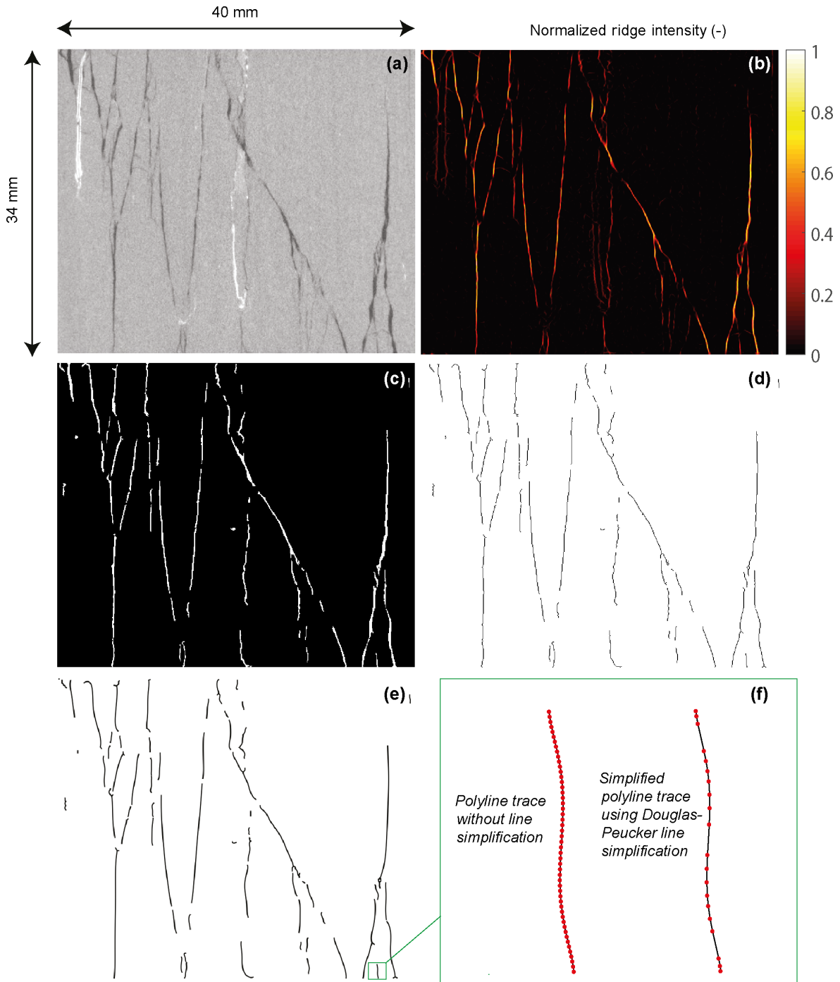
Figure 2. Illustration of the steps involved in the automatic fracture extraction using a 40 \times 34 mm fractured shale core image. (a) CT scan core image from Dwarkasing (2016). (b) Normalized ridge ensemble. (c) Segmentation applied to the ridge ensemble. (d) Skeletonization applied to the segmented ridge. (e) Vectorized polylines fitted to the skeletonized clusters. (f) Effect of line simplification applied to a single vectorized segment.
