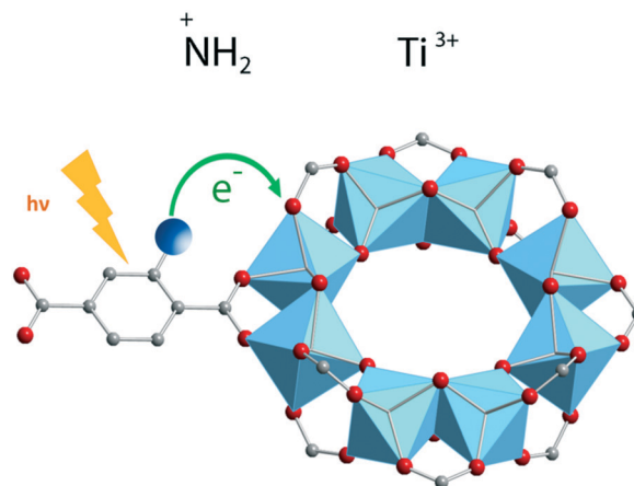
Fig. 6 Ligand-to-metal charge transfer (LMCT) and location of photogenerated charges in \text{NH}_2\text{-MIL-125}(\text{Ti}) . 52 Reproduced with permission from Wiley.
