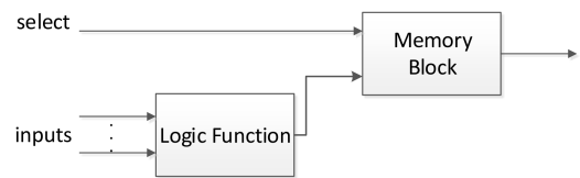
FIGURE 17. Generic QCA circuit with memory.
