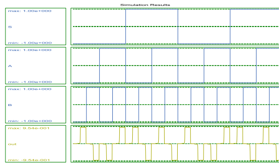
FIGURE 11. Fig. 10 circuit simulation results.
