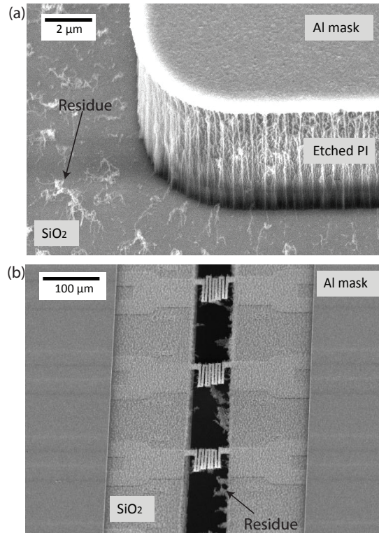
Figure 2: (a) Residue covered SiO 2 surface after reactive ion etch of PI with Al metal as the mask. (b) Free standing metal interconnect structures on the same wafer covered with “fur-like” residues after the PI etch.
