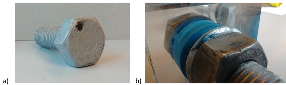
Fig. 1. (a) M20 × 50 mm ISO4017 8.8U bolt with an injection channel in the bolt head. (b) Resin-injected bolted connection with transparent plate package. The resin (blue) is injected through a hole in the bolt head. (For interpretation of the references to colour in this figure legend, the reader is referred to the web version of this article.)
