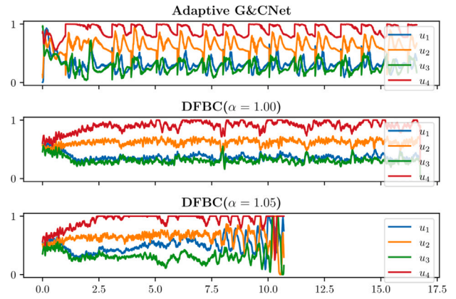
Fig. 12. Comparison of the normalized RPM commands of the Adaptive G&CNet compared to the fastest DFBC flight at \alpha = 1.00 and the failed flight at \alpha = 1.05 .
