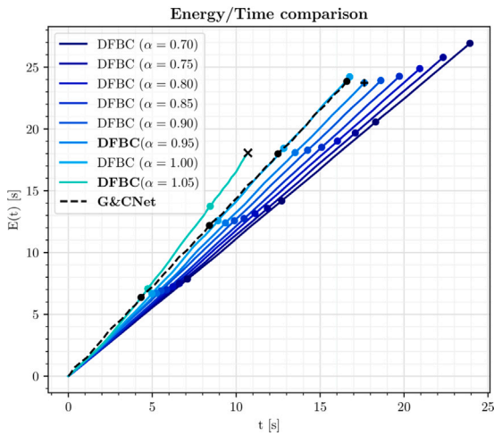
Fig. 10. Energy plotted over time during 4 laps of the 3 \times 4 m track with the added weight. The points in time where a lap is completed are represented by a dot. The DFBC method that uses the least energy is marked with a “+”. The flight that crashes is marked with an “x”.
