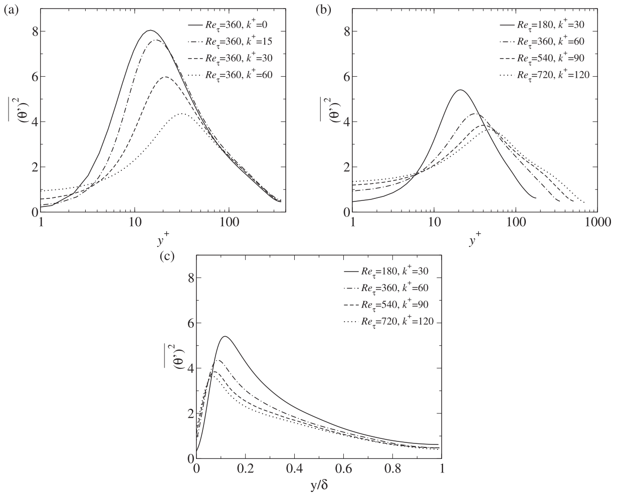
Fig. 8. (a) \overline{(\theta')^2} normalized by T_\tau^2 for Re_\tau = 360 . (b) \overline{(\theta')^2} for k/\delta = 1/6 . (c) Same as (b), except that \overline{(\theta')^2} is plotted against y/\delta .
