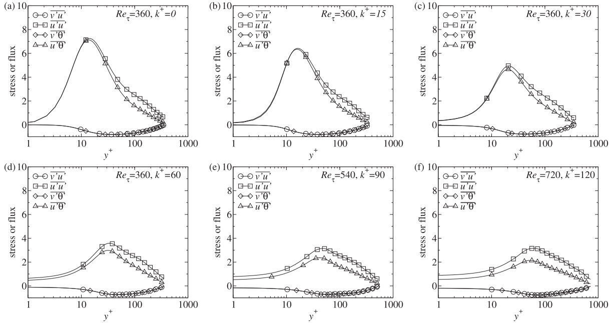
Fig. 9. The wall normal Reynolds stress ( \overline{v'u'} , normalized by u_\tau^2 ) and heat flux ( \overline{v'\theta'} , normalized by u_\tau T_\tau ) for cases with different k^+ . In the top row (a/b/c), Re_\tau = 360 , while in the bottom row (d/e/f), k/\delta = 1/6 .
