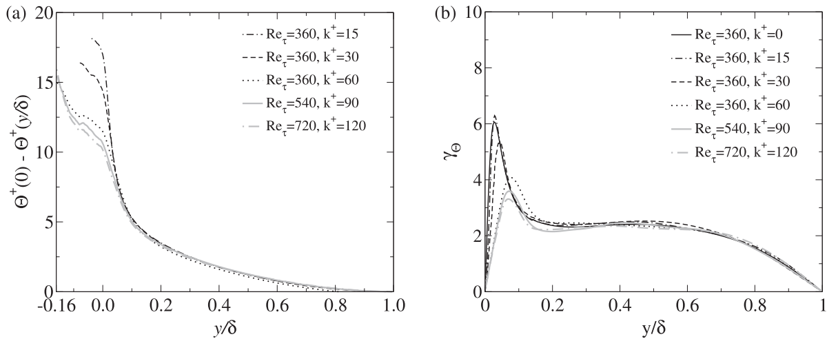
Fig. 6. (a) Temperature defect profiles. (b) Temperature diagnostic function.
