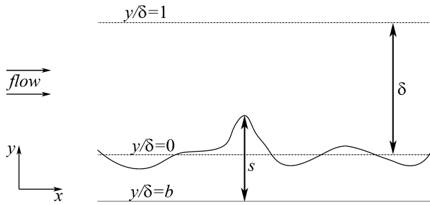
Fig. 2. Schematic of half the computational domain. \delta is the mean channel half height measured from the surface to the centreline of the channel. s is the surface height measured from the lowest point of the computational domain to the surface. b is the lowest point in the domain and equals -0.16 ( 1 \times 1 surface), -0.08 ( 2 \times 2 surface) and -0.04 ( 4 \times 4 surface).
