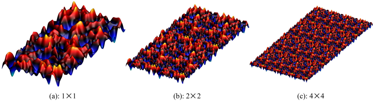
Fig. 1. Height maps of three different rough walls. (a) The filtered result of a grit-blasted surface. (b) a 2 \times 2 tiled version of the first surface. (c) a 4 \times 4 tiled version of the first surface.
