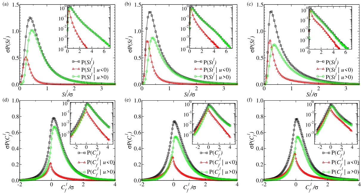
Fig. 16. Probability density functions of the local Stanton numbers St^l (top row) and skin friction coefficients C_f^l (bottom row) for the cases k^+ = 15 (a/d), k^+ = 30 (b/e) and k^+ = 60 (c/f). Re = 360 . \sigma denotes the standard deviation of P(St^l) .
