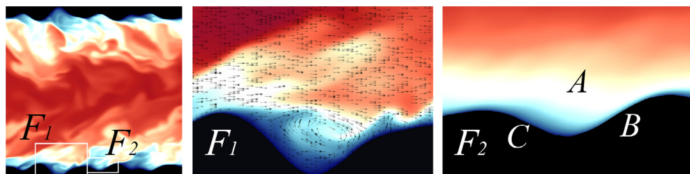
Fig. 12. Left: part of the simulated channel with instantaneous temperature contours. Middle: instantaneous velocity vectors and close to a recirculation zone from frame F_1 . Velocity vectors are not to scale. Right: time averaged temperature contours close to a recirculation zone from frame F_2 .
