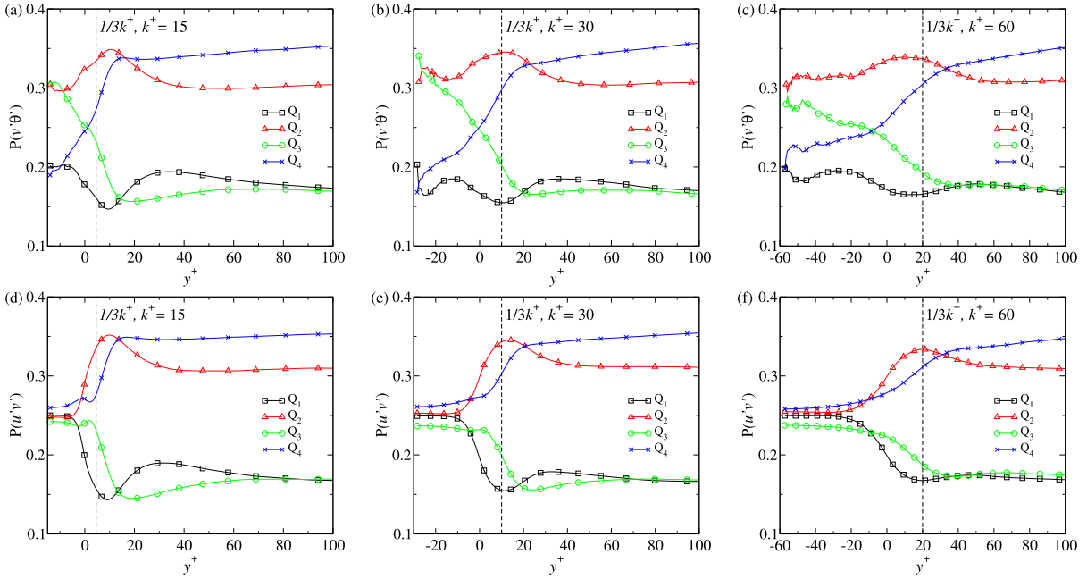
Fig. 14. Quadrant probabilities of the Reynolds shear stress v'u' and the turbulent heat flux v'\theta' for Re_\tau = 360, k^+ = 15 (a/d) k^+ = 30 (b/e) and k^+ = 60 (c/f).
