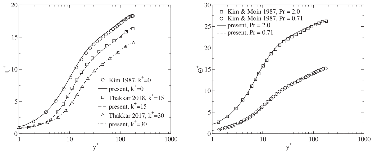
Fig. 4. Comparison of mean velocity and temperature profiles for k^+ = 0, 15 and 30 at Re_{\tau} = 180 with results from Busse et al. [7], Thakkar et al. [36], Kim et al. [20] and Kim and Moin [19].
