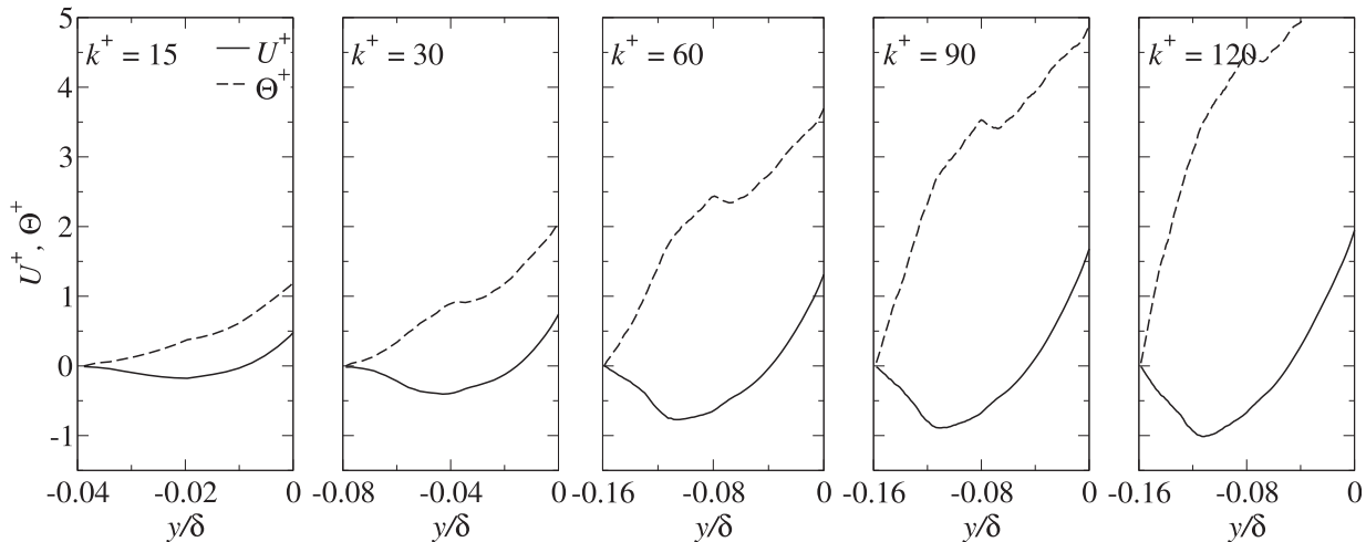
Fig. 13. Velocity and temperature profiles well within the roughness sublayer.
