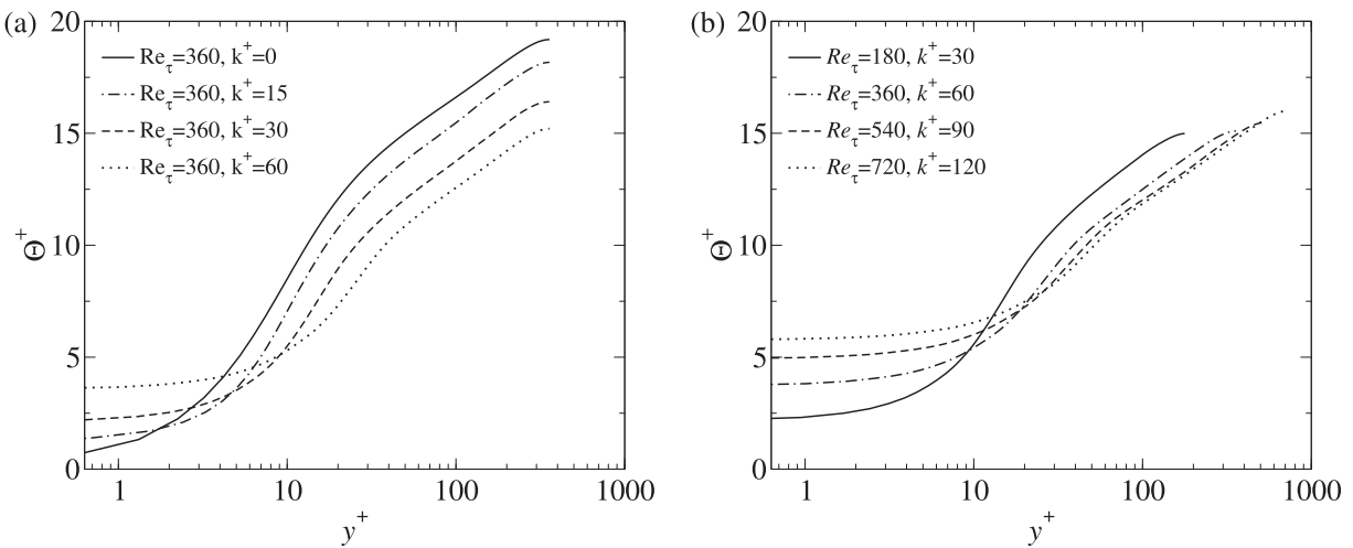
Fig. 5. (a) Mean temperature profiles for Re_{\tau} = 360 . (b) Mean temperature profiles for k/\delta = 1/6 .
