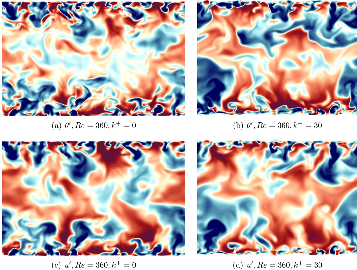
Fig. 11. Instantaneous scalar and streamwise velocity fluctuation fields in the y-z -plane in a smooth channel and a channel with wall roughness.
