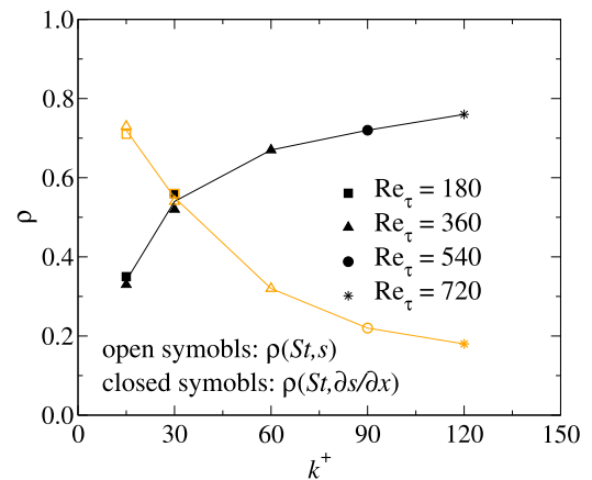
Fig. 17. Correlation coefficients \rho(s, St) and \rho(St, \partial s/\partial x, St) .
