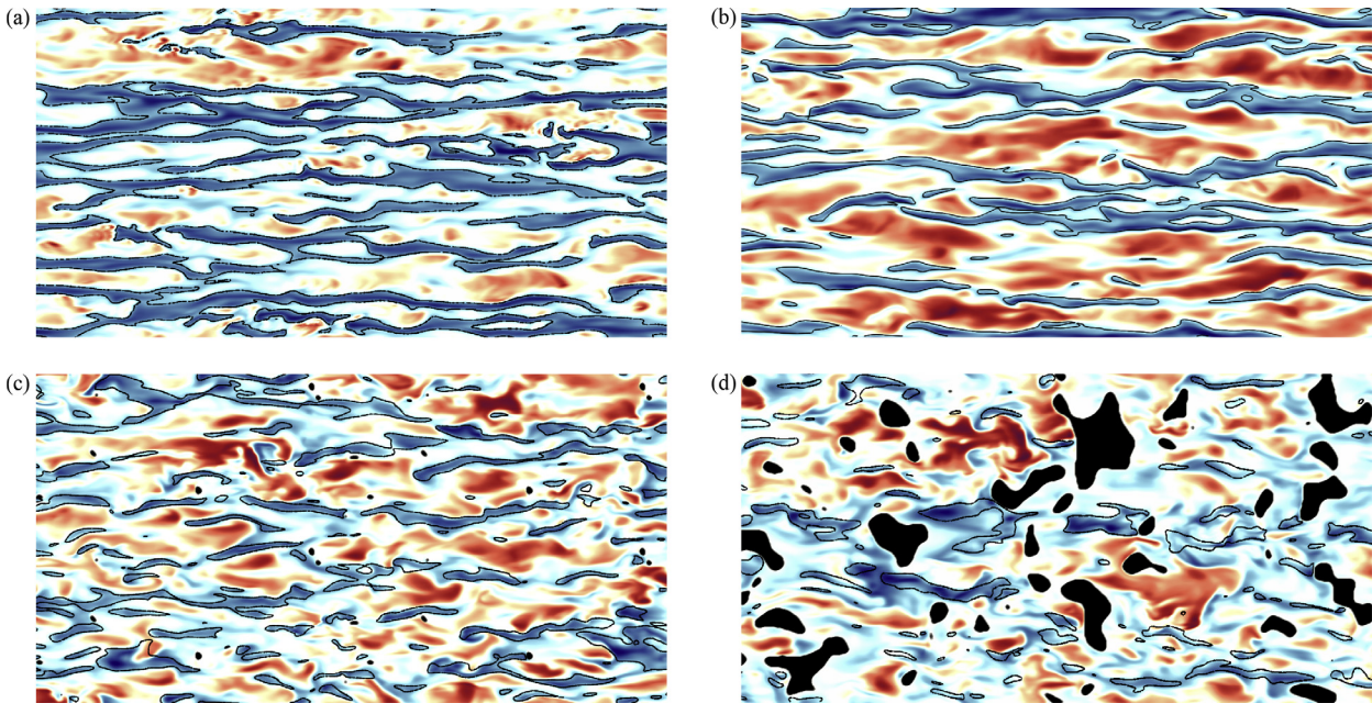
Fig. 10. Temperature streaks at y^+ = 15 , in the Re_\tau = 360, k^+ = 0 (a), Re_\tau = 360, k^+ = 15 (b), Re_\tau = 360, k^+ = 30 (c) and Re_\tau = 360, k^+ = 60 (d) cases. Blue regions correspond to \theta' < 0 , while red regions correspond to \theta' > 0 regions. Black lines enclose regions where u' < 0 . Solid black areas are surface protrusions. (For interpretation of the references to colour in this figure legend, the reader is referred to the web version of this article.)
