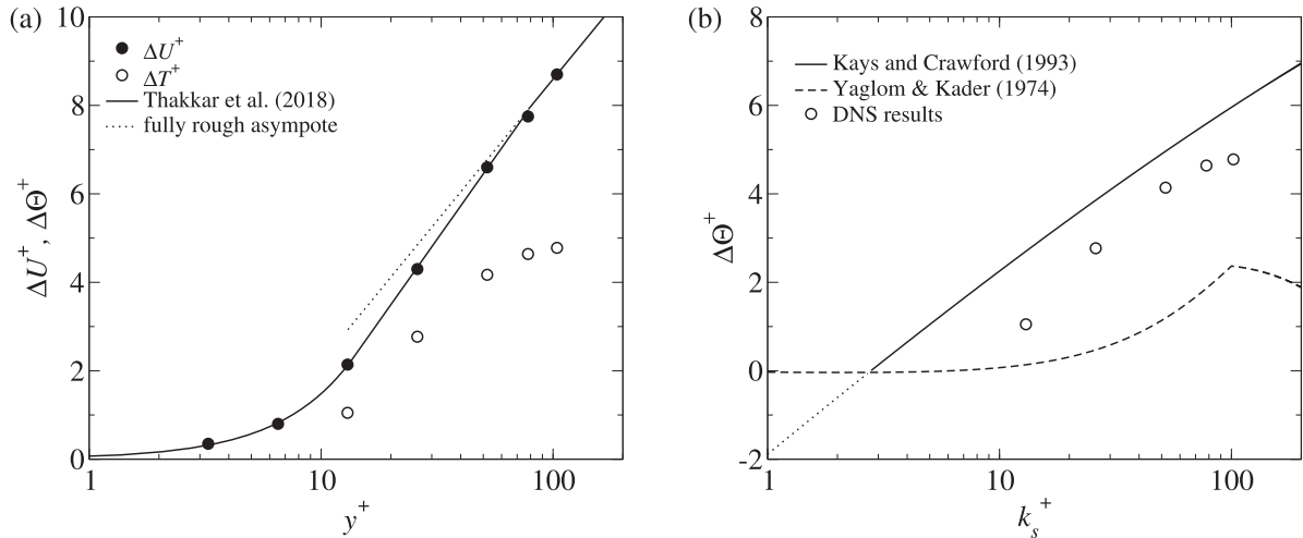
Fig. 18. (a) Wall roughness function for momentum \Delta U^+ and for temperature \Delta \Theta^+ . (b) The temperature roughness function (DNS results) along with estimates obtained from Kays and Crawford [18] and Yaglom and Kader [39].
