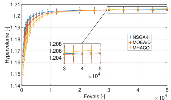
Fig. 4. Hypervolume evolution of MOEA/D, NSGA-II and MHACO on the JUICE bi-objective problem.
