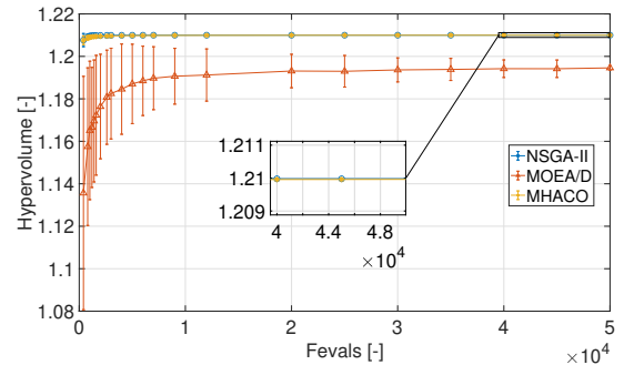
Fig. 3. Average hypervolume evolution of MOEA/D, NSGA-II and MHACO on the Earth-Mars bi-objective transfer problem.
