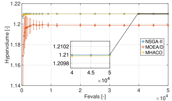
Fig. 2. Average hypervolume evolution of MOEA/D, NSGA-II and MHACO on the Earth-Venus bi-objective transfer problem.
