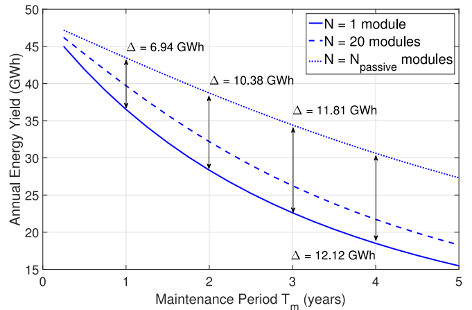
Fig. 19. Annual energy yield with extreme modularity.
