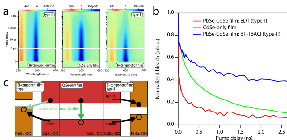
Figure 4. Transient absorption (TA) measurements of electron dynamics upon direct CdSe excitation. (a) TA color maps of a TBACI/BT heterojunction film (left), a CdSe-only film treated with TBACI (middle), and an EDT heterojunction film (right) excited at 570 nm, above the onset of CdSe absorption. The minimum of each color scale is set to the lowest differential absorbance value. The TBACI/BT film shows the longest bleach lifetime, while the bleach of the EDT film is the shortest-lived. (b) Normalized bleach amplitude for the TA measurements displayed in (a), quantitatively showing the difference in bleach decay between the films. (c) Proposed model for the dynamics of bleach decay upon direct CdSe excitation. The increased bleach lifetime in the TBACI/BT film is attributed to spatial separation between electrons and holes across the type-II heterojunction. In the type-I EDT-treated film, instead, electron transfer contributes to the depopulation of the CdSe band edges, increasing the rate of bleach decay.
