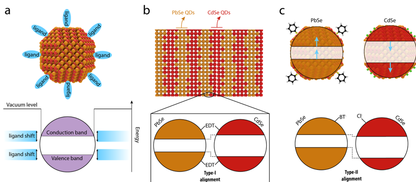
Figure 1. Schematics of QD heterojunction films. (a) Band edges of a semiconductor QD can be shifted by the presence of passivating ligands with different dipole moments. 15,32,33 (b) Structure of a PbSe–CdSe heterojunction QD film, fabricated by dip-coating alternating layers of PbSe and CdSe QDs, and ligand-exchanging the original ligands of the as-synthesized QDs for shorter linker molecules. The inset shows the heterojunction formed by CdSe and PbSe QDs treated with ethanedithiol (EDT), characterized by a type-I band alignment. 34,35 (c) Energy shift induced by the benzenethiol (BT, top left) and tetrabutylammonium chloride (TBACl, top right) ligand treatment on the conduction- and valence-band-edge positions in an EDT-capped QD, as reported by Brown et al., 32 together with the possible type-II heterojunction resulting from BT treatment of PbSe QDs and TBACl treatment of CdSe QDs.
