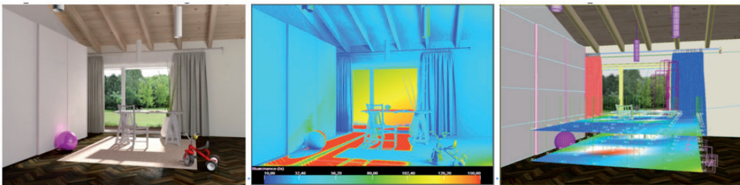
Figure 1 The leftmost image shows a scene, the middle image is a false colour representation of the illuminance over all surfaces of a scene, the right image is a false colour representation of the illuminance over planar cross-sections in the space (available in colour in online version)
