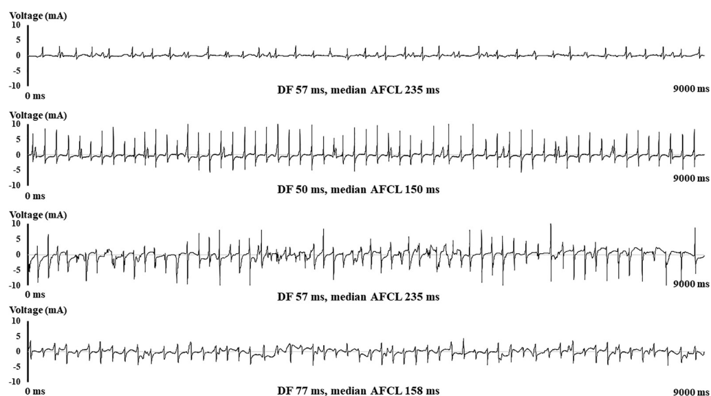
FIGURE 6 Electrograms at DF_{max} Domains
