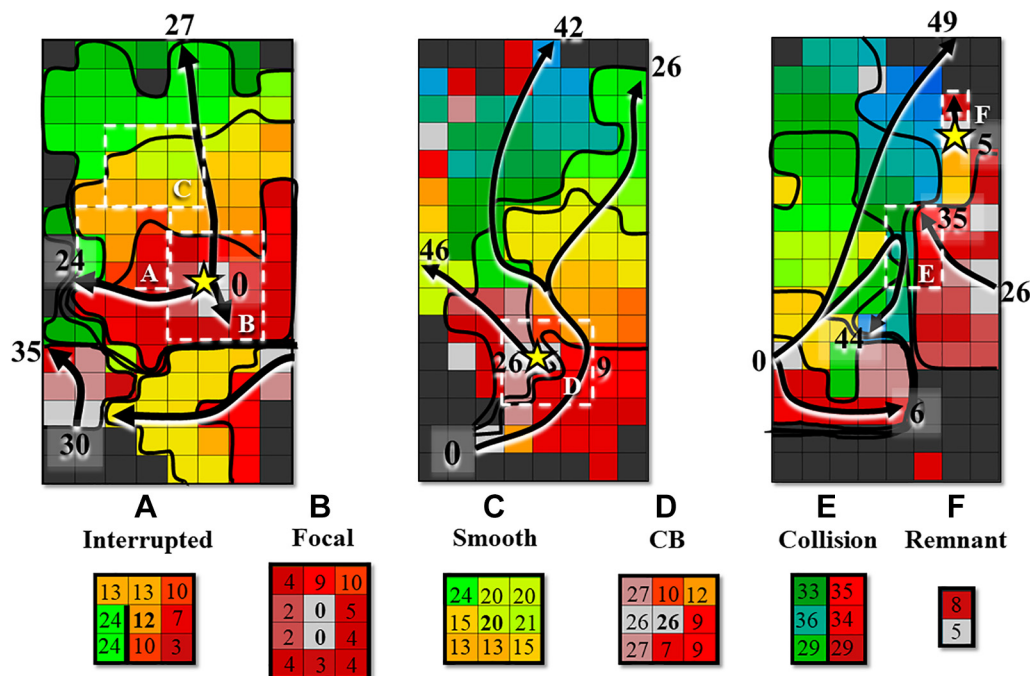
FIGURE 1 Classification of Fibrillation Waves
