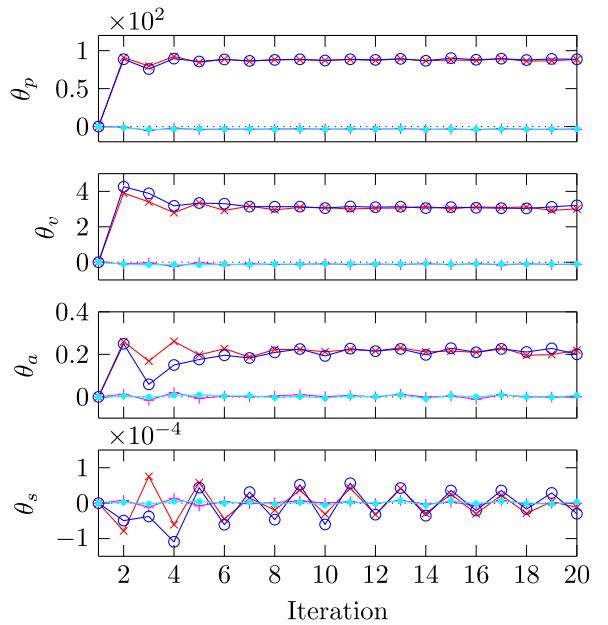
Fig. 22. Tuning parameters learned through iterations in experiment with interaction compensation. \theta_{.11} (—) and \theta_{.21} (—) are using the multirate zero-order-hold differentiator. \theta_{.11} (—) and \theta_{.21} (—) are using the multirate zero-order-hold differentiator. Other tuning parameters are \theta_{.12} = \theta_{.22} = 0 because the reference of the rotation R_z is set to 0 rad for all time.
