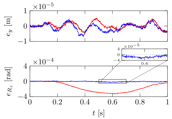
Fig. 14. Tracking error e(t) in experiment using the multirate zero-order-hold differentiator: without (—) and with (—) interaction compensation. Rotation error e_{R_z} is improved about factor 10.
