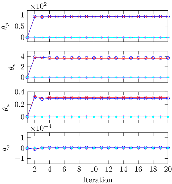
Fig. 19. Tuning parameters learned through iterations in simulation with interaction compensation. \theta_{.11} (—) and \theta_{.21} (—) are using the multirate zero-order-hold differentiator. \theta_{.11} (—) and \theta_{.21} (—) are using the multirate zero-order-hold differentiator. Other tuning parameters are \theta_{.12} = \theta_{.22} = 0 because the reference of the rotation R_z is set to 0 rad for all time.
