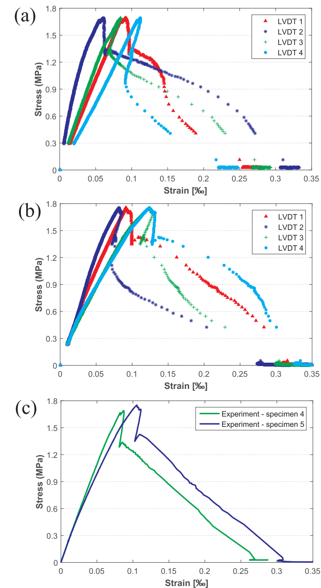
Fig. 4. Experimental stress-strain responses of single notched cement paste pipes (Fig. 1b) subjected to uniaxial tensile loading along vertical direction. (a) Specimen 4, (b) specimen 5 and (c) comparison between specimen 4 and specimen 5 (strain is the average value of the four LVDTs).
