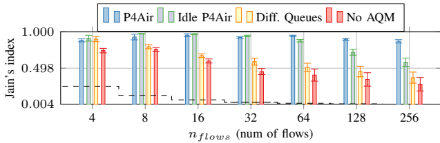
(f) Average Inter- and intra- fairness. The share of flows per group was varied between 0% and 100% with a step of 25% (as in Fig. 7e). All flows had the same RTT. For each n_{flows} , each combination (35 different) is run 4 times (140 in total). Theoretical minimum is shown as a dashed black line.
