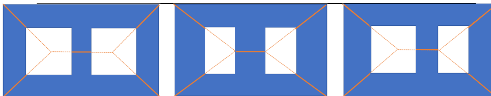
Figure 10. Failure mechanisms for double window configurations 1 to 3. Cracks are indicated by the solid orange lines.
