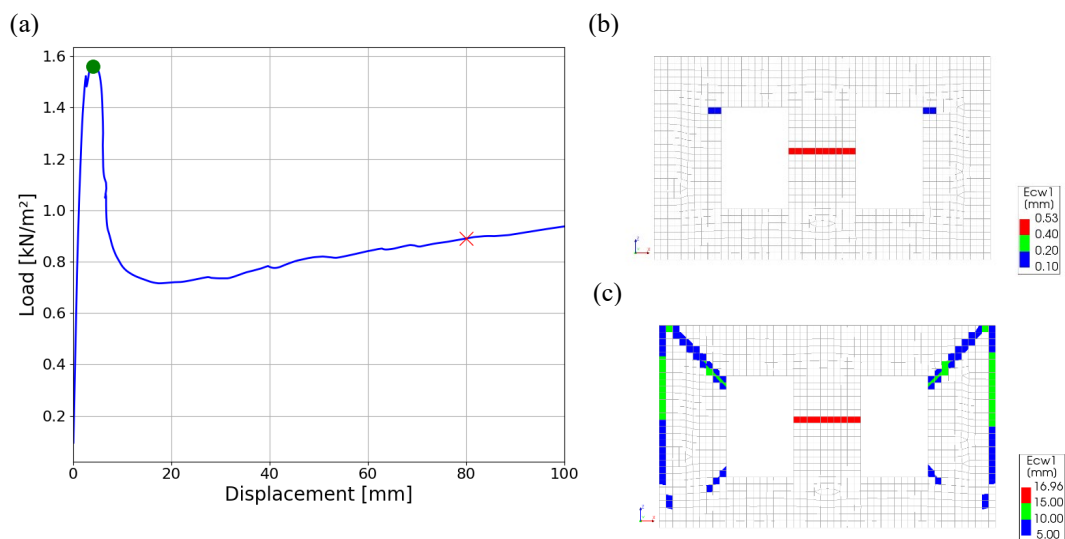
Figure 5. Crack patterns configuration 2: wall with two windows of 1.0 \times 1.5 \text{ m}^2 at (b) ultimate load capacity ((a) green marker) and at (c) a maximum out-of-plane wall displacement of 80 mm ((a) red marker).
