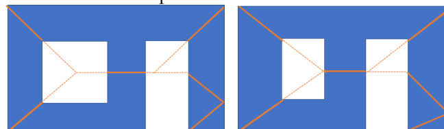
Figure 11. Failure mechanism for window-door configurations 1 and 2. Cracks are indicated by the solid orange lines.
