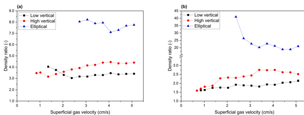
Fig. 11. Density ratios between top and bottom sections of vibro-fluidized beds consisting of nano-powder with (a) low and (b) high initial bed heights.
