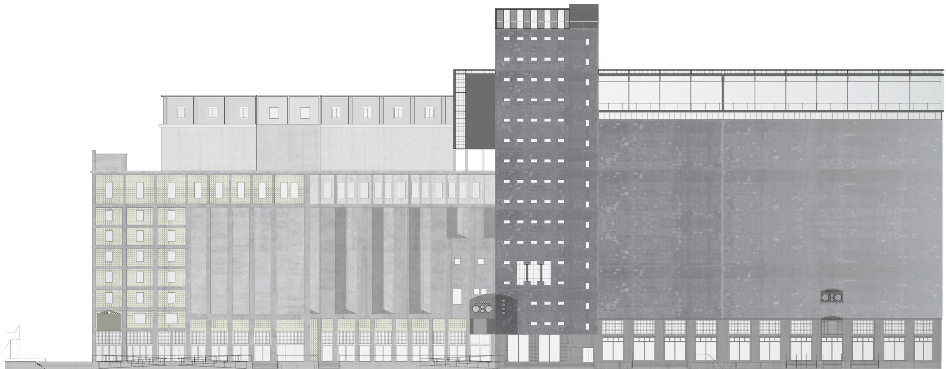
North Facade - scale 1:350
