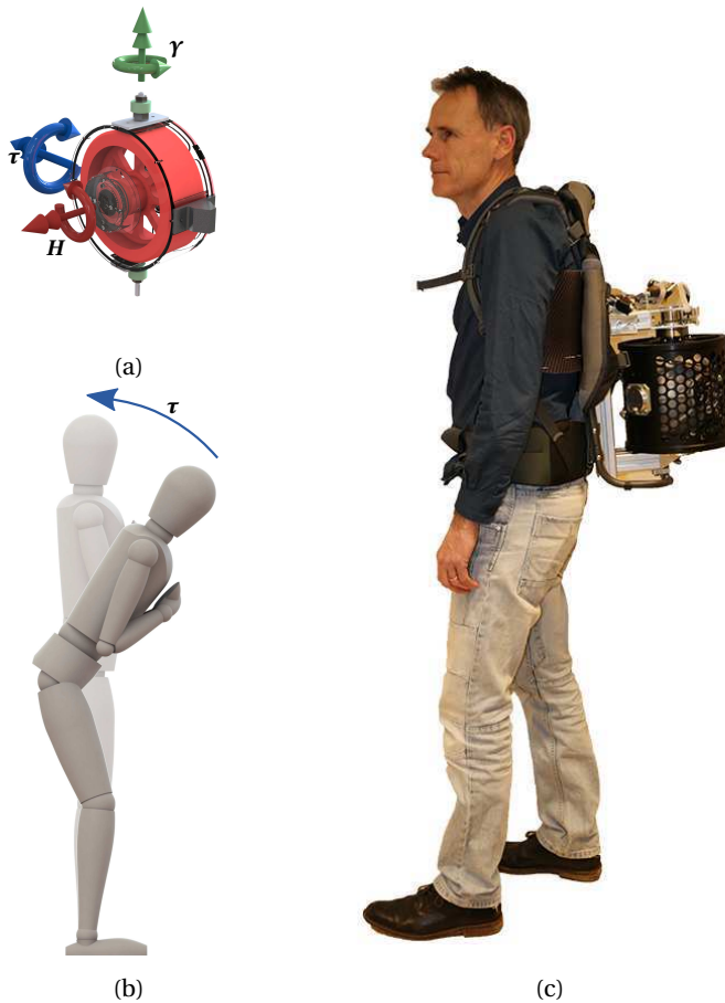
Figure 4.1: GyBAR prototype wearable gyroscopic actuator. (a): Assistive torque, \tau , is proportional to the angular momentum, H , of a spinning mass and the rate at which it is gimbaled, \gamma , in a motorized frame. (b): Example use of a torque to restore upright posture. (c): Subject wearing the new version of the GyBAR.
