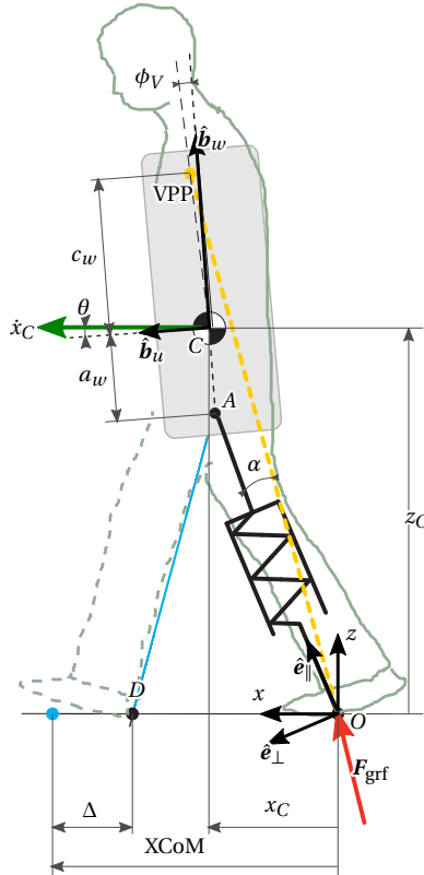
Figure 2.1: Geometrical representation of Virtual Pendulum Model with Virtual Pivot Point (VPP) control for the upper body (with ground reaction force F_{grf} ) and foot placement with the extrapolated center of mass (XCoM, calculated with i.a. the velocity, v , of the center of mass)
