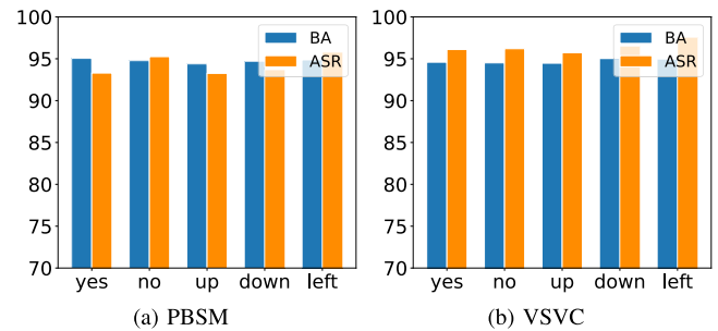
Fig. 6. The effects of the target label on our PBSM and VSVC attacks on the SCD-10 dataset.
