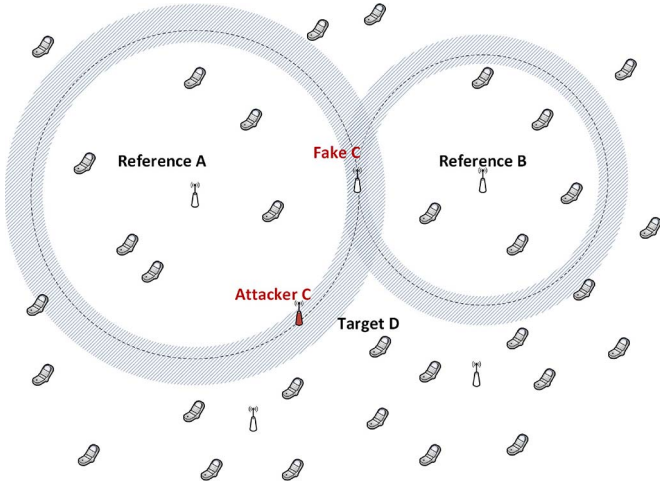
Fig. 10. Attacker C reports its fake location at fake\ C . Both reference nodes, such as reference\ A and reference\ B , and the target node target\ D can self-estimate the PLE. Based on the self-estimated PLE and the location information, the shaded area can be constructed as the trust region for detecting an attacker, outside of which attacker\ C will be detected.
